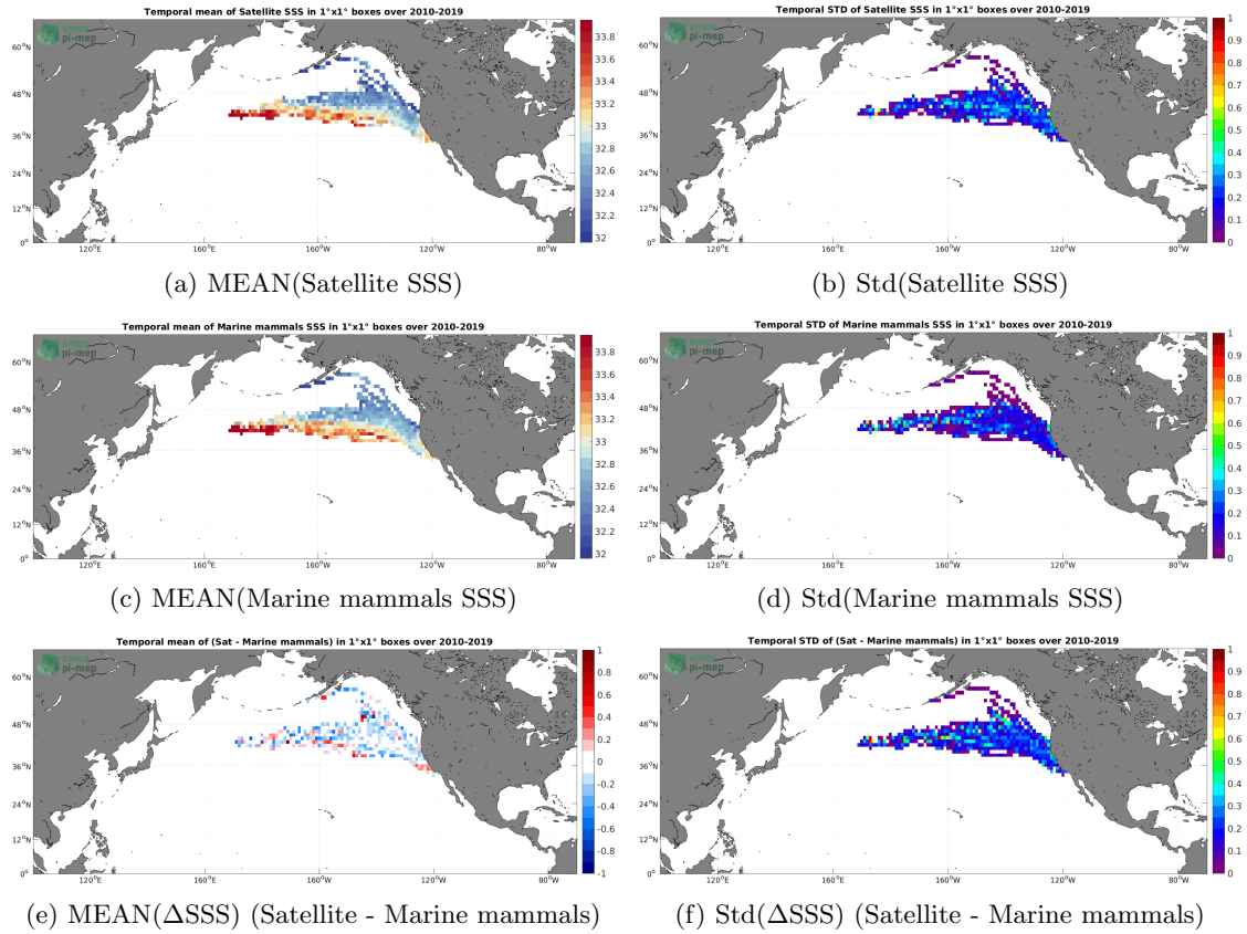
Figure 6: Temporal mean (left) and Std (right) of SSS from SMOS SSS L3 v8 - 9 Days (CATDS-CECOS-LOCEAN) (top), Marine mammals (middle), and of \Delta SSS (Satellite - Marine mammals). Only match-up pairs are used to generate these maps.
