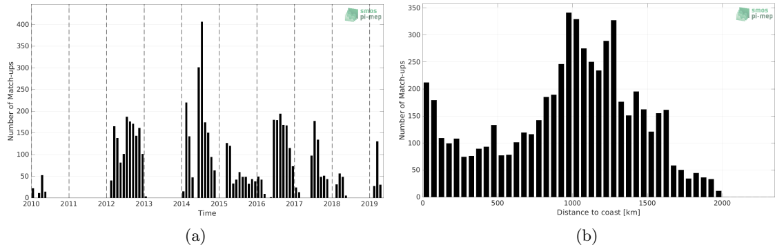
Figure 1: Number of match-ups between Marine mammals and SMOS SSS L3 v8 - 9 Days (CATDS-CECOS-LOCEAN) SSS as a function of time (a) and as function of the distance to coast (b) over the North Pacific Ocean Pi-MEP region and for the full satellite product period.
