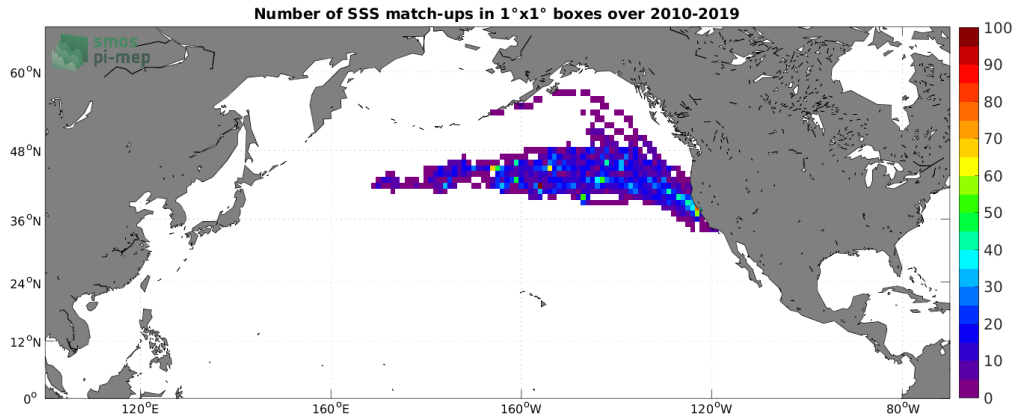
Figure 4: Number of SSS match-ups between Marine mammals SSS and the SMOS SSS L3 v8 - 9 Days (CATDS-CECOS-LOCEAN) SSS product for the North Pacific Ocean Pi-MEP region over 1^\circ \times 1^\circ boxes and for the full satellite product period.
