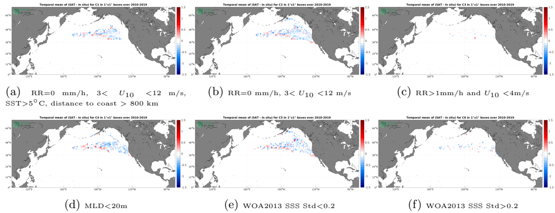
Figure 12: Temporal mean gridded over spatial boxes of size 1^{\circ}\times 1^{\circ} of \Delta\text{SSS} (SMOS SSS L3 v8 - 9 Days (CATDS-CECOS-LOCEAN) - Marine mammals) for 6 different subdatasets corresponding to:RR=0 mm/h, 3 < U_{10} < 12 m/s, SST > 5^{\circ}\text{C} , distance to coast > 800 km (a), RR=0 mm/h, 3 < U_{10} < 12 m/s (b), RR > 1 mm/h and U_{10} < 4 m/s (c),MLD < 20\text{m} (d),WOA2013 SSS Std < 0.2 (e),WOA2013 SSS Std > 0.2 (f).
