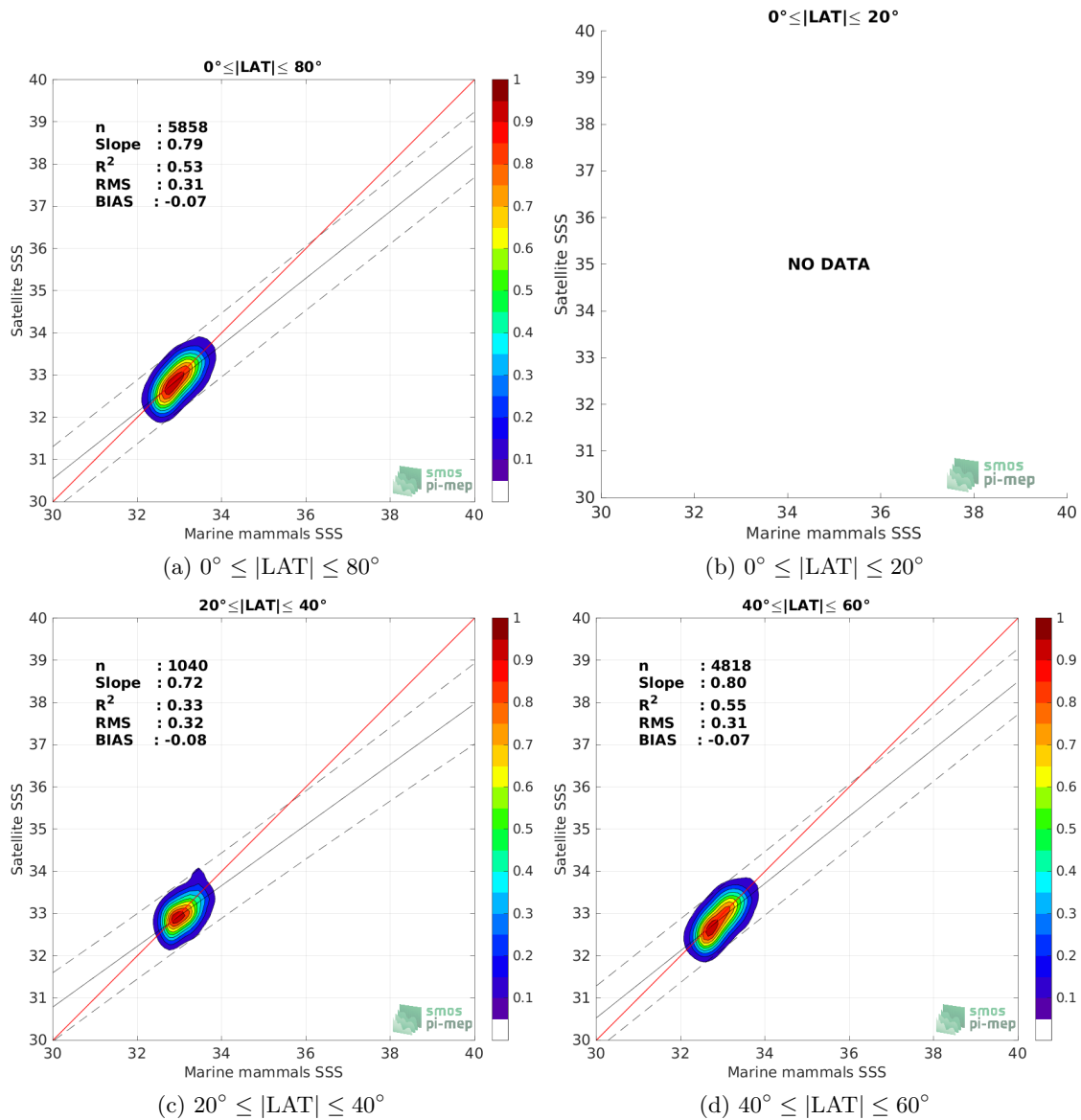
Figure 9: Contour maps of the concentration of SMOS SSS L3 v8 - 9 Days (CATDS-CECOS-LOCEAN) SSS ( y -axis) versus Marine mammals SSS ( x -axis) at match-up pairs for different latitude bands. For each plot, the red line shows x=y . The black thin and dashed lines indicate a linear fit through the data cloud and the \pm 95\% confidence levels, respectively. The number match-up pairs n , the slope and R^2 coefficient of the linear fit, the root mean square (RMS) and the mean bias between satellite and in situ data are indicated for each latitude band in each plots.
