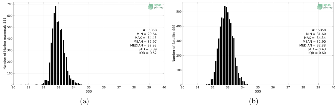
Figure 2: Histograms of SSS from Marine mammals (a) and SMOS SSS L3 v8 - 9 Days (CATDS-CECOS-LOCEAN) (b) considering all match-up pairs per bins of 0.1 over the North Pacific Ocean Pi-MEP region and for the full satellite product period.
