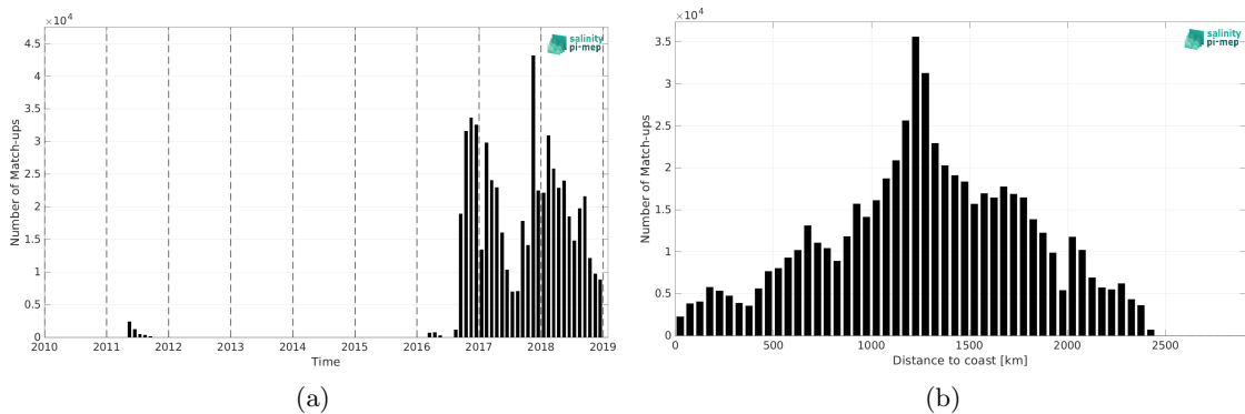
Figure 1: Number of match-ups between Surface drifters and SMOS SSS L3 v8 - 9 Days (CATDS-CEC-LOCEAN) SSS as a function of time (a) and as function of the distance to coast (b) over the North Pacific Ocean Pi-MEP region and for the full satellite product period.
