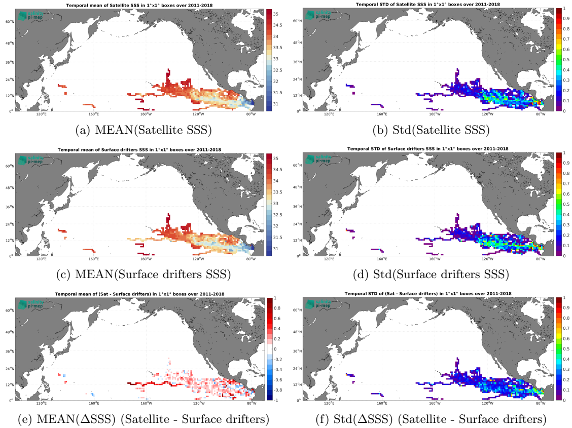
Figure 5: Temporal mean (left) and Std (right) of SSS from SMOS SSS L3 v8 - 9 Days (CATDS-CEC-LOCEAN) (top), Surface drifters (middle), and of \Delta SSS (Satellite - Surface drifters). Only match-up pairs are used to generate these maps.
