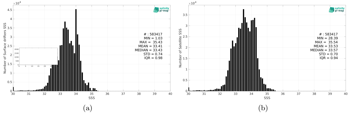
Figure 2: Histograms of SSS from Surface drifters (a) and SMOS SSS L3 v8 - 9 Days (CATDS-CEC-LOCEAN) (b) considering all match-up pairs per bins of 0.1 over the North Pacific Ocean Pi-MEP region and for the full satellite product period.
