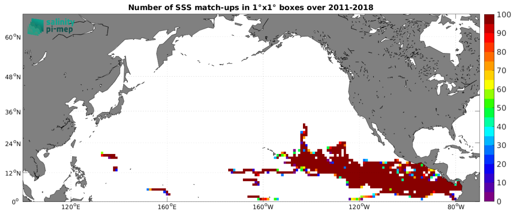
Figure 3: Number of SSS match-ups between Surface drifters SSS and the SMOS SSS L3 v8 - 9 Days (CATDS-CEC-LOCEAN) SSS product for the North Pacific Ocean Pi-MEP region over 1^\circ \times 1^\circ boxes and for the full satellite product period.
