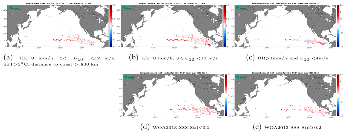
Figure 11: Temporal mean gridded over spatial boxes of size 1^\circ \times 1^\circ of \Delta SSS (SMOS SSS L3 v8 - 9 Days (CATDS-CEC-LOCEAN) - Surface drifters) for 5 different subdatasets corresponding to:RR=0 mm/h, 3 < U_{10} < 12 m/s, SST >5^\circ C, distance to coast > 800 km (a), RR=0 mm/h, 3 < U_{10} < 12 m/s (b), RR >1 mm/h and U_{10} < 4 m/s (c), WOA2013 SSS Std <0.2 (d), WOA2013 SSS Std >0.2 (e).
