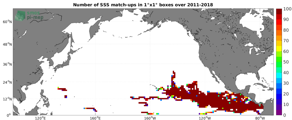
Figure 3: Number of SSS match-ups between Surface drifters SSS and the SMOS SSS L3 v8 - 9 Days (CATDS-CECOS-LOCEAN) SSS product for the North Pacific Ocean Pi-MEP region over 1^\circ \times 1^\circ boxes and for the full satellite product period.
