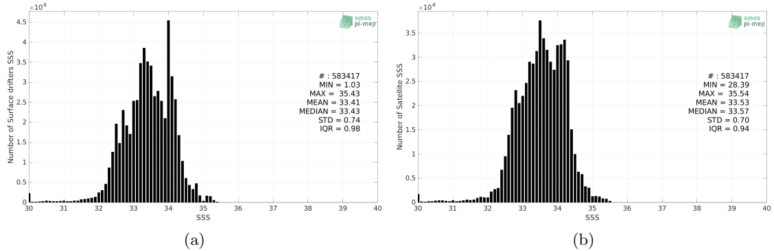
Figure 2: Histograms of SSS from Surface drifters (a) and SMOS SSS L3 v8 - 9 Days (CATDS-CECOS-LOCEAN) (b) considering all match-up pairs per bins of 0.1 over the North Pacific Ocean Pi-MEP region and for the full satellite product period.
