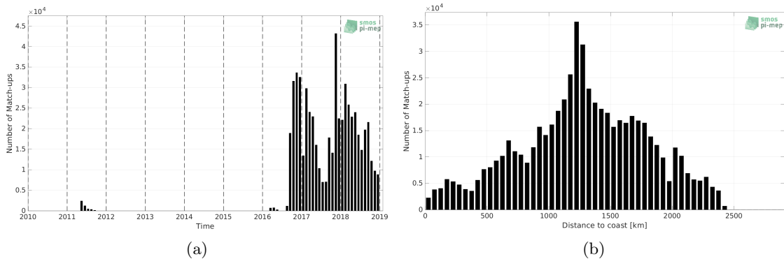
Figure 1: Number of match-ups between Surface drifters and SMOS SSS L3 v8 - 9 Days (CATDS-CECOS-LOCEAN) SSS as a function of time (a) and as function of the distance to coast (b) over the North Pacific Ocean Pi-MEP region and for the full satellite product period.
