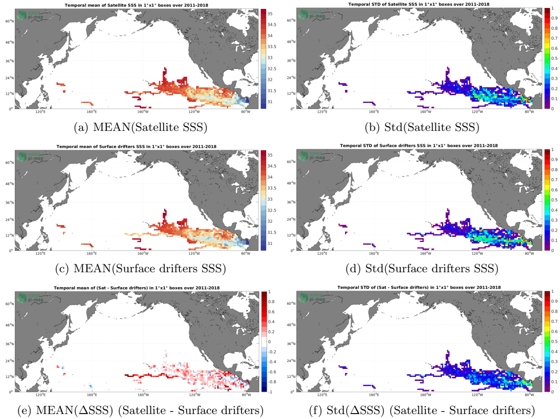
Figure 5: Temporal mean (left) and Std (right) of SSS from SMOS SSS L3 v8 - 9 Days (CATDS-CECOS-LOCEAN) (top), Surface drifters (middle), and of \Delta SSS (Satellite - Surface drifters). Only match-up pairs are used to generate these maps.
