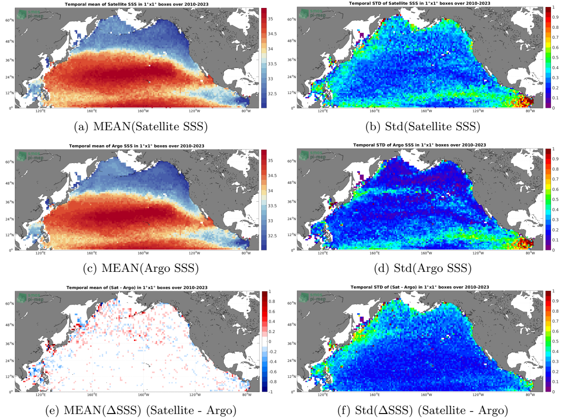
Figure 6: Temporal mean (left) and Std (right) of SSS from SMOS SSS L3 v8 - 9 Days (CATDS-CECOS-LOCEAN) (top), Argo (middle), and of \Delta SSS (Satellite - Argo). Only match-up pairs are used to generate these maps.
