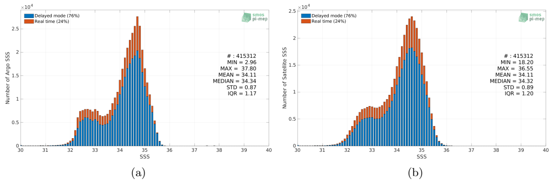
Figure 2: Histograms of SSS from Argo (a) and SMOS SSS L3 v8 - 9 Days (CATDS-CECOS-LOCEAN) (b) considering all match-up pairs per bins of 0.1 over the North Pacific Ocean Pi-MEP region and for the full satellite product period.
