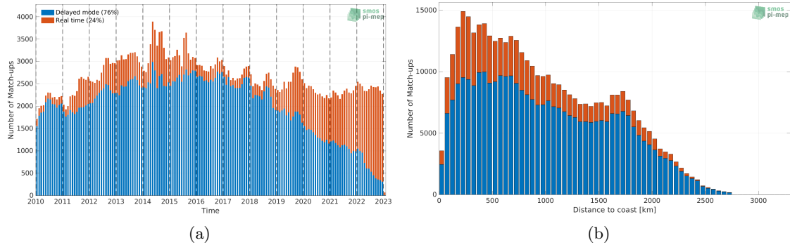
Figure 1: Number of match-ups between Argo and SMOS SSS L3 v8 - 9 Days (CATDS-CECOS-LOCEAN) SSS as a function of time (a) and as function of the distance to coast (b) over the North Pacific Ocean Pi-MEP region and for the full satellite product period.
