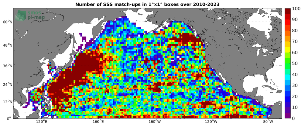
Figure 4: Number of SSS match-ups between Argo SSS and the SMOS SSS L3 v8 - 9 Days (CATDS-CECOS-LOCEAN) SSS product for the North Pacific Ocean Pi-MEP region over 1^\circ \times 1^\circ boxes and for the full satellite product period.
