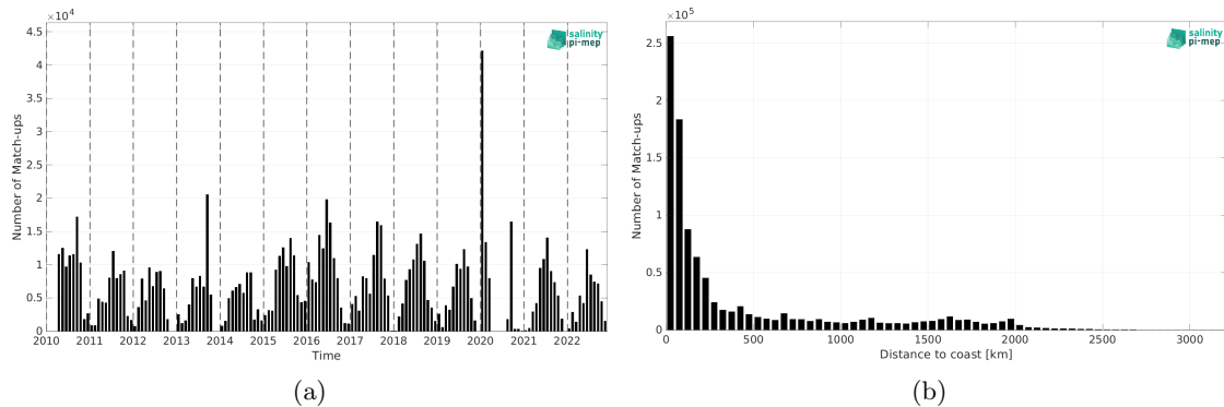
Figure 1: Number of match-ups between TSG (SAMOS) and SMOS SSS L3 v8 - 18 Days (CATDS-CEC-LOCEAN) SSS as a function of time (a) and as function of the distance to coast (b) over the North Pacific Ocean Pi-MEP region and for the full satellite product period.
