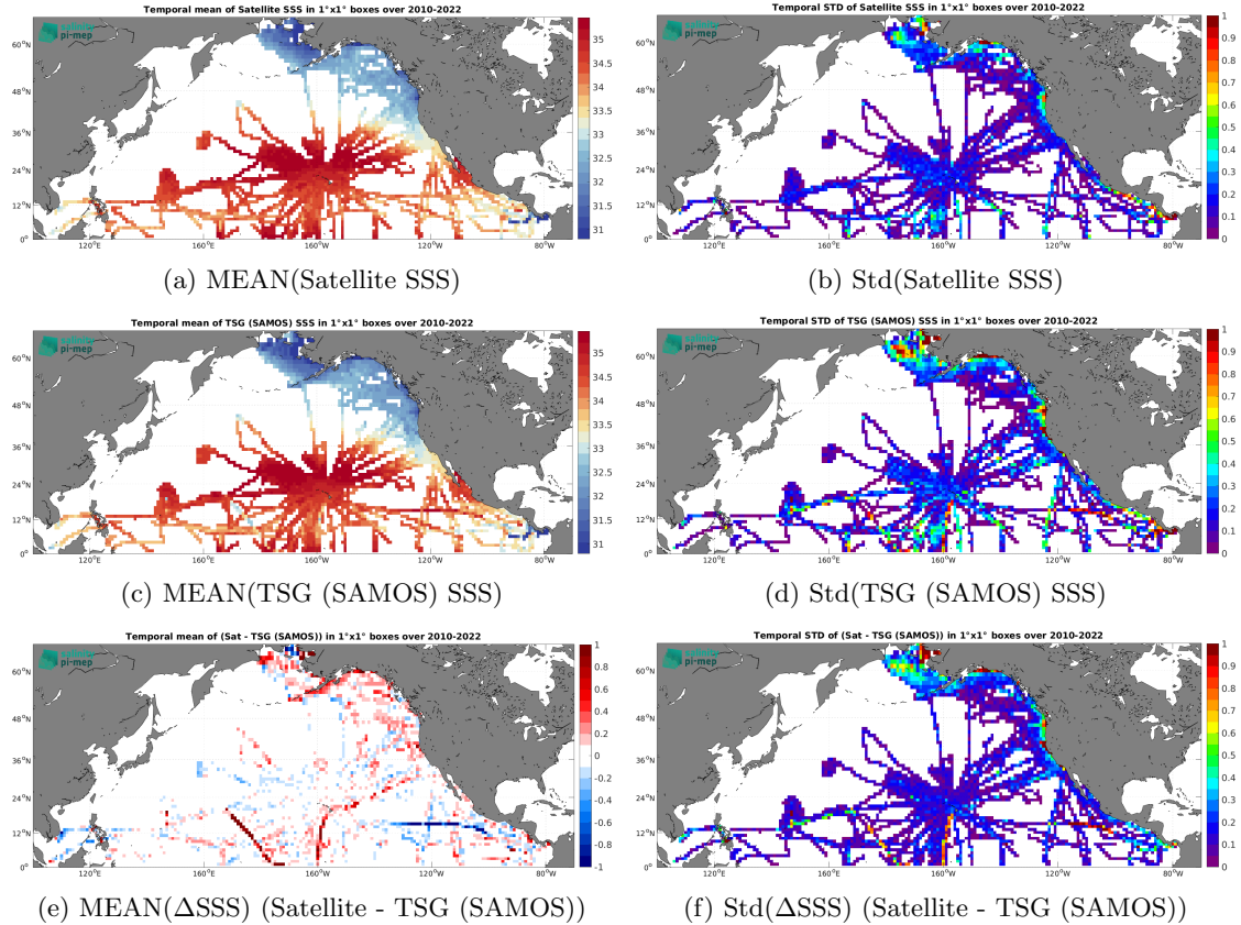
Figure 6: Temporal mean (left) and Std (right) of SSS from SMOS SSS L3 v8 - 18 Days (CATDS-CEC-LOCEAN) (top), TSG (SAMOS) (middle), and of \Delta SSS (Satellite - TSG (SAMOS)). Only match-up pairs are used to generate these maps.
