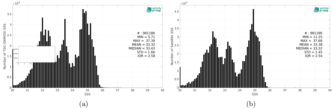
Figure 2: Histograms of SSS from TSG (SAMOS) (a) and SMOS SSS L3 v8 - 18 Days (CATDS-CEC-LOCEAN) (b) considering all match-up pairs per bins of 0.1 over the North Pacific Ocean Pi-MEP region and for the full satellite product period.
