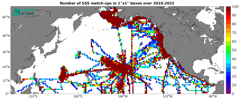
Figure 4: Number of SSS match-ups between TSG (SAMOS) SSS and the SMOS SSS L3 v8 - 18 Days (CATDS-CEC-LOCEAN) SSS product for the North Pacific Ocean Pi-MEP region over 1^\circ \times 1^\circ boxes and for the full satellite product period.
