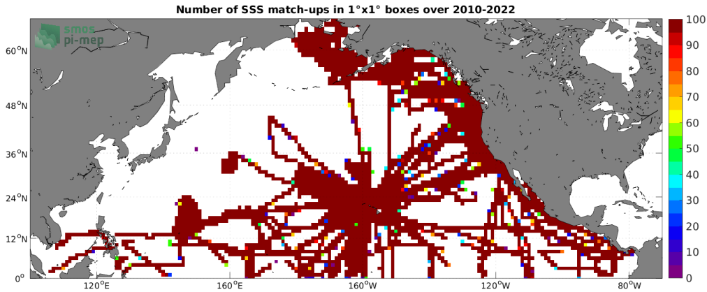
Figure 4: Number of SSS match-ups between TSG (SAMOS) SSS and the SMOS SSS L3 v8 - 18 Days (CATDS-CECOS-LOCEAN) SSS product for the North Pacific Ocean Pi-MEP region over 1^\circ \times 1^\circ boxes and for the full satellite product period.
