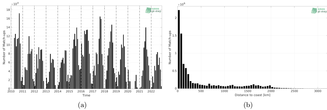
Figure 1: Number of match-ups between TSG (SAMOS) and SMOS SSS L3 v8 - 18 Days (CATDS-CECOS-LOCEAN) SSS as a function of time (a) and as function of the distance to coast (b) over the North Pacific Ocean Pi-MEP region and for the full satellite product period.
