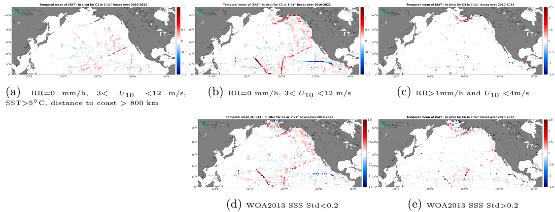
Figure 12: Temporal mean gridded over spatial boxes of size 1^\circ \times 1^\circ of \Delta SSS (SMOS SSS L3 v8 - 18 Days (CATDS-CECOS-LOCEAN) - TSG (SAMOS)) for 5 different subdatasets corresponding to:RR=0 mm/h, 3 < U_{10} < 12 m/s, SST >5^\circ C, distance to coast > 800 km (a), RR=0 mm/h, 3 < U_{10} < 12 m/s (b), RR >1 mm/h and U_{10} < 4 m/s (c), WOA2013 SSS Std <0.2 (d), WOA2013 SSS Std >0.2 (e).
