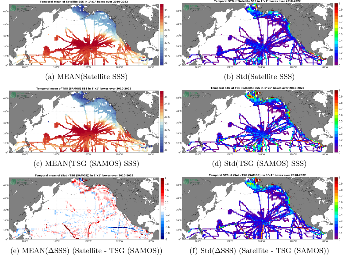
Figure 6: Temporal mean (left) and Std (right) of SSS from SMOS SSS L3 v8 - 18 Days (CATDS-CECOS-LOCEAN) (top), TSG (SAMOS) (middle), and of \Delta SSS (Satellite - TSG (SAMOS)). Only match-up pairs are used to generate these maps.
