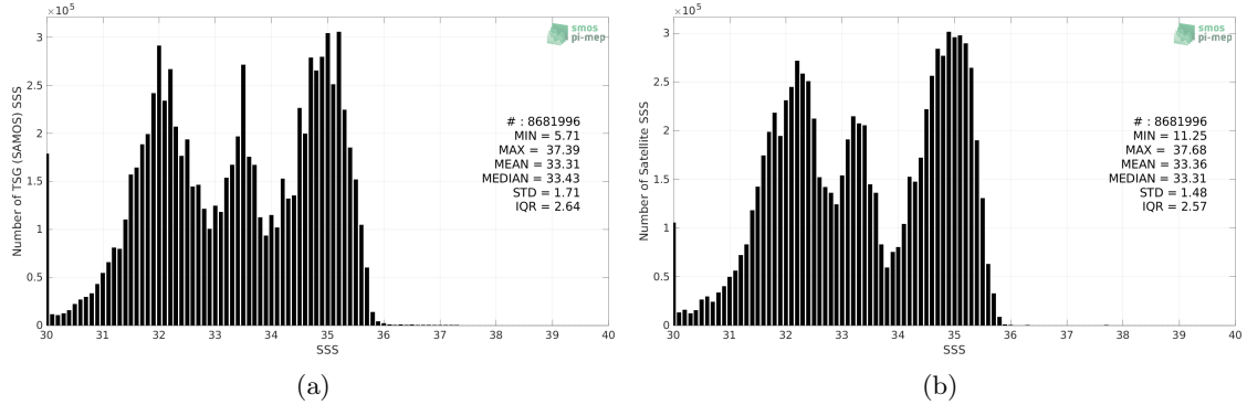
Figure 2: Histograms of SSS from TSG (SAMOS) (a) and SMOS SSS L3 v8 - 18 Days (CATDS-CECOS-LOCEAN) (b) considering all match-up pairs per bins of 0.1 over the North Pacific Ocean Pi-MEP region and for the full satellite product period.
