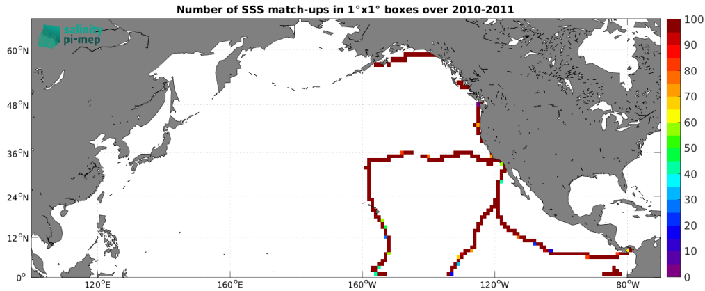
Figure 4: Number of SSS match-ups between TSG (GOSUD-Sailing-ship) SSS and the SMOS SSS L3 v8 - 18 Days (CATDS-CEC-LOCEAN) SSS product for the North Pacific Ocean Pi-MEP region over 1^\circ \times 1^\circ boxes and for the full satellite product period.
