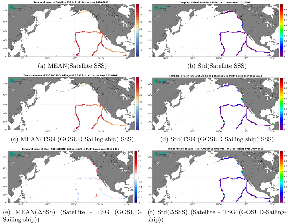
Figure 6: Temporal mean (left) and Std (right) of SSS from SMOS SSS L3 v8 - 18 Days (CATDS-CEC-LOCEAN) (top), TSG (GOSUD-Sailing-ship) (middle), and of \Delta SSS (Satellite - TSG (GOSUD-Sailing-ship)). Only match-up pairs are used to generate these maps.
