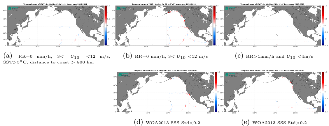
Figure 12: Temporal mean gridded over spatial boxes of size 1^\circ \times 1^\circ of \Delta SSS (SMOS SSS L3 v8 - 18 Days (CATDS-CEC-LOCEAN) - TSG (GOSUD-Sailing-ship)) for 5 different subdatasets corresponding to:RR=0 mm/h, 3 < U_{10} < 12 m/s, SST >5^\circ\text{C} , distance to coast > 800 km (a), RR=0 mm/h, 3 < U_{10} < 12 m/s (b), RR >1 mm/h and U_{10} < 4 m/s (c), WOA2013 SSS Std <0.2 (d), WOA2013 SSS Std >0.2 (e).
