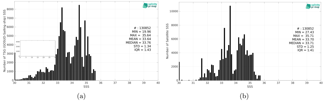
Figure 2: Histograms of SSS from TSG (GOSUD-Sailing-ship) (a) and SMOS SSS L3 v8 - 18 Days (CATDS-CEC-LOCEAN) (b) considering all match-up pairs per bins of 0.1 over the North Pacific Ocean Pi-MEP region and for the full satellite product period.
