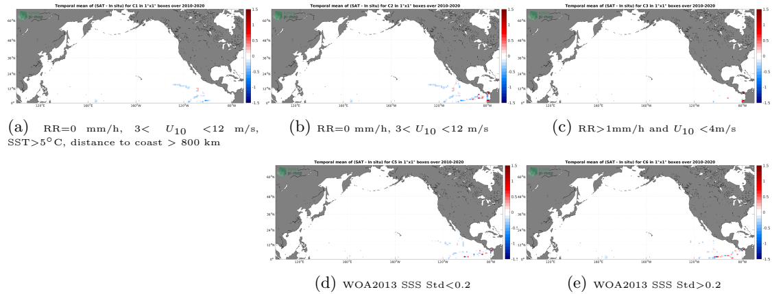
Figure 12: Temporal mean gridded over spatial boxes of size 1^{\circ}\times 1^{\circ} of \Delta SSS (SMOS SSS L3 v8 - 18 Days (CATDS-CECOS-LOCEAN) - TSG (GOSUD-Research-vessel)) for 5 different sub-datasets corresponding to:RR=0 mm/h, 3 < U_{10} < 12 m/s, SST >5^{\circ}\text{C} , distance to coast > 800 km (a), RR=0 mm/h, 3 < U_{10} < 12 m/s (b), RR >1 mm/h and U_{10} < 4 m/s (c), WOA2013 SSS Std <0.2 (d), WOA2013 SSS Std >0.2 (e).
