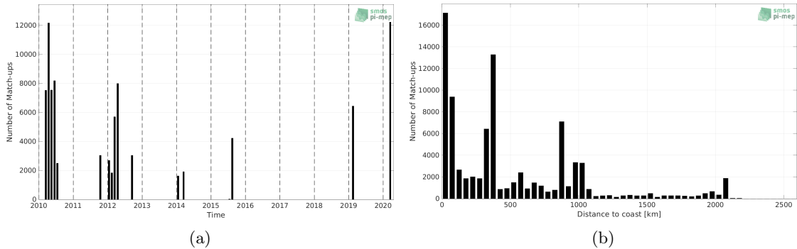
Figure 1: Number of match-ups between TSG (GOSUD-Research-vessel) and SMOS SSS L3 v8 - 18 Days (CATDS-CECOS-LOCEAN) SSS as a function of time (a) and as function of the distance to coast (b) over the North Pacific Ocean Pi-MEP region and for the full satellite product period.
