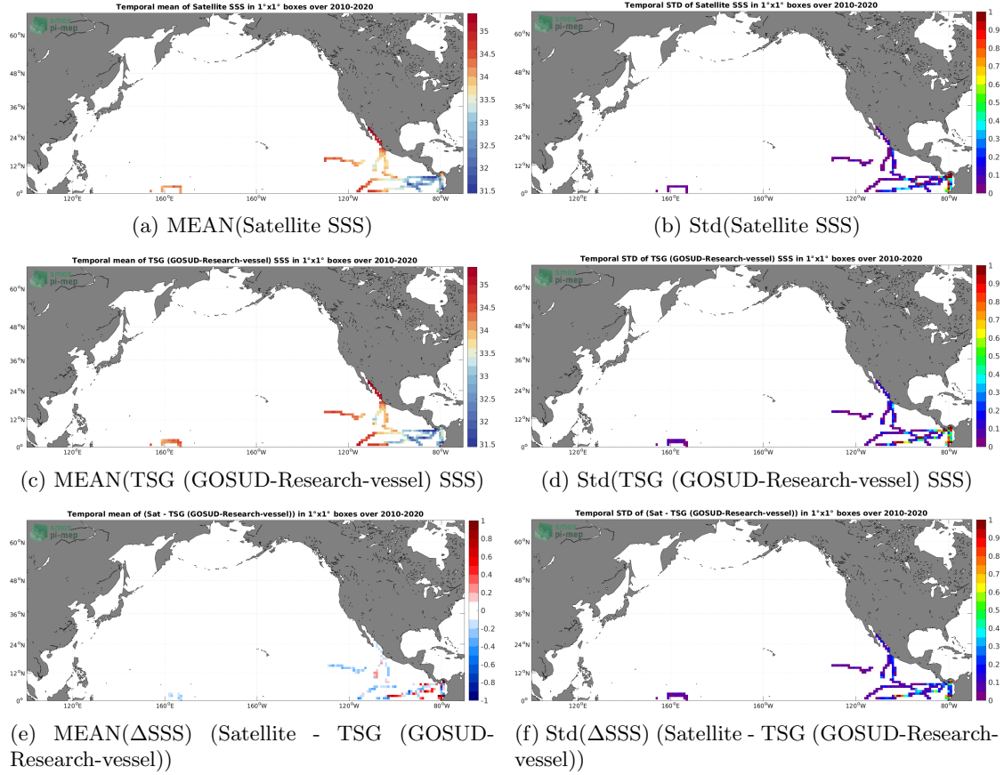
Figure 6: Temporal mean (left) and Std (right) of SSS from SMOS SSS L3 v8 - 18 Days (CATDS-CECOS-LOCEAN) (top), TSG (GOSUD-Research-vessel) (middle), and of \Delta SSS (Satellite - TSG (GOSUD-Research-vessel)). Only match-up pairs are used to generate these maps.
