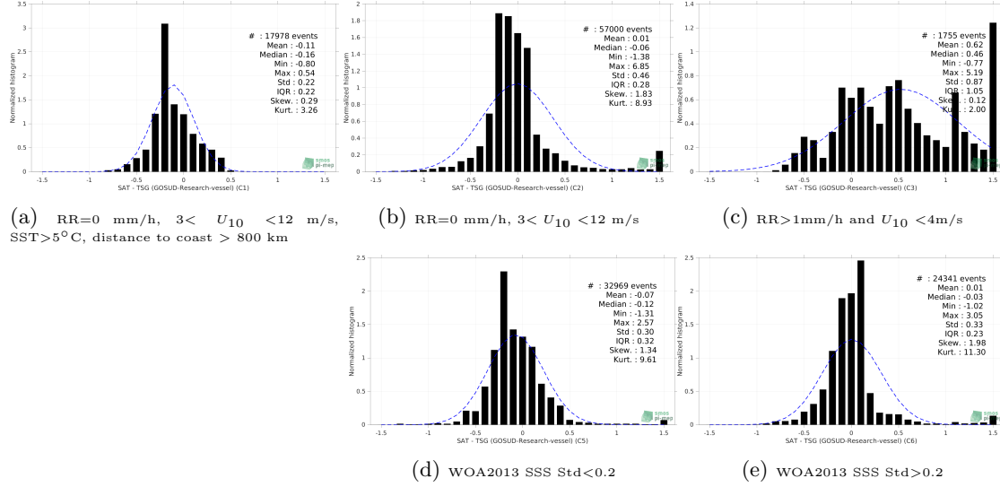
Figure 13: Normalized histogram of \Delta SSS (SMOS SSS L3 v8 - 18 Days (CATDS-CECOS-LOCEAN) - TSG (GOSUD-Research-vessel)) for 5 different subdatasets corresponding to: RR=0 mm/h, 3 < U_{10} < 12 m/s, SST > 5°C, distance to coast > 800 km (a), RR=0 mm/h, 3 < U_{10} < 12 m/s (b), RR > 1mm/h and U_{10} < 4 m/s (c), WOA2013 SSS Std < 0.2 (d), WOA2013 SSS Std > 0.2 (e).
