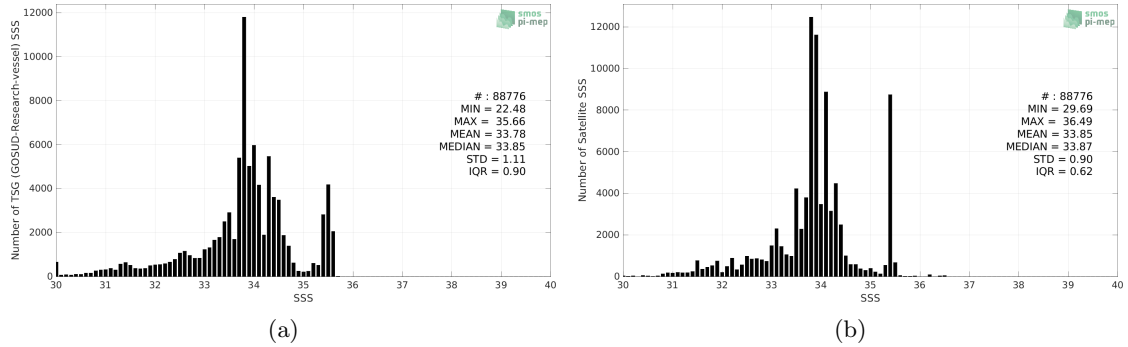
Figure 2: Histograms of SSS from TSG (GOSUD-Research-vessel) (a) and SMOS SSS L3 v8 - 18 Days (CATDS-CECOS-LOCEAN) (b) considering all match-up pairs per bins of 0.1 over the North Pacific Ocean Pi-MEP region and for the full satellite product period.
