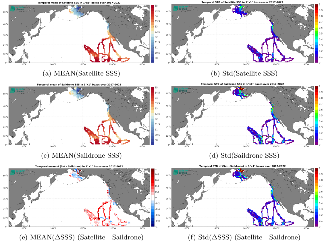
Figure 6: Temporal mean (left) and Std (right) of SSS from SMOS SSS L3 v8 - 18 Days (CATDS-CEC-LOCEAN) (top), Saildrone (middle), and of \Delta\text{SSS} (Satellite - Saildrone). Only match-up pairs are used to generate these maps.
