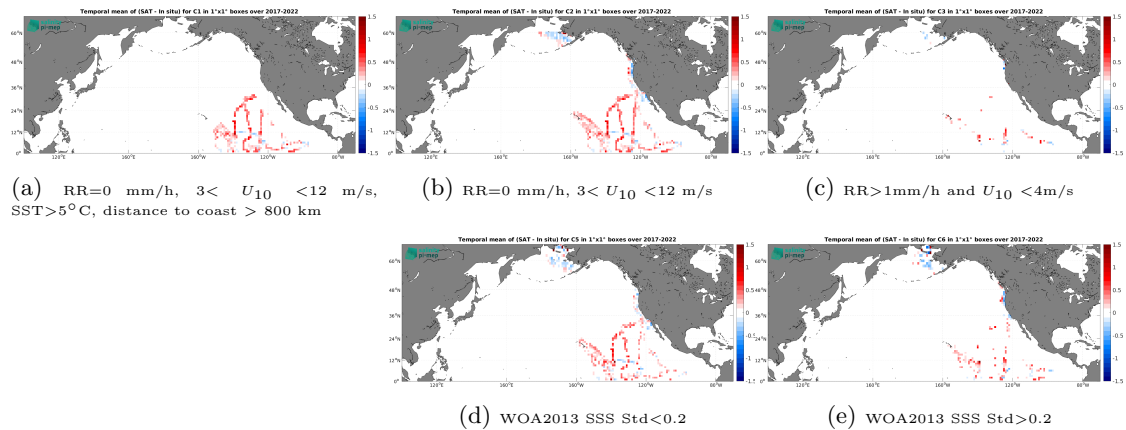
Figure 12: Temporal mean gridded over spatial boxes of size 1^\circ \times 1^\circ of \Delta SSS (SMOS SSS L3 v8 - 18 Days (CATDS-CEC-LOCEAN) - Saildrone) for 5 different subdatasets corresponding to:RR=0 mm/h, 3 < U_{10} < 12 m/s, SST >5^\circ\text{C} , distance to coast > 800 km (a), RR=0 mm/h, 3 < U_{10} < 12 m/s (b), RR >1 mm/h and U_{10} < 4 m/s (c), WOA2013 SSS Std <0.2 (d), WOA2013 SSS Std >0.2 (e).
