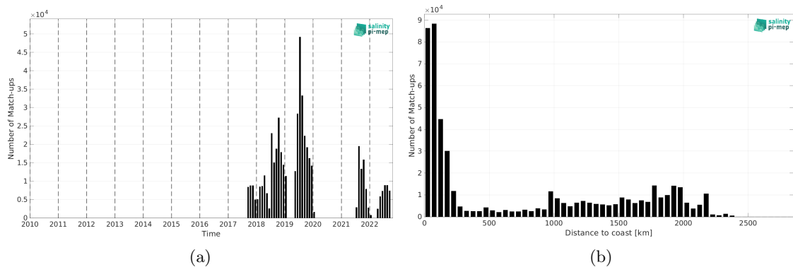
Figure 1: Number of match-ups between Saildrone and SMOS SSS L3 v8 - 18 Days (CATDS-CEC-LOCEAN) SSS as a function of time (a) and as function of the distance to coast (b) over the North Pacific Ocean Pi-MEP region and for the full satellite product period.
