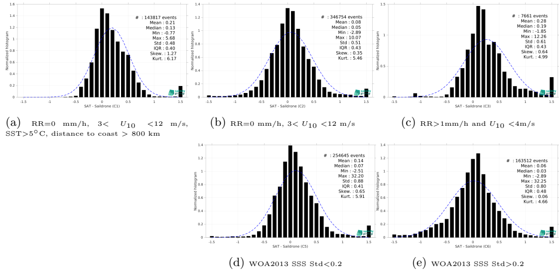
Figure 13: Normalized histogram of \Delta\text{SSS} (SMOS SSS L3 v8 - 18 Days (CATDS-CEC-LOCEAN) - Sailldrone) for 5 different subdatasets corresponding to: RR=0 mm/h, 3 < U_{10} < 12 m/s, SST>5°C, distance to coast > 800 km (a), RR=0 mm/h, 3 < U_{10} < 12 m/s (b), RR>1mm/h and U_{10} < 4 m/s (c), WOA2013 SSS Std<0.2 (d), WOA2013 SSS Std>0.2 (e).
