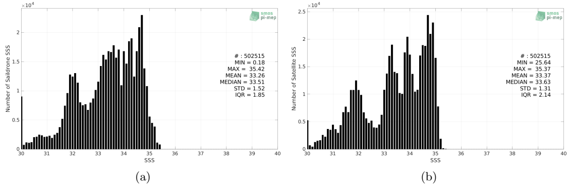
Figure 2: Histograms of SSS from Saildrone (a) and SMOS SSS L3 v8 - 18 Days (CATDS-CECOS-LOCEAN) (b) considering all match-up pairs per bins of 0.1 over the North Pacific Ocean Pi-MEP region and for the full satellite product period.
