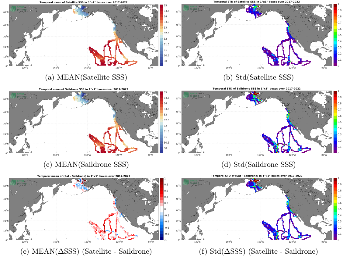
Figure 6: Temporal mean (left) and Std (right) of SSS from SMOS SSS L3 v8 - 18 Days (CATDS-CECOS-LOCEAN) (top), Saildrone (middle), and of \Delta\text{SSS} (Satellite - Saildrone). Only match-up pairs are used to generate these maps.
