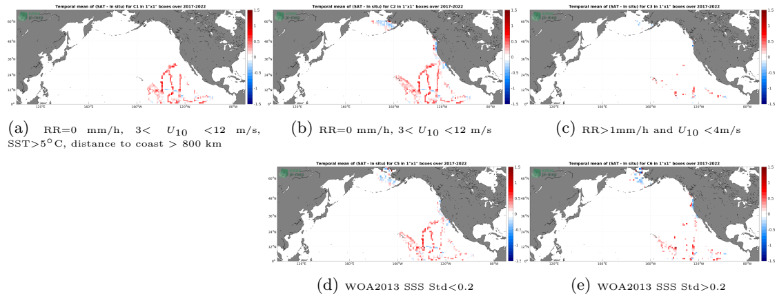
Figure 12: Temporal mean gridded over spatial boxes of size 1^\circ \times 1^\circ of \Delta SSS (SMOS SSS L3 v8 - 18 Days (CATDS-CECOS-LOCEAN) - Sairdrone) for 5 different subdatasets corresponding to:RR=0 mm/h, 3 < U_{10} < 12 m/s, SST >5^\circ C, distance to coast > 800 km (a), RR=0 mm/h, 3 < U_{10} < 12 m/s (b), RR >1 mm/h and U_{10} < 4 m/s (c), WOA2013 SSS Std <0.2 (d), WOA2013 SSS Std >0.2 (e).
