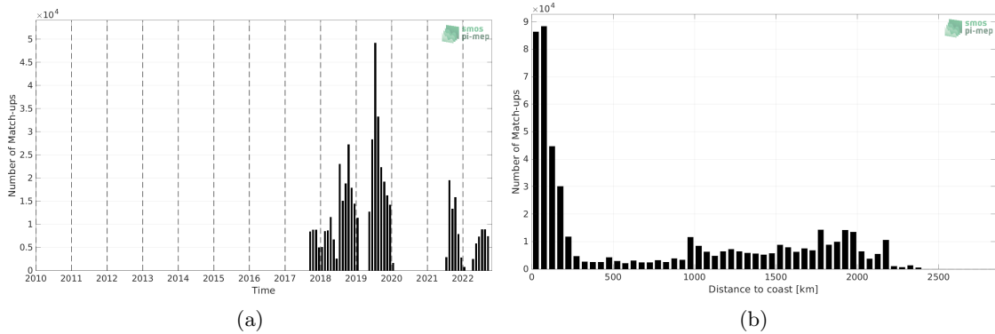
Figure 1: Number of match-ups between Saildrone and SMOS SSS L3 v8 - 18 Days (CATDS-CECOS-LOCEAN) SSS as a function of time (a) and as function of the distance to coast (b) over the North Pacific Ocean Pi-MEP region and for the full satellite product period.
