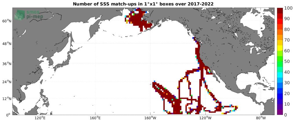
Figure 4: Number of SSS match-ups between Saildrone SSS and the SMOS SSS L3 v8 - 18 Days (CATDS-CECOS-LOCEAN) SSS product for the North Pacific Ocean Pi-MEP region over 1^\circ \times 1^\circ boxes and for the full satellite product period.
