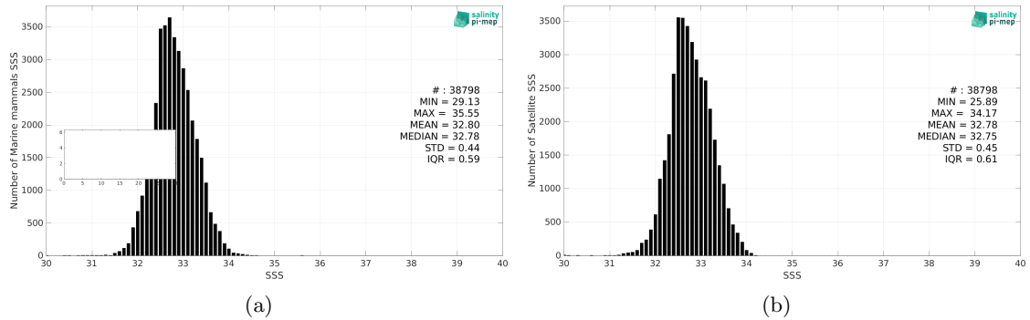
Figure 2: Histograms of SSS from Marine mammals (a) and SMOS SSS L3 v8 - 18 Days (CATDS-CEC-LOCEAN) (b) considering all match-up pairs per bins of 0.1 over the North Pacific Ocean Pi-MEP region and for the full satellite product period.
