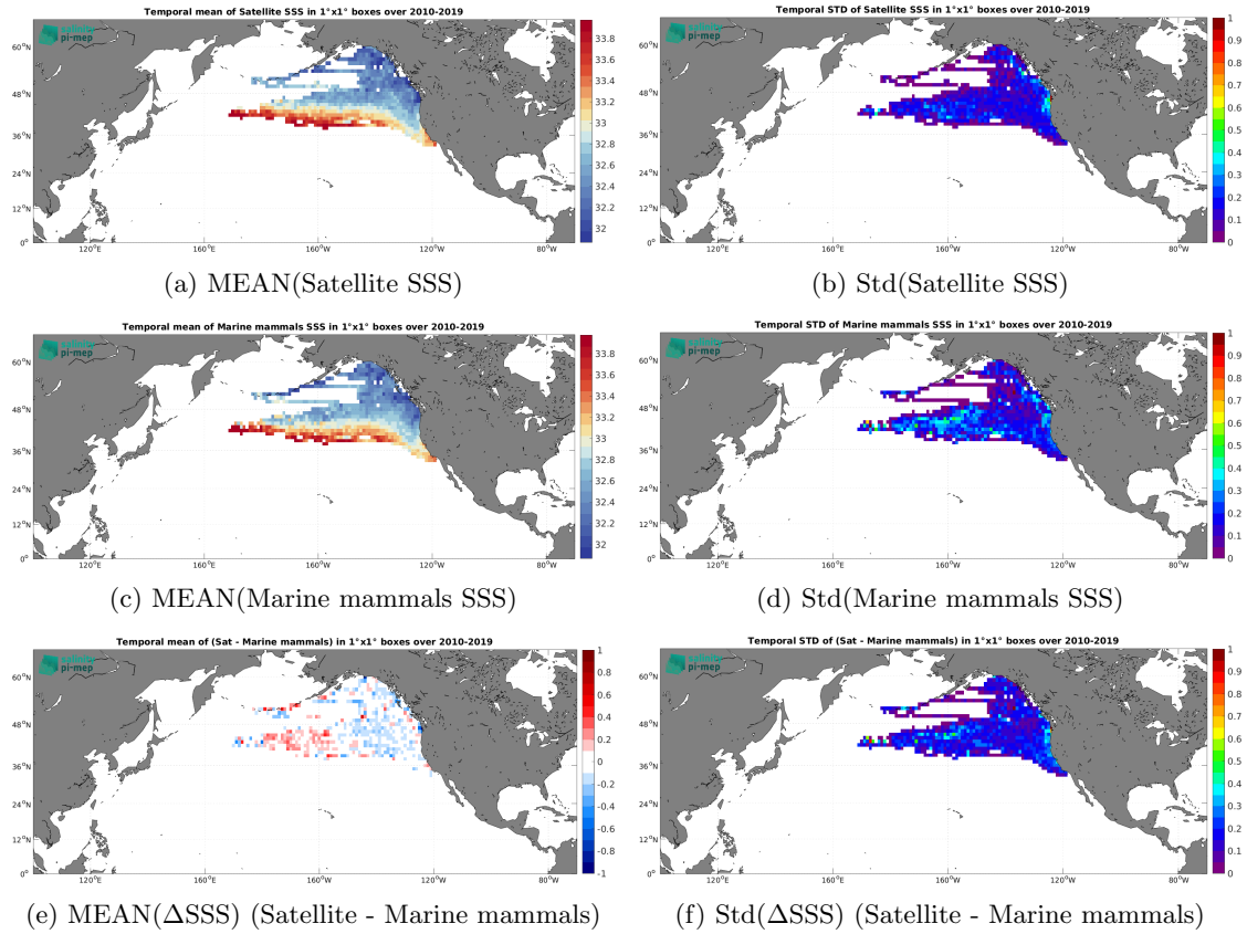
Figure 6: Temporal mean (left) and Std (right) of SSS from SMOS SSS L3 v8 - 18 Days (CATDS-CEC-LOCEAN) (top), Marine mammals (middle), and of \Delta SSS (Satellite - Marine mammals). Only match-up pairs are used to generate these maps.
