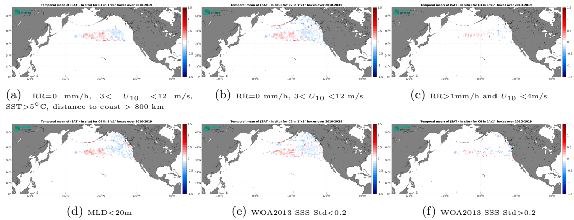
Figure 12: Temporal mean gridded over spatial boxes of size 1^{\circ}\times 1^{\circ} of \Delta\text{SSS} (SMOS SSS L3 v8 - 18 Days (CATDS-CEC-LOCEAN) - Marine mammals) for 6 different subdatasets corresponding to:RR=0 mm/h, 3 < U_{10} < 12 m/s, SST >5^{\circ}\text{C} , distance to coast > 800 km (a), RR=0 mm/h, 3 < U_{10} < 12 m/s (b), RR >1 mm/h and U_{10} < 4 m/s (c),MLD <20 m (d),WOA2013 SSS Std <0.2 (e),WOA2013 SSS Std >0.2 (f).
