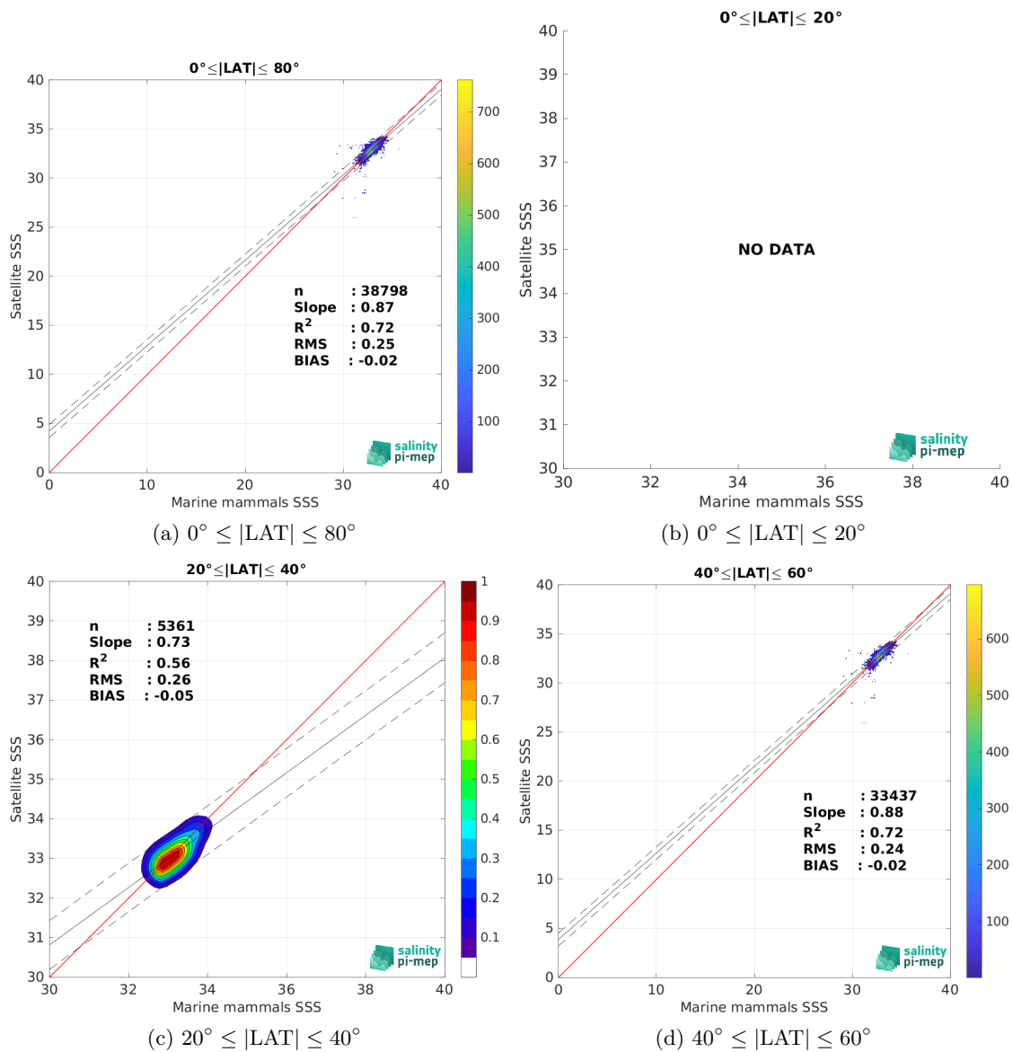
Figure 9: Contour maps of the concentration of SMOS SSS L3 v8 - 18 Days (CATDS-CEC-LOCEAN) SSS ( y -axis) versus Marine mammals SSS ( x -axis) at match-up pairs for different latitude bands. For each plot, the red line shows x=y . The black thin and dashed lines indicate a linear fit through the data cloud and the \pm 95\% confidence levels, respectively. The number match-up pairs n , the slope and R^2 coefficient of the linear fit, the root mean square (RMS) and the mean bias between satellite and in situ data are indicated for each latitude band in each plots.
