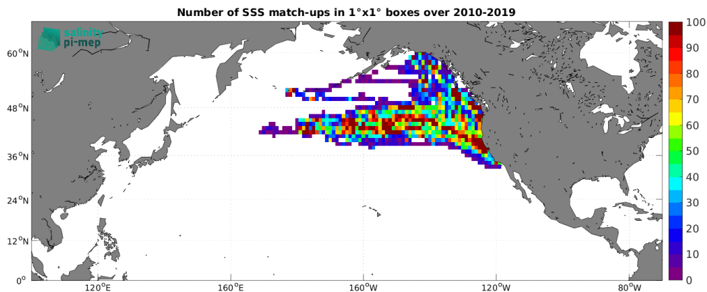
Figure 4: Number of SSS match-ups between Marine mammals SSS and the SMOS SSS L3 v8 - 18 Days (CATDS-CEC-LOCEAN) SSS product for the North Pacific Ocean Pi-MEP region over 1^\circ \times 1^\circ boxes and for the full satellite product period.
