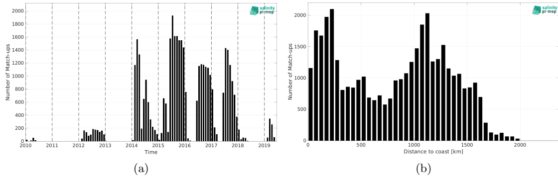
Figure 1: Number of match-ups between Marine mammals and SMOS SSS L3 v8 - 18 Days (CATDS-CEC-LOCEAN) SSS as a function of time (a) and as function of the distance to coast (b) over the North Pacific Ocean Pi-MEP region and for the full satellite product period.
