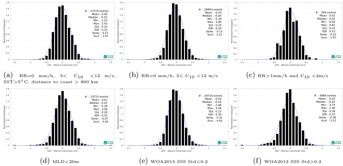
Figure 13: Normalized histogram of \Delta SSS (SMOS SSS L3 v8 - 18 Days (CATDS-CEC-LOCEAN) - Marine mammals) for 6 different subdatasets corresponding to: RR=0 mm/h, 3 < U_{10} < 12 m/s, SST > 5°C, distance to coast > 800 km (a), RR=0 mm/h, 3 < U_{10} < 12 m/s (b), RR > 1mm/h and U_{10} < 4 m/s (c), MLD < 20m (d), WOA2013 SSS Std < 0.2 (e), WOA2013 SSS Std > 0.2 (f).
