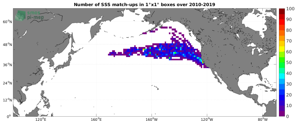
Figure 4: Number of SSS match-ups between Marine mammals SSS and the SMOS SSS L3 v8 - 18 Days (CATDS-CECOS-LOCEAN) SSS product for the North Pacific Ocean Pi-MEP region over 1^\circ \times 1^\circ boxes and for the full satellite product period.
