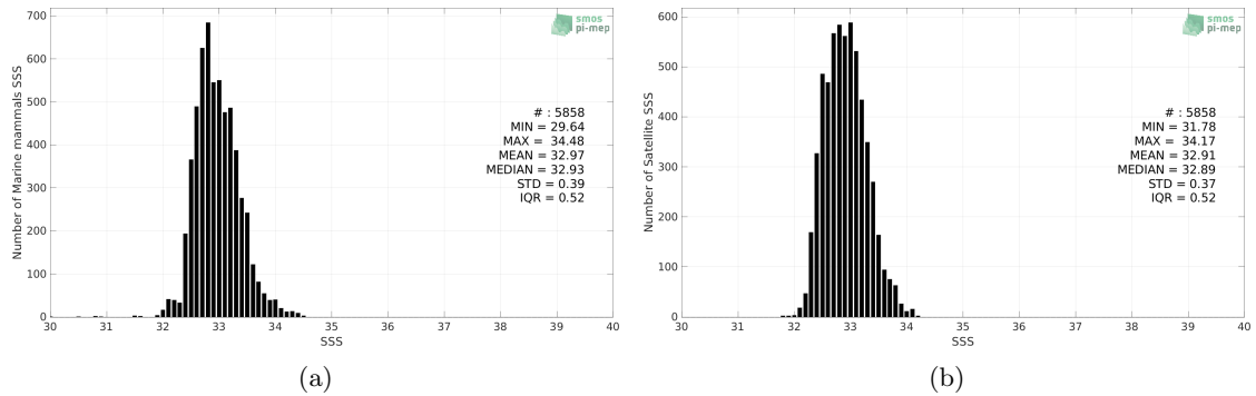
Figure 2: Histograms of SSS from Marine mammals (a) and SMOS SSS L3 v8 - 18 Days (CATDS-CECOS-LOCEAN) (b) considering all match-up pairs per bins of 0.1 over the North Pacific Ocean Pi-MEP region and for the full satellite product period.
