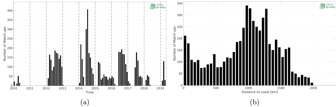
Figure 1: Number of match-ups between Marine mammals and SMOS SSS L3 v8 - 18 Days (CATDS-CECOS-LOCEAN) SSS as a function of time (a) and as function of the distance to coast (b) over the North Pacific Ocean Pi-MEP region and for the full satellite product period.
