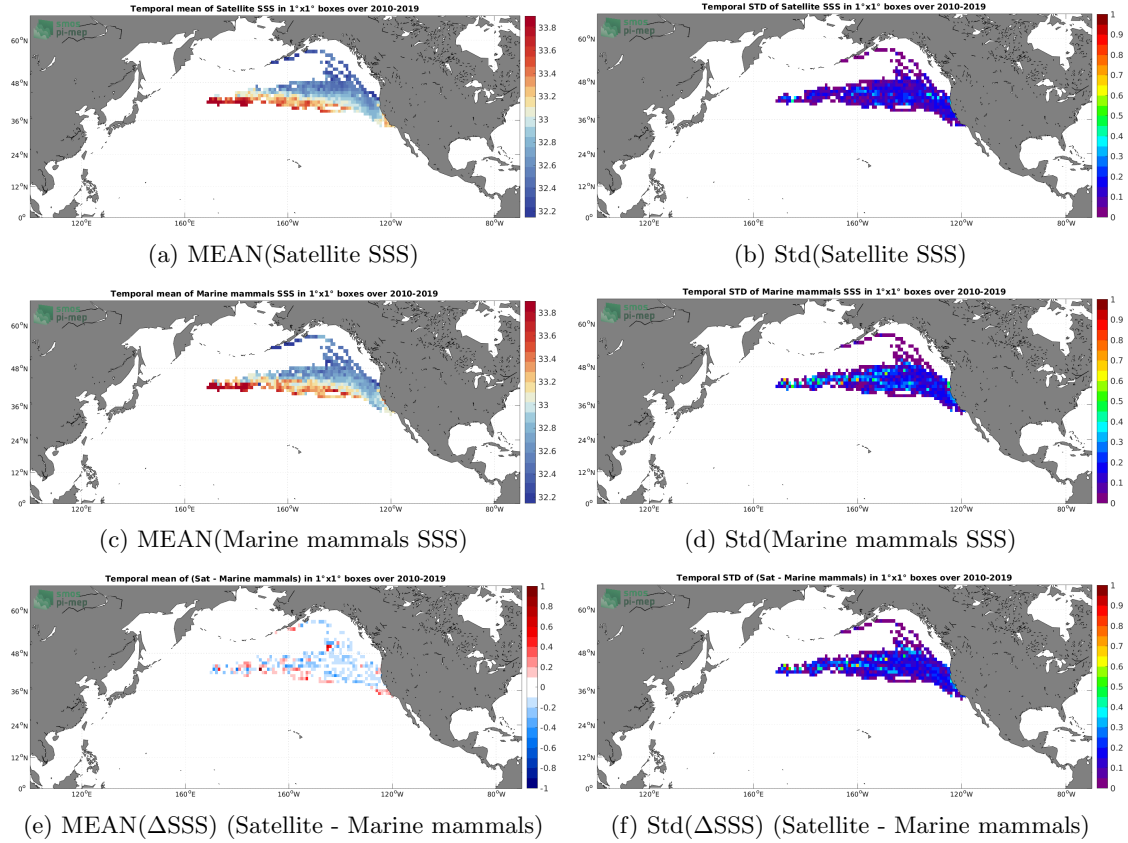
Figure 6: Temporal mean (left) and Std (right) of SSS from SMOS SSS L3 v8 - 18 Days (CATDS-CECOS-LOCEAN) (top), Marine mammals (middle), and of \Delta SSS (Satellite - Marine mammals). Only match-up pairs are used to generate these maps.
