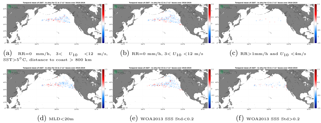
Figure 12: Temporal mean gridded over spatial boxes of size 1^{\circ}\times 1^{\circ} of \Delta\text{SSS} (SMOS SSS L3 v8 - 18 Days (CATDS-CECOS-LOCEAN) - Marine mammals) for 6 different subdatasets corresponding to:RR=0 mm/h, 3 < U_{10} < 12 m/s, SST >5^{\circ}\text{C} , distance to coast > 800 km (a), RR=0 mm/h, 3 < U_{10} < 12 m/s (b), RR >1 mm/h and U_{10} < 4 m/s (c),MLD <20 m (d),WOA2013 SSS Std <0.2 (e),WOA2013 SSS Std >0.2 (f).
