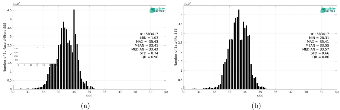
Figure 2: Histograms of SSS from Surface drifters (a) and SMOS SSS L3 v8 - 18 Days (CATDS-CEC-LOCEAN) (b) considering all match-up pairs per bins of 0.1 over the North Pacific Ocean Pi-MEP region and for the full satellite product period.
