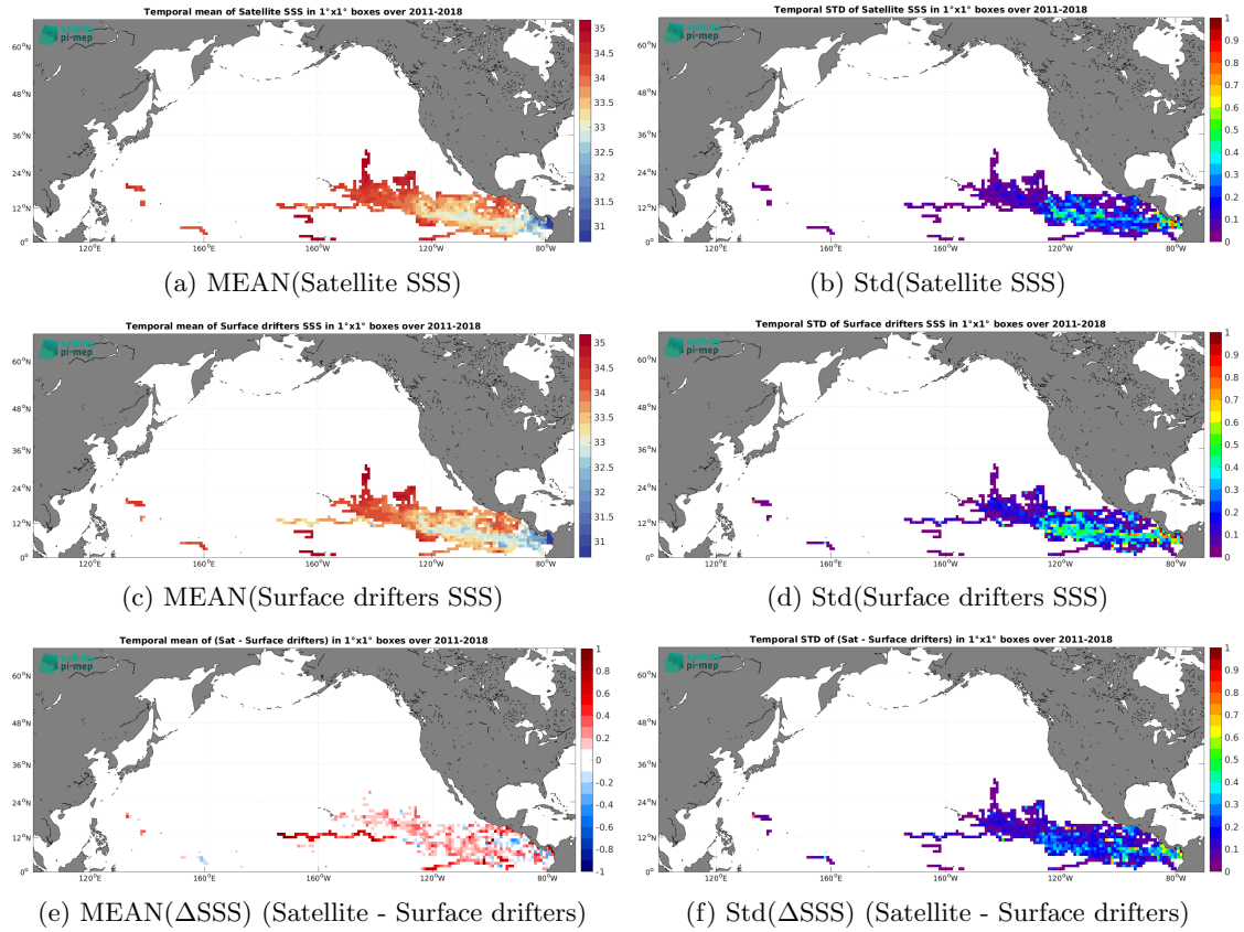
Figure 5: Temporal mean (left) and Std (right) of SSS from SMOS SSS L3 v8 - 18 Days (CATDS-CEC-LOCEAN) (top), Surface drifters (middle), and of \Delta SSS (Satellite - Surface drifters). Only match-up pairs are used to generate these maps.
