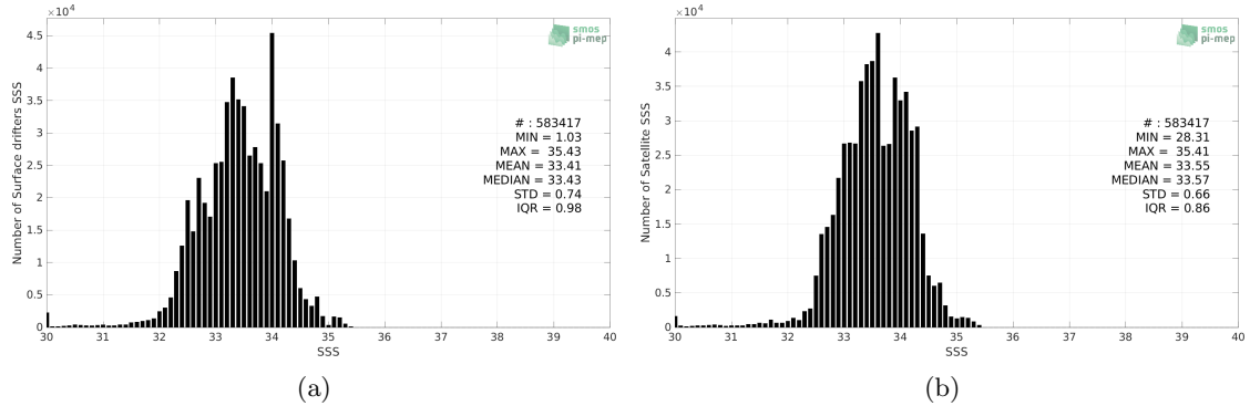
Figure 2: Histograms of SSS from Surface drifters (a) and SMOS SSS L3 v8 - 18 Days (CATDS-CECOS-LOCEAN) (b) considering all match-up pairs per bins of 0.1 over the North Pacific Ocean Pi-MEP region and for the full satellite product period.
