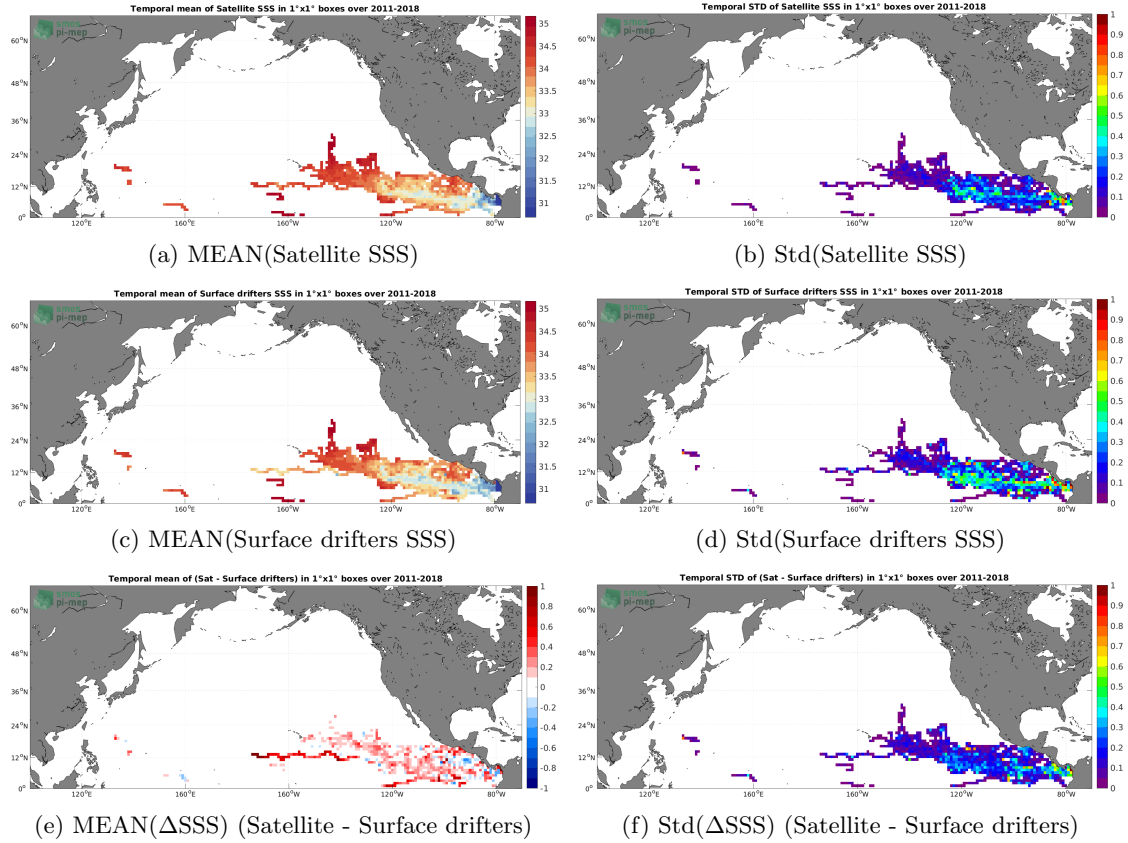
Figure 5: Temporal mean (left) and Std (right) of SSS from SMOS SSS L3 v8 - 18 Days (CATDS-CECOS-LOCEAN) (top), Surface drifters (middle), and of \Delta SSS (Satellite - Surface drifters). Only match-up pairs are used to generate these maps.
