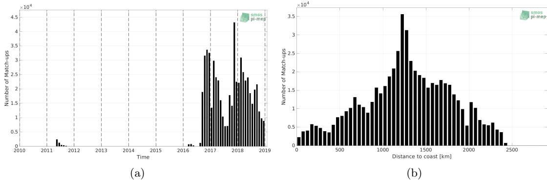
Figure 1: Number of match-ups between Surface drifters and SMOS SSS L3 v8 - 18 Days (CATDS-CECOS-LOCEAN) SSS as a function of time (a) and as function of the distance to coast (b) over the North Pacific Ocean Pi-MEP region and for the full satellite product period.
