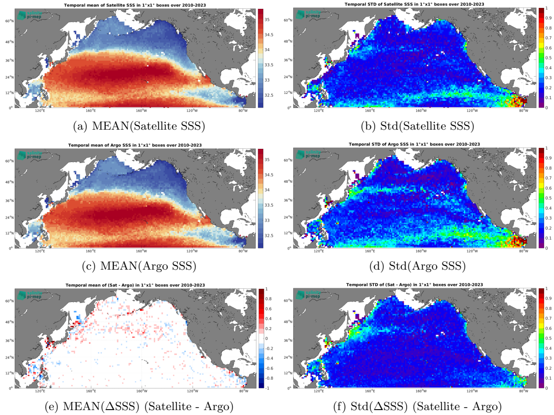
Figure 6: Temporal mean (left) and Std (right) of SSS from SMOS SSS L3 v8 - 18 Days (CATDS-CEC-LOCEAN) (top), Argo (middle), and of \Delta SSS (Satellite - Argo). Only match-up pairs are used to generate these maps.
