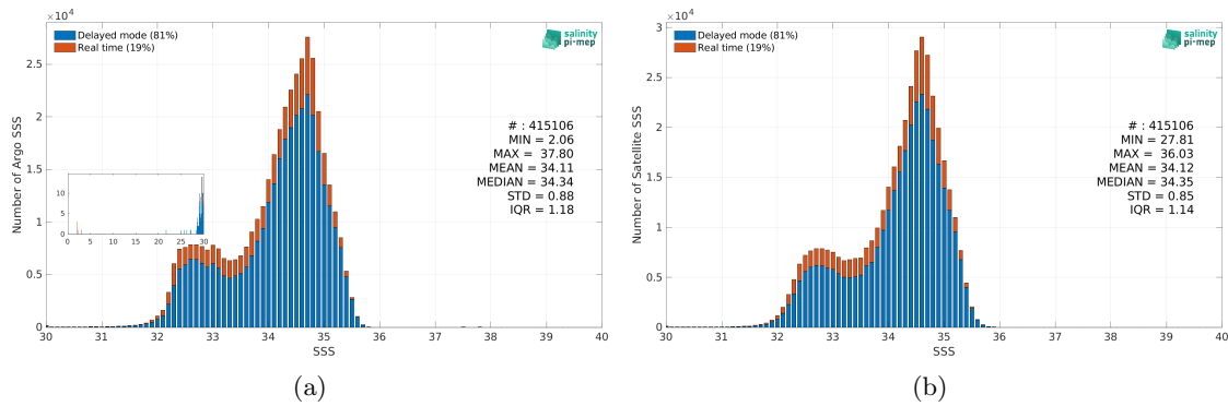
Figure 2: Histograms of SSS from Argo (a) and SMOS SSS L3 v8 - 18 Days (CATDS-CEC-LOCEAN) (b) considering all match-up pairs per bins of 0.1 over the North Pacific Ocean Pi-MEP region and for the full satellite product period.
