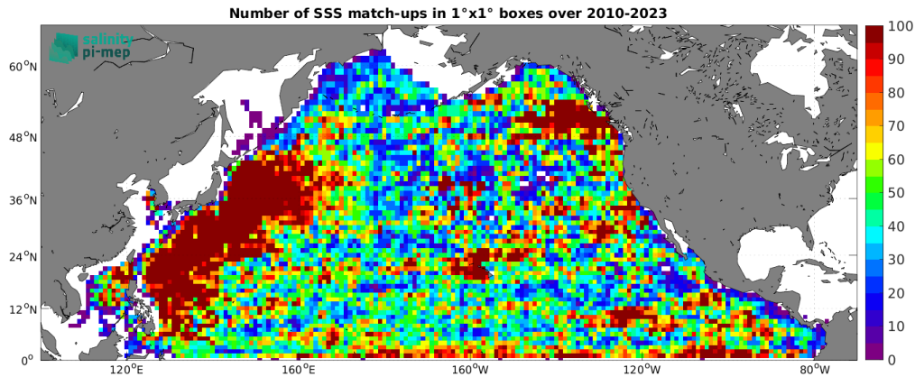
Figure 4: Number of SSS match-ups between Argo SSS and the SMOS SSS L3 v8 - 18 Days (CATDS-CEC-LOCEAN) SSS product for the North Pacific Ocean Pi-MEP region over 1^\circ \times 1^\circ boxes and for the full satellite product period.
