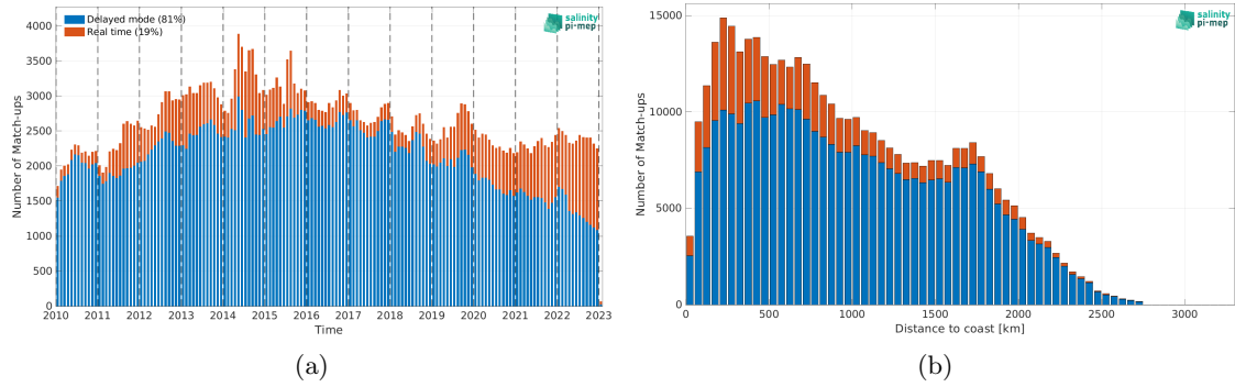
Figure 1: Number of match-ups between Argo and SMOS SSS L3 v8 - 18 Days (CATDS-CEC-LOCEAN) SSS as a function of time (a) and as function of the distance to coast (b) over the North Pacific Ocean Pi-MEP region and for the full satellite product period.
