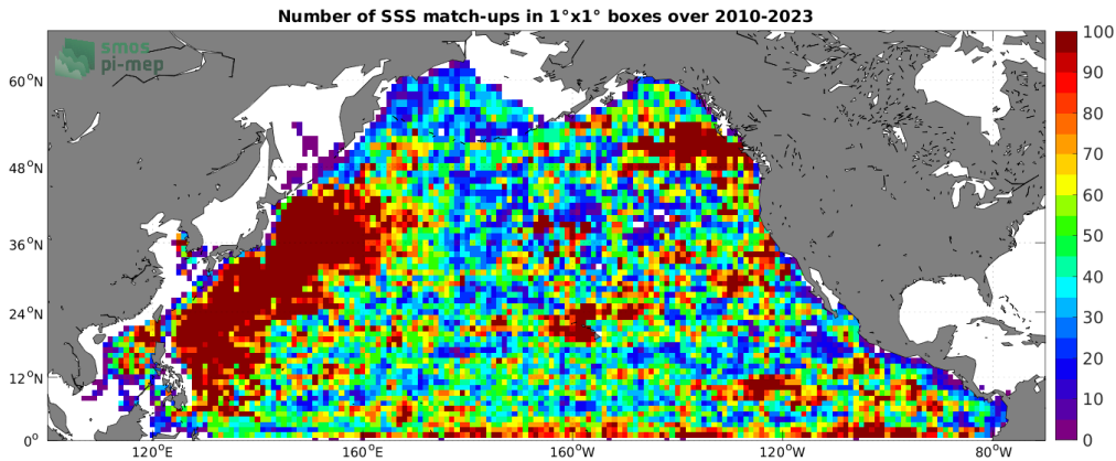
Figure 4: Number of SSS match-ups between Argo SSS and the SMOS SSS L3 v8 - 18 Days (CATDS-CECOS-LOCEAN) SSS product for the North Pacific Ocean Pi-MEP region over 1^\circ \times 1^\circ boxes and for the full satellite product period.
