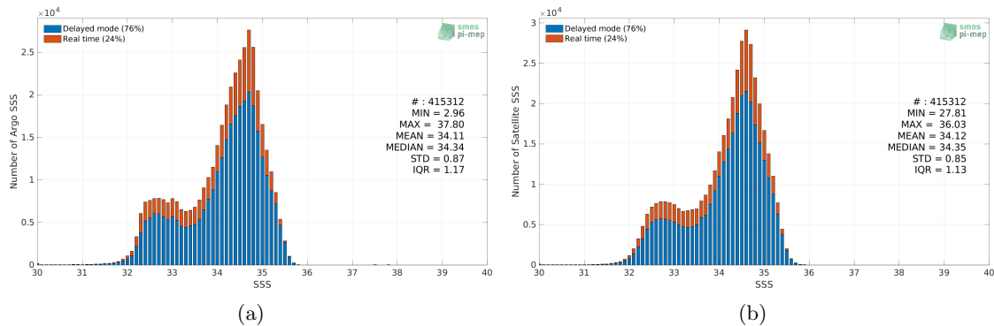
Figure 2: Histograms of SSS from Argo (a) and SMOS SSS L3 v8 - 18 Days (CATDS-CECOS-LOCEAN) (b) considering all match-up pairs per bins of 0.1 over the North Pacific Ocean Pi-MEP region and for the full satellite product period.
