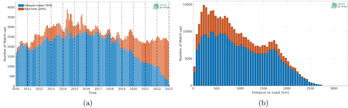
Figure 1: Number of match-ups between Argo and SMOS SSS L3 v8 - 18 Days (CATDS-CECOS-LOCEAN) SSS as a function of time (a) and as function of the distance to coast (b) over the North Pacific Ocean Pi-MEP region and for the full satellite product period.
