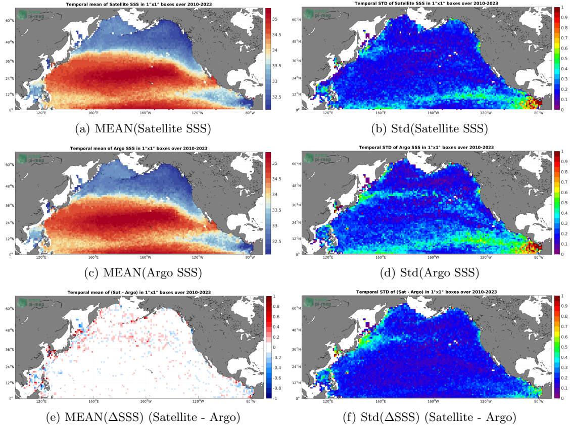
Figure 6: Temporal mean (left) and Std (right) of SSS from SMOS SSS L3 v8 - 18 Days (CATDS-CECOS-LOCEAN) (top), Argo (middle), and of \Delta SSS (Satellite - Argo). Only match-up pairs are used to generate these maps.
