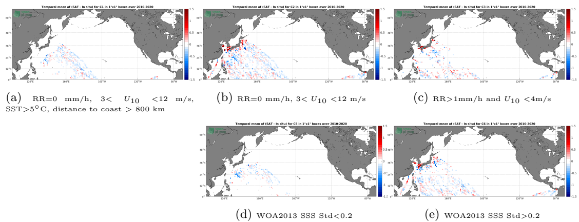
Figure 12: Temporal mean gridded over spatial boxes of size 1^\circ \times 1^\circ of \Delta\text{SSS} (SMOS SSS L3 v7 - 9 Days (CATDS-CECOS-LOCEAN) - TSG (LEGOS-DM)) for 5 different subdatasets corresponding to:RR=0 mm/h, 3 < U_{10} < 12 m/s, SST >5^\circ\text{C} , distance to coast > 800 km (a), RR=0 mm/h, 3 < U_{10} < 12 m/s (b), RR >1 mm/h and U_{10} < 4 m/s (c), WOA2013 SSS Std <0.2 (d), WOA2013 SSS Std >0.2 (e).
