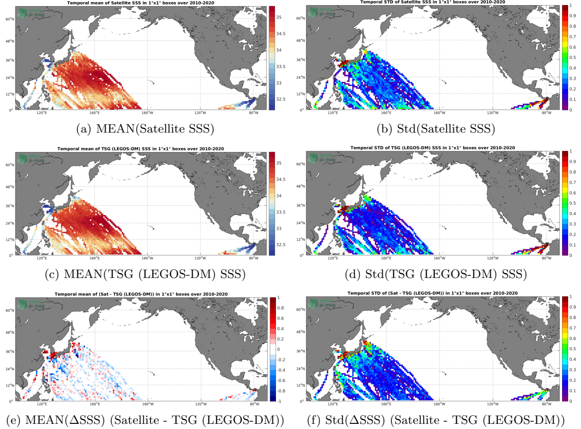
Figure 6: Temporal mean (left) and Std (right) of SSS from SMOS SSS L3 v7 - 9 Days (CATDS-CECOS-LOCEAN) (top), TSG (LEGOS-DM) ( in situ dataset) (middle), and of \Delta\text{SSS} (Satellite - TSG (LEGOS-DM)). Only match-up pairs are used to generate these maps.
