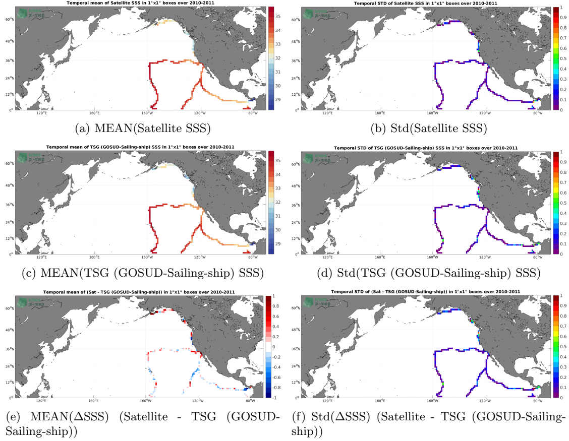
Figure 6: Temporal mean (left) and Std (right) of SSS from SMOS SSS L3 v7 - 9 Days (CATDS-CECOS-LOCEAN) (top), TSG (GOSUD-Sailing-ship) (middle), and of \Delta SSS (Satellite - TSG (GOSUD-Sailing-ship)). Only match-up pairs are used to generate these maps.
