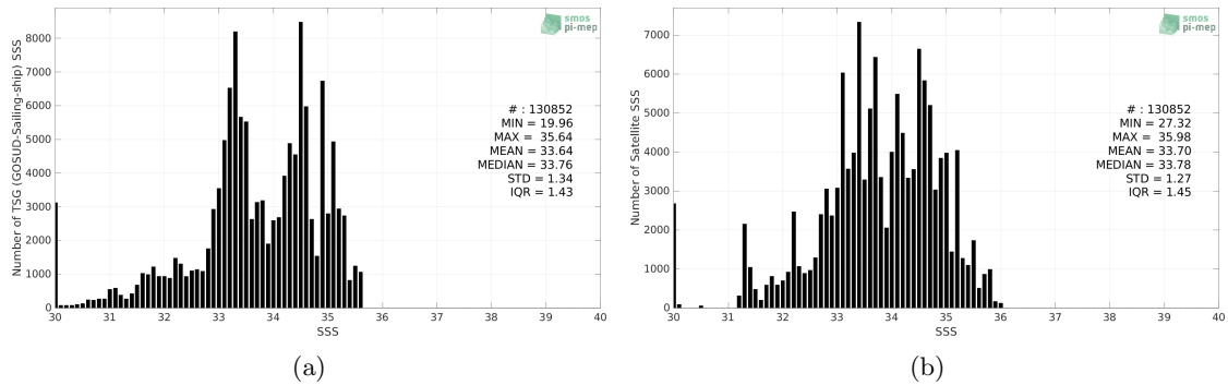
Figure 2: Histograms of SSS from TSG (GOSUD-Sailing-ship) (a) and SMOS SSS L3 v7 - 9 Days (CATDS-CECOS-LOCEAN) (b) considering all match-up pairs per bins of 0.1 over the North Pacific Ocean Pi-MEP region and for the full satellite product period.
