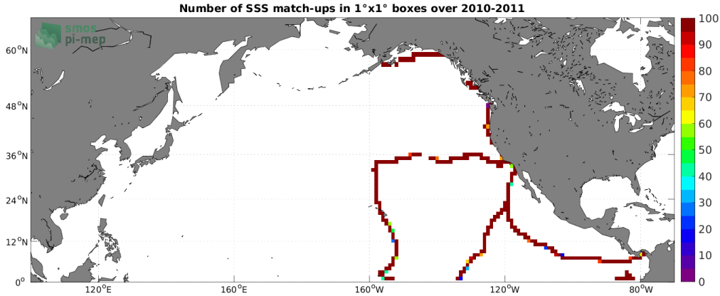
Figure 4: Number of SSS match-ups between TSG (GOSUD-Sailing-ship) SSS and the SMOS SSS L3 v7 - 9 Days (CATDS-CECOS-LOCEAN) SSS product for the North Pacific Ocean Pi-MEP region over 1^\circ \times 1^\circ boxes and for the full satellite product period.
