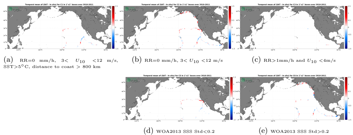
Figure 12: Temporal mean gridded over spatial boxes of size 1^\circ \times 1^\circ of \Delta SSS (SMOS SSS L3 v7 - 9 Days (CATDS-CECOS-LOCEAN) - TSG (GOSUD-Sailing-ship)) for 5 different subdatasets corresponding to:RR=0 mm/h, 3 < U_{10} < 12 m/s, SST>5°C, distance to coast > 800 km (a), RR=0 mm/h, 3 < U_{10} < 12 m/s (b), RR>1mm/h and U_{10} < 4 m/s (c), WOA2013 SSS Std<0.2 (d), WOA2013 SSS Std>0.2 (e).
