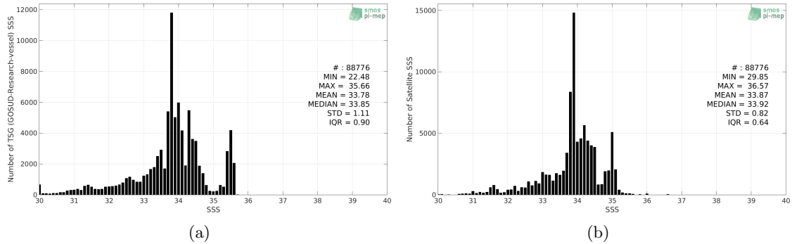
Figure 2: Histograms of SSS from TSG (GOSUD-Research-vessel) (a) and SMOS SSS L3 v7 - 9 Days (CATDS-CECOS-LOCEAN) (b) considering all match-up pairs per bins of 0.1 over the North Pacific Ocean Pi-MEP region and for the full satellite product period.
