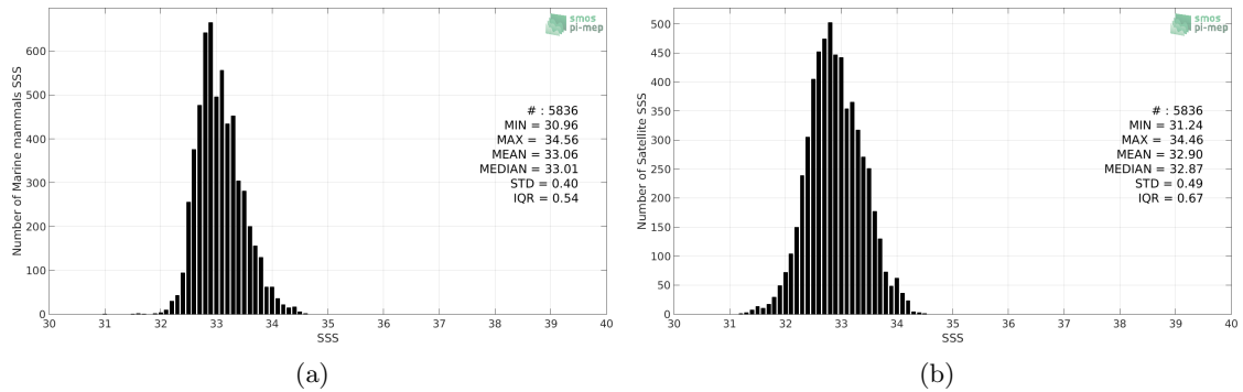
Figure 2: Histograms of SSS from Marine mammals (a) and SMOS SSS L3 v7 - 9 Days (CATDS-CECOS-LOCEAN) (b) considering all match-up pairs per bins of 0.1 over the North Pacific Ocean Pi-MEP region and for the full satellite product period.
