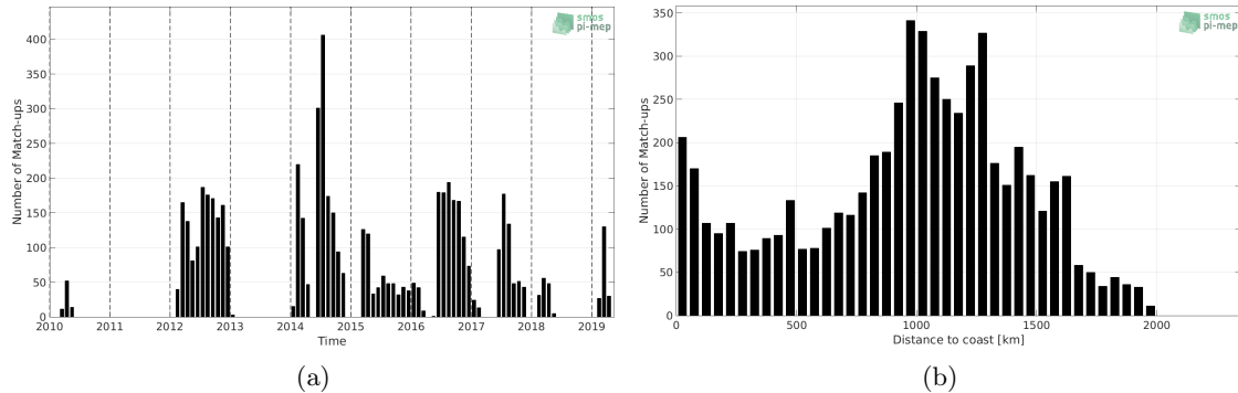
Figure 1: Number of match-ups between Marine mammals and SMOS SSS L3 v7 - 9 Days (CATDS-CECOS-LOCEAN) SSS as a function of time (a) and as function of the distance to coast (b) over the North Pacific Ocean Pi-MEP region and for the full satellite product period.
