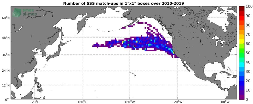
Figure 4: Number of SSS match-ups between Marine mammals SSS and the SMOS SSS L3 v7 - 9 Days (CATDS-CECOS-LOCEAN) SSS product for the North Pacific Ocean Pi-MEP region over 1^\circ \times 1^\circ boxes and for the full satellite product period.
