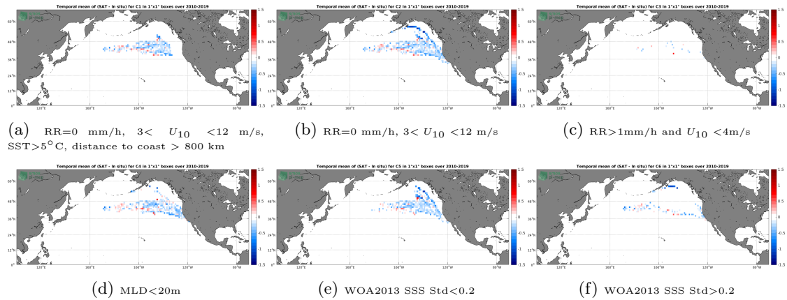
Figure 12: Temporal mean gridded over spatial boxes of size 1^{\circ}\times 1^{\circ} of \Delta\text{SSS} (SMOS SSS L3 v7 - 9 Days (CATDS-CECOS-LOCEAN) - Marine mammals) for 6 different subdatasets corresponding to:RR=0 mm/h, 3 < U_{10} < 12 m/s, SST >5^{\circ}\text{C} , distance to coast > 800 km (a), RR=0 mm/h, 3 < U_{10} < 12 m/s (b), RR >1 mm/h and U_{10} < 4 m/s (c),MLD <20 m (d),WOA2013 SSS Std <0.2 (e),WOA2013 SSS Std >0.2 (f).
