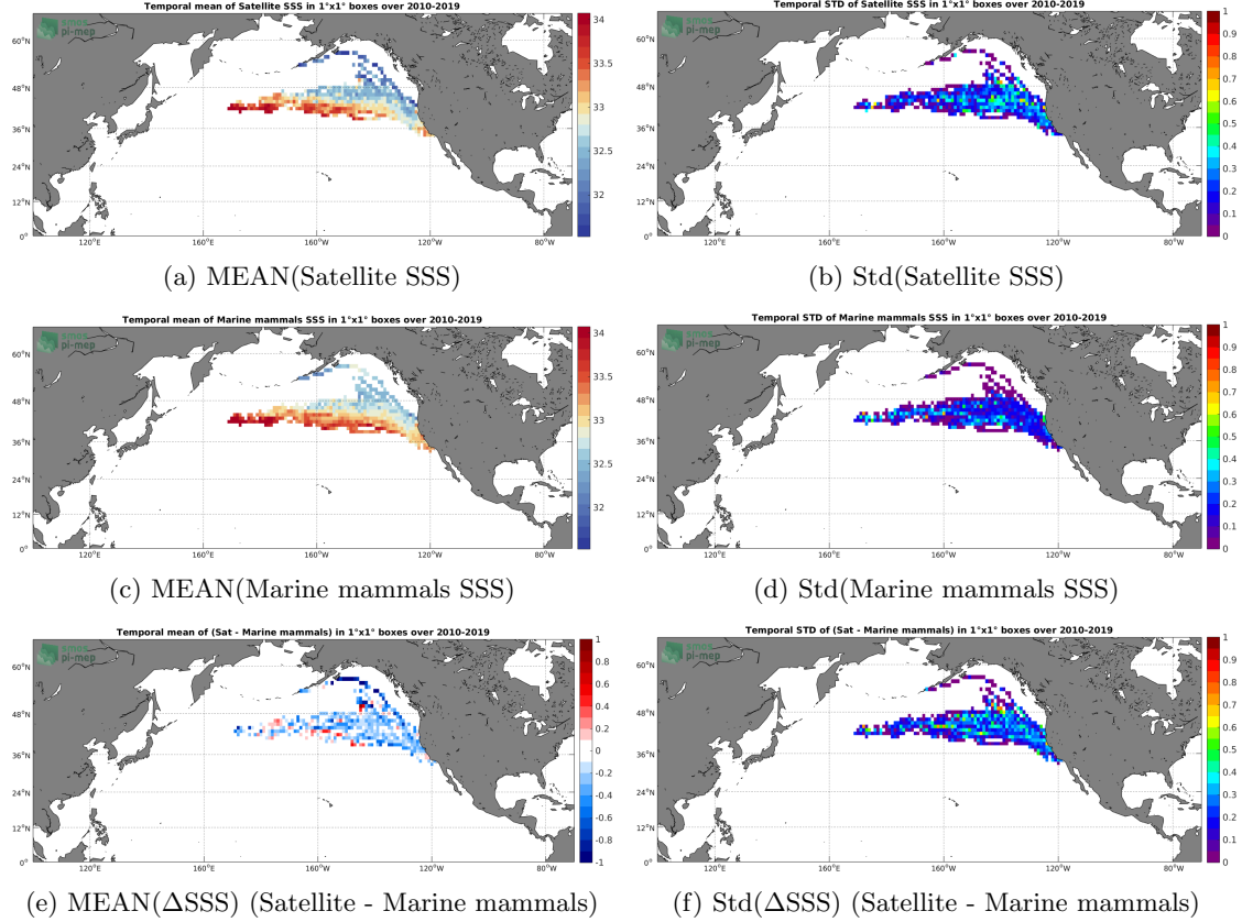
Figure 6: Temporal mean (left) and Std (right) of SSS from SMOS SSS L3 v7 - 9 Days (CATDS-CECOS-LOCEAN) (top), Marine mammals (middle), and of \Delta SSS (Satellite - Marine mammals). Only match-up pairs are used to generate these maps.
