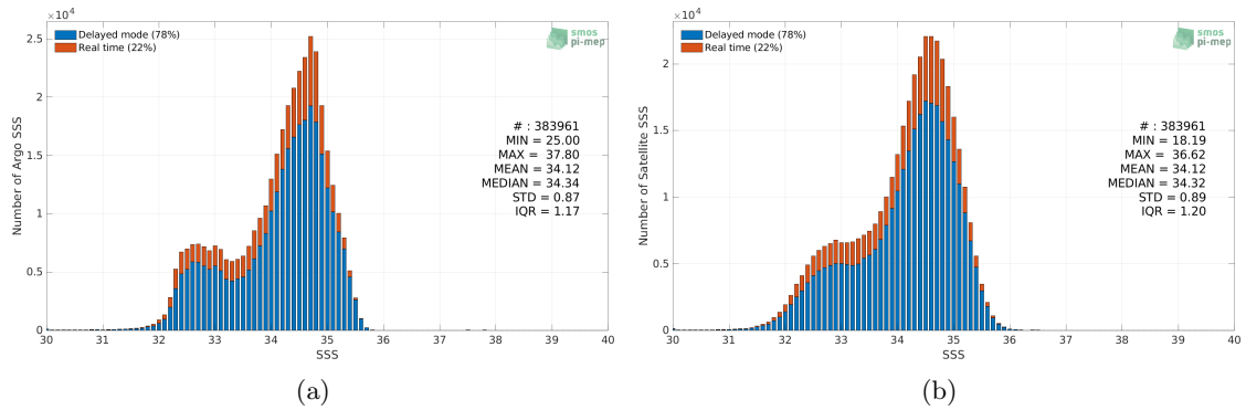
Figure 2: Histograms of SSS from Argo (a) and SMOS SSS L3 v7 - 9 Days (CATDS-CECOS-LOCEAN) (b) considering all match-up pairs per bins of 0.1 over the North Pacific Ocean Pi-MEP region and for the full satellite product period.
