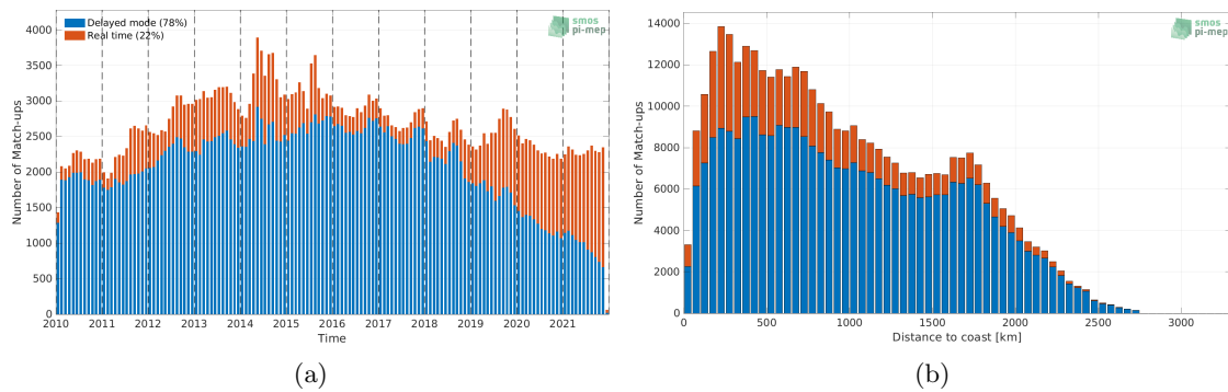
Figure 1: Number of match-ups between Argo and SMOS SSS L3 v7 - 9 Days (CATDS-CECOS-LOCEAN) SSS as a function of time (a) and as function of the distance to coast (b) over the North Pacific Ocean Pi-MEP region and for the full satellite product period.
