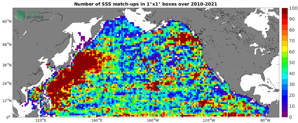
Figure 4: Number of SSS match-ups between Argo SSS and the SMOS SSS L3 v7 - 9 Days (CATDS-CECOS-LOCEAN) SSS product for the North Pacific Ocean Pi-MEP region over 1^\circ \times 1^\circ boxes and for the full satellite product period.
