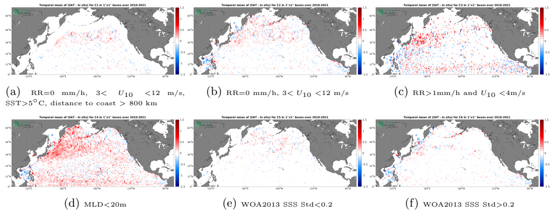
Figure 12: Temporal mean gridded over spatial boxes of size 1^\circ \times 1^\circ of \Delta SSS (SMOS SSS L3 v7 - 9 Days (CATDS-CECOS-LOCEAN) - Argo) for 6 different subdatasets corresponding to:RR=0 mm/h, 3 < U_{10} < 12 m/s, SST >5^\circ C, distance to coast > 800 km (a), RR=0 mm/h, 3 < U_{10} < 12 m/s (b), RR >1 mm/h and U_{10} < 4 m/s (c),MLD <20 m (d),WOA2013 SSS Std <0.2 (e),WOA2013 SSS Std >0.2 (f).
