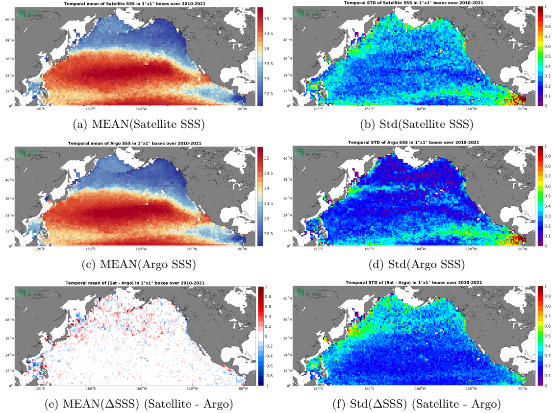
Figure 6: Temporal mean (left) and Std (right) of SSS from SMOS SSS L3 v7 - 9 Days (CATDS-CECOS-LOCEAN) (top), Argo (middle), and of \Delta\text{SSS} (Satellite - Argo). Only match-up pairs are used to generate these maps.
