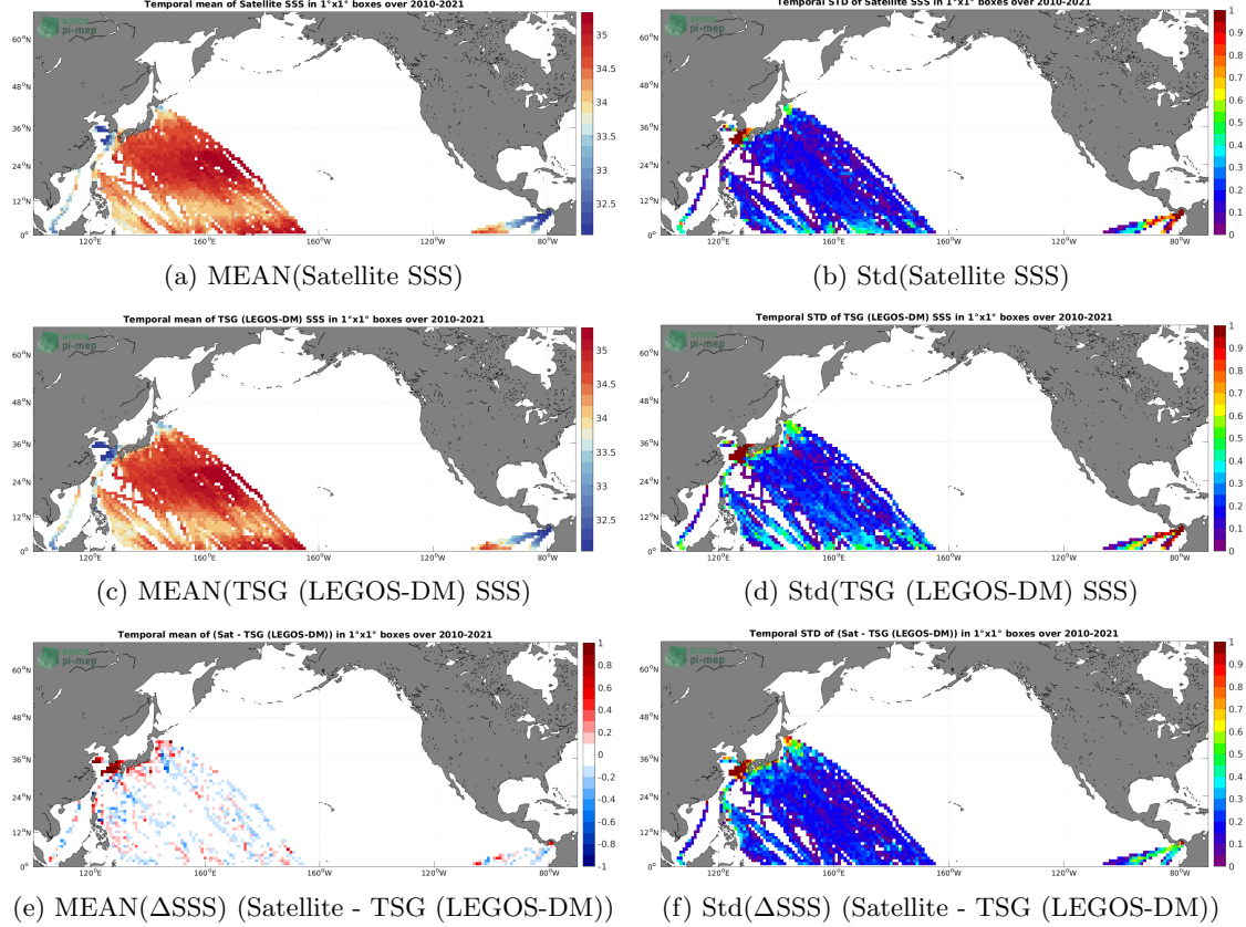
(a) MEAN(Satellite SSS) (b) Std(Satellite SSS) (c) MEAN(TSG (LEGOS-DM) SSS) (d) Std(TSG (LEGOS-DM) SSS) (e) MEAN( \Delta\text{SSS} ) (Satellite - TSG (LEGOS-DM)) (f) Std( \Delta\text{SSS} ) (Satellite - TSG (LEGOS-DM)) Figure 6: Temporal mean (left) and Std (right) of SSS from SMOS SSS L3 v7 - 18 Days (CATDS-CECOS-LOCEAN) (top), TSG (LEGOS-DM) (middle), and of \Delta\text{SSS} (Satellite - TSG (LEGOS-DM)). Only match-up pairs are used to generate these maps.
