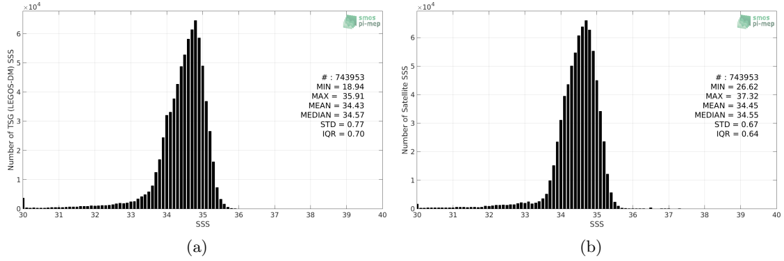
Figure 2: Histograms of SSS from TSG (LEGOS-DM) (a) and SMOS SSS L3 v7 - 18 Days (CATDS-CECOS-LOCEAN) (b) considering all match-up pairs per bins of 0.1 over the North Pacific Ocean Pi-MEP region and for the full satellite product period.
