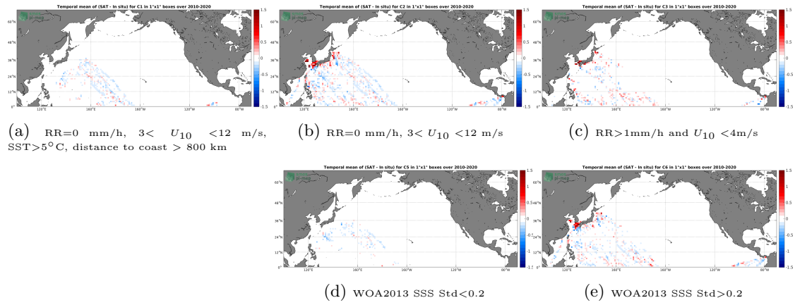
Figure 12: Temporal mean gridded over spatial boxes of size 1^\circ \times 1^\circ of \Delta SSS (SMOS SSS L3 v7 - 18 Days (CATDS-CECOS-LOCEAN) - TSG (LEGOS-DM)) for 5 different subdatasets corresponding to: RR=0 mm/h, 3 < U_{10} < 12 m/s, SST >5^\circ\text{C} , distance to coast > 800 km (a), RR=0 mm/h, 3 < U_{10} < 12 m/s (b), RR >1 mm/h and U_{10} < 4 m/s (c), WOA2013 SSS Std <0.2 (d), WOA2013 SSS Std >0.2 (e).
