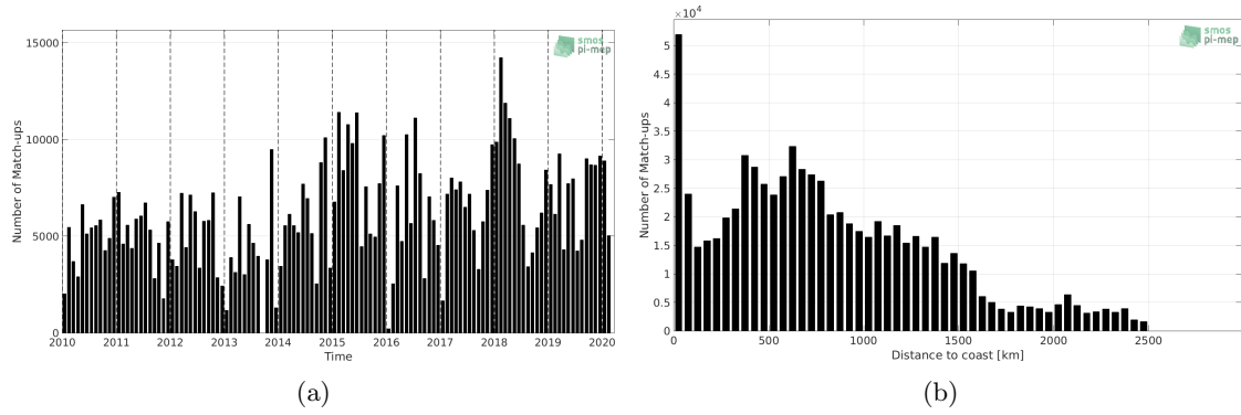
Figure 1: Number of match-ups between TSG (LEGOS-DM) and SMOS SSS L3 v7 - 18 Days (CATDS-CECOS-LOCEAN) SSS as a function of time (a) and as function of the distance to coast (b) over the North Pacific Ocean Pi-MEP region and for the full satellite product period.
