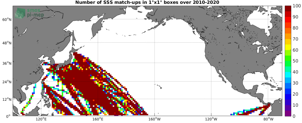
Figure 4: Number of SSS match-ups between TSG (LEGOS-DM) SSS and the SMOS SSS L3 v7 - 18 Days (CATDS-CECOS-LOCEAN) SSS product for the North Pacific Ocean Pi-MEP region over 1^\circ \times 1^\circ boxes and for the full satellite product period.
