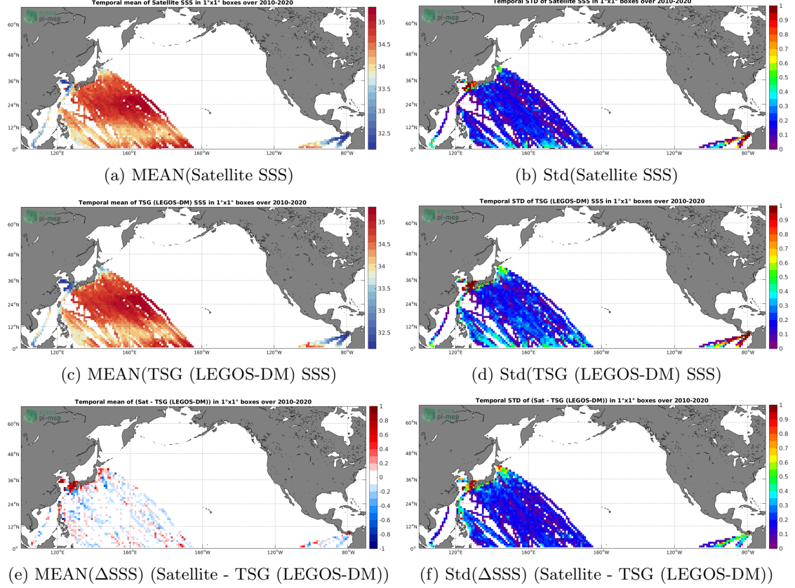
Figure 6: Temporal mean (left) and Std (right) of SSS from SMOS SSS L3 v7 - 18 Days (CATDS-CECOS-LOCEAN) (top), TSG (LEGOS-DM) (middle), and of \Delta\text{SSS} (Satellite - TSG (LEGOS-DM)). Only match-up pairs are used to generate these maps.
