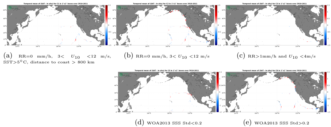
Figure 12: Temporal mean gridded over spatial boxes of size 1^\circ \times 1^\circ of \Delta\text{SSS} (SMOS SSS L3 v7 - 18 Days (CATDS-CECOS-LOCEAN) - TSG (GOSUD-Sailing-ship)) for 5 different subdatasets corresponding to:RR=0 mm/h, 3 < U_{10} < 12 m/s, SST >5^\circ\text{C} , distance to coast > 800 km (a), RR=0 mm/h, 3 < U_{10} < 12 m/s (b), RR >1 mm/h and U_{10} < 4 m/s (c), WOA2013 SSS Std <0.2 (d), WOA2013 SSS Std >0.2 (e).
