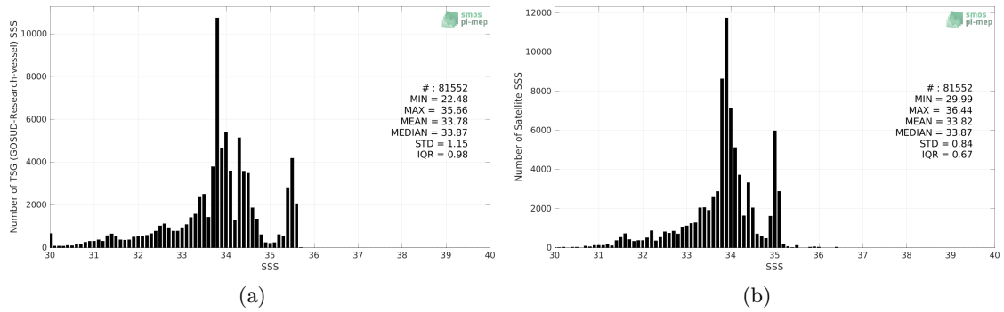
Figure 2: Histograms of SSS from TSG (GOSUD-Research-vessel) (a) and SMOS SSS L3 v7 - 18 Days (CATDS-CECOS-LOCEAN) (b) considering all match-up pairs per bins of 0.1 over the North Pacific Ocean Pi-MEP region and for the full satellite product period.
