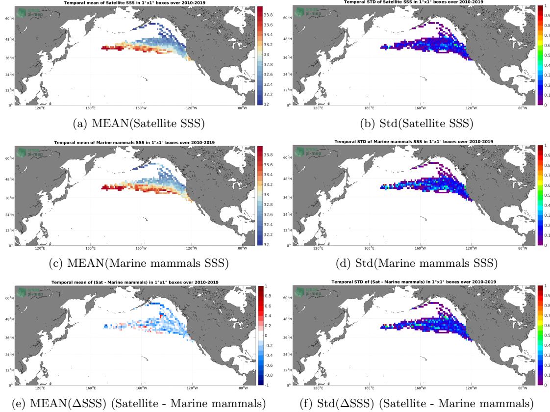
Figure 6: Temporal mean (left) and Std (right) of SSS from SMOS SSS L3 v7 - 18 Days (CATDS-CECOS-LOCEAN) (top), Marine mammals (middle), and of \Delta SSS (Satellite - Marine mammals). Only match-up pairs are used to generate these maps.
