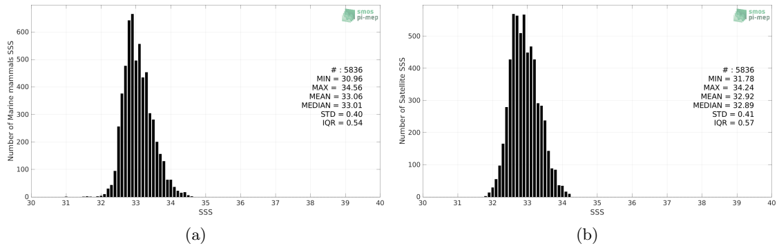
Figure 2: Histograms of SSS from Marine mammals (a) and SMOS SSS L3 v7 - 18 Days (CATDS-CECOS-LOCEAN) (b) considering all match-up pairs per bins of 0.1 over the North Pacific Ocean Pi-MEP region and for the full satellite product period.
