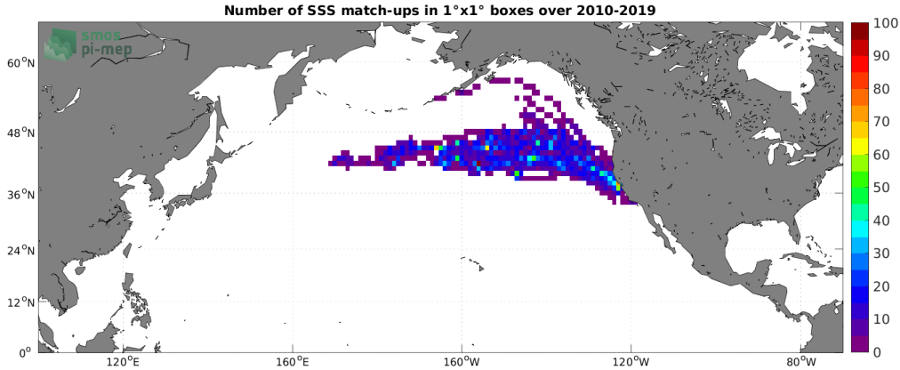
Figure 4: Number of SSS match-ups between Marine mammals SSS and the SMOS SSS L3 v7 - 18 Days (CATDS-CECOS-LOCEAN) SSS product for the North Pacific Ocean Pi-MEP region over 1^\circ \times 1^\circ boxes and for the full satellite product period.
