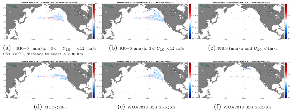
Figure 12: Temporal mean gridded over spatial boxes of size 1^{\circ}\times 1^{\circ} of \Delta\text{SSS} (SMOS SSS L3 v7 - 18 Days (CATDS-CECOS-LOCEAN) - Marine mammals) for 6 different subdatasets corresponding to:RR=0 mm/h, 3 < U_{10} < 12 m/s, SST > 5^{\circ}\text{C} , distance to coast > 800 km (a), RR=0 mm/h, 3 < U_{10} < 12 m/s (b), RR > 1\text{mm/h} and U_{10} < 4\text{m/s} (c),MLD < 20\text{m} (d),WOA2013 SSS Std < 0.2 (e),WOA2013 SSS Std > 0.2 (f).
