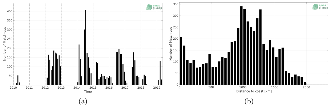
Figure 1: Number of match-ups between Marine mammals and SMOS SSS L3 v7 - 18 Days (CATDS-CECOS-LOCEAN) SSS as a function of time (a) and as function of the distance to coast (b) over the North Pacific Ocean Pi-MEP region and for the full satellite product period.
