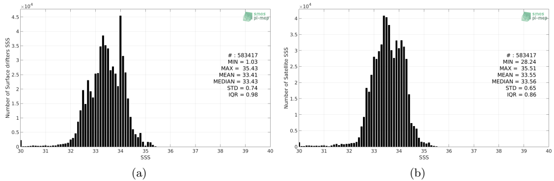
Figure 2: Histograms of SSS from Surface drifters (a) and SMOS SSS L3 v7 - 18 Days (CATDS-CECOS-LOCEAN) (b) considering all match-up pairs per bins of 0.1 over the North Pacific Ocean Pi-MEP region and for the full satellite product period.
