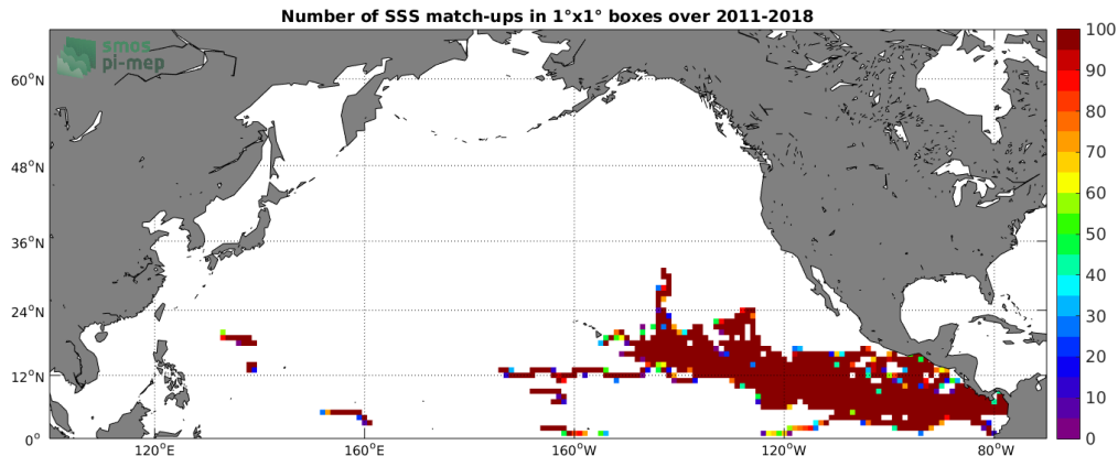
Figure 3: Number of SSS match-ups between Surface drifters SSS and the SMOS SSS L3 v7 - 18 Days (CATDS-CECOS-LOCEAN) SSS product for the North Pacific Ocean Pi-MEP region over 1^\circ \times 1^\circ boxes and for the full satellite product period.
