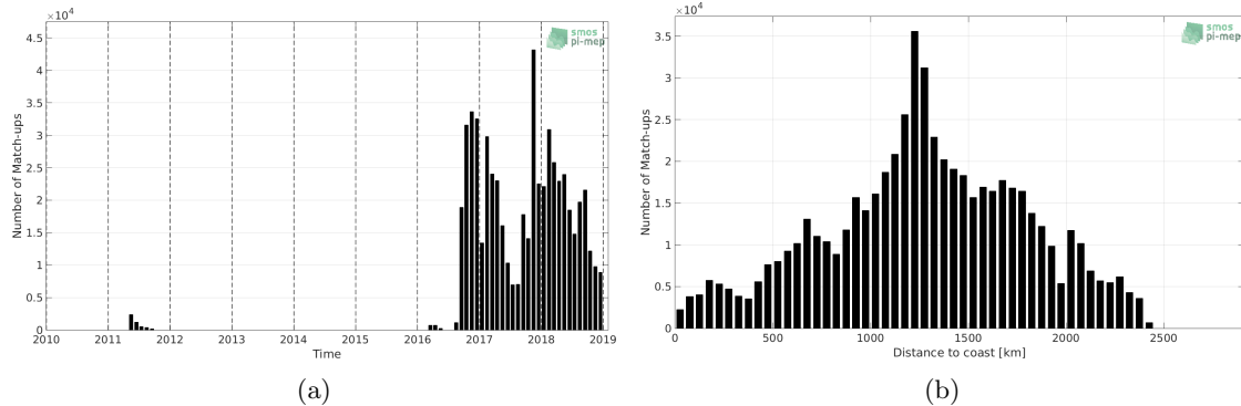
Figure 1: Number of match-ups between Surface drifters and SMOS SSS L3 v7 - 18 Days (CATDS-CECOS-LOCEAN) SSS as a function of time (a) and as function of the distance to coast (b) over the North Pacific Ocean Pi-MEP region and for the full satellite product period.
