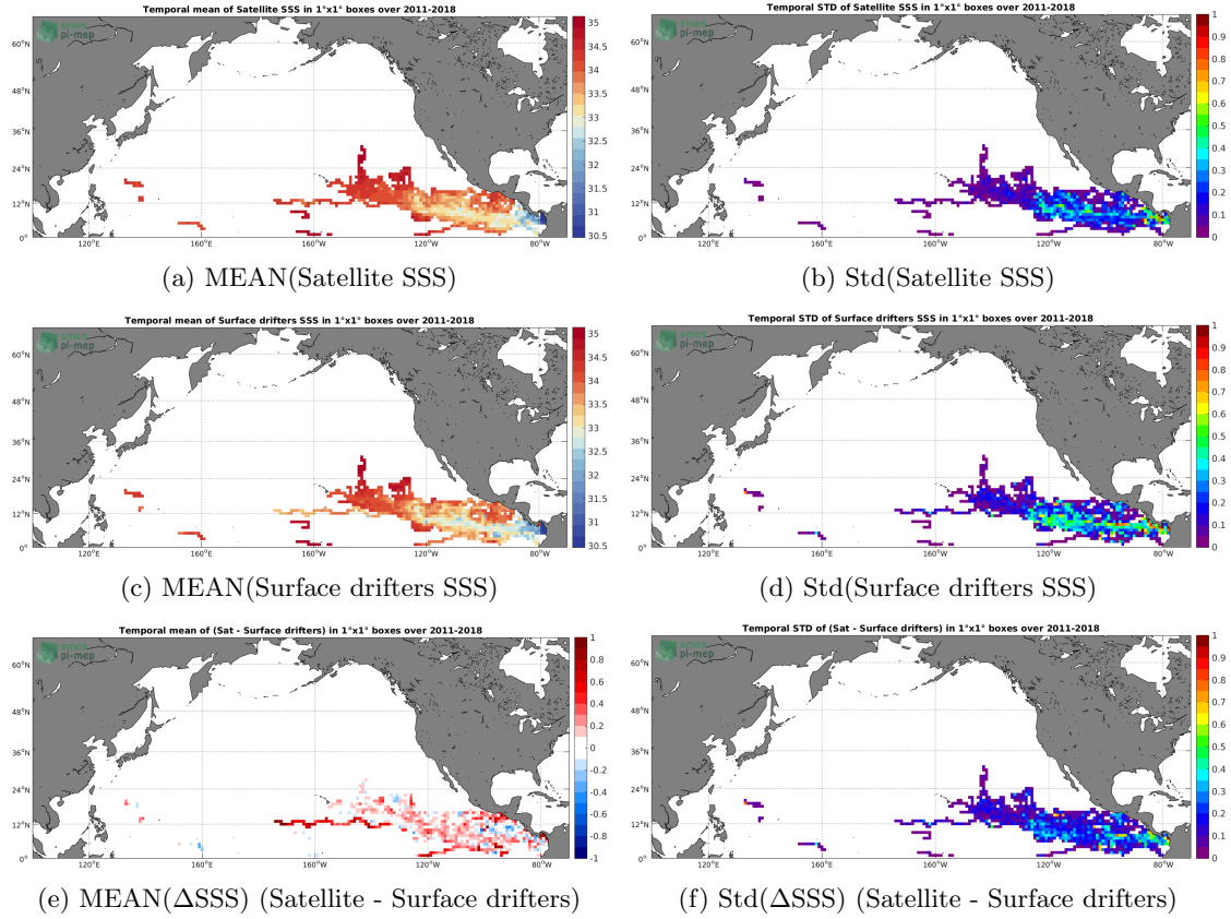
Figure 5: Temporal mean (left) and Std (right) of SSS from SMOS SSS L3 v7 - 18 Days (CATDS-CECOS-LOCEAN) (top), Surface drifters (middle), and of \Delta SSS (Satellite - Surface drifters). Only match-up pairs are used to generate these maps.
