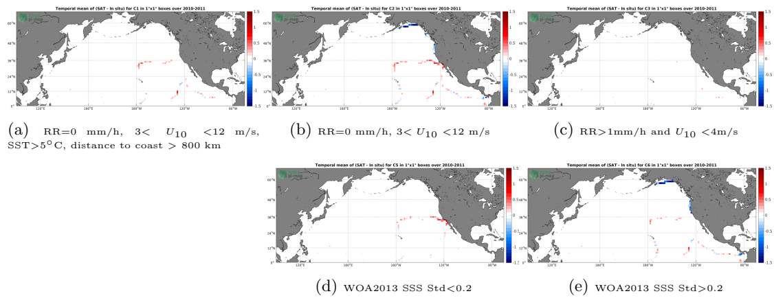
Figure 12: Temporal mean gridded over spatial boxes of size 1^\circ \times 1^\circ of \Delta\text{SSS} (SMOS SSS L3 v5 - 9 Days (CATDS-CECOS-LOCEAN) - TSG (GOSUD-Sailing-ship)) for 5 different subdatasets corresponding to: RR=0 mm/h, 3 < U_{10} < 12 m/s, SST > 5°C, distance to coast > 800 km (a), RR=0 mm/h, 3 < U_{10} < 12 m/s (b), RR > 1mm/h and U_{10} < 4 m/s (c), WOA2013 SSS Std < 0.2 (d), WOA2013 SSS Std > 0.2 (e).
