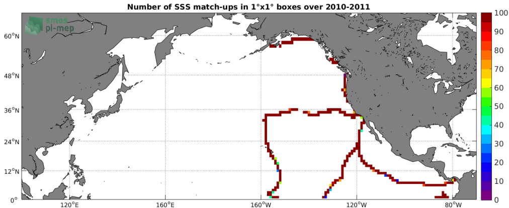
Figure 4: Number of SSS match-ups between TSG (GOSUD-Sailing-ship) SSS and the SMOS SSS L3 v5 - 9 Days (CATDS-CECOS-LOCEAN) SSS product for the North Pacific Ocean Pi-MEP region over 1°x1° boxes and for the full satellite product period.
