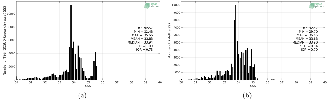
Figure 2: Histograms of SSS from TSG (GOSUD-Research-vessel) (a) and SMOS SSS L3 v5 - 9 Days (CATDS-CECOS-LOCEAN) (b) considering all match-up pairs per bins of 0.1 over the North Pacific Ocean Pi-MEP region and for the full satellite product period.
