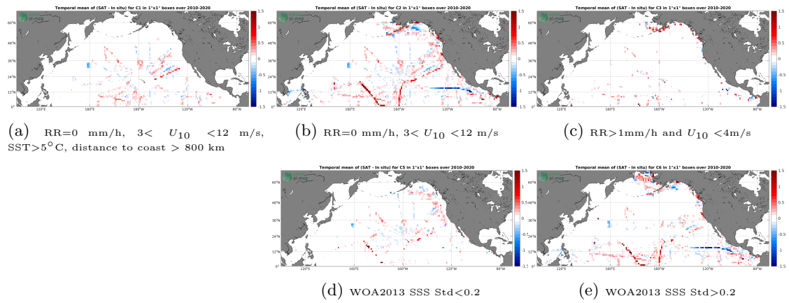
Figure 12: Temporal mean gridded over spatial boxes of size 1°x1° of \Delta SSS (SMOS SSS L3 v5 - 18 Days (CATDS-CECOS-LOCEAN) - TSG (SAMOS)) for 5 different subdatasets corresponding to:RR=0 mm/h, 3 < U_{10} < 12 m/s, SST>5°C, distance to coast > 800 km (a), RR=0 mm/h, 3 < U_{10} < 12 m/s (b), RR>1mm/h and U_{10} < 4 m/s (c), WOA2013 SSS Std<0.2 (d), WOA2013 SSS Std>0.2 (e).
