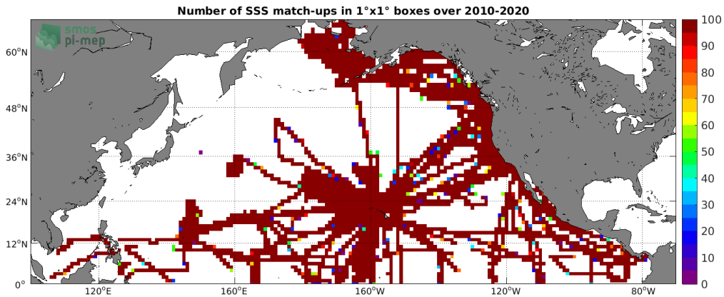
Figure 4: Number of SSS match-ups between TSG (SAMOS) SSS and the SMOS SSS L3 v5 - 18 Days (CATDS-CECOS-LOCEAN) SSS product for the North Pacific Ocean Pi-MEP region over 1°x1° boxes and for the full satellite product period.
