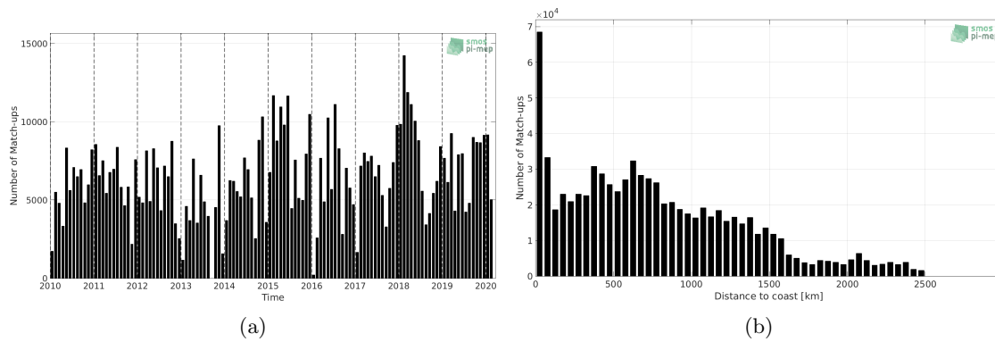
Figure 1: Number of match-ups between TSG (LEGOS-DM) and SMOS SSS L3 v5 - 18 Days (CATDS-CECOS-LOCEAN) SSS as a function of time (a) and as function of the distance to coast (b) over the North Pacific Ocean Pi-MEP region and for the full satellite product period.
