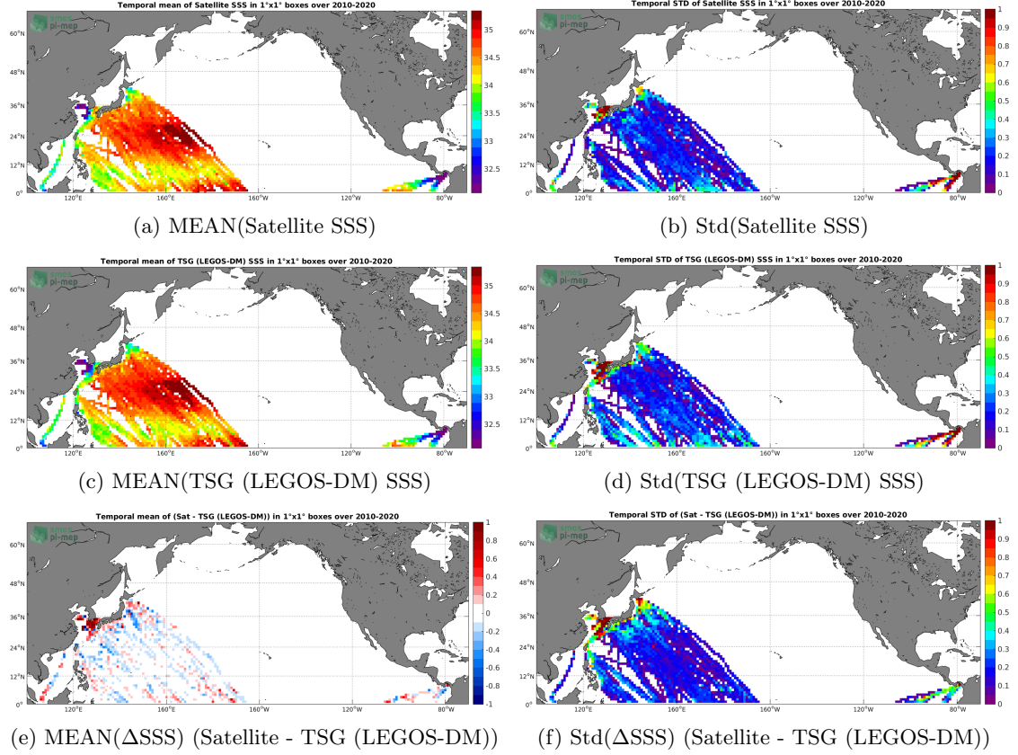
Figure 6: Temporal mean (left) and Std (right) of SSS from SMOS SSS L3 v5 - 18 Days (CATDS-CECOS-LOCEAN) (top), TSG (LEGOS-DM) ( in situ dataset) (middle), and of \Delta\text{SSS} (Satellite - TSG (LEGOS-DM)). Only match-up pairs are used to generate these maps.
