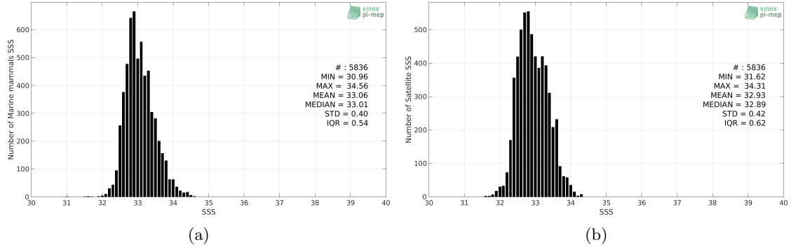
Figure 2: Histograms of SSS from Marine mammals (a) and SMOS SSS L3 v5 - 18 Days (CATDS-CECOS-LOCEAN) (b) considering all match-up pairs per bins of 0.1 over the North Pacific Ocean Pi-MEP region and for the full satellite product period.
