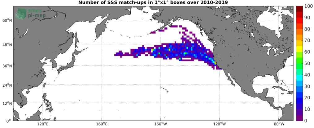
Figure 4: Number of SSS match-ups between Marine mammals SSS and the SMOS SSS L3 v5 - 18 Days (CATDS-CECOS-LOCEAN) SSS product for the North Pacific Ocean Pi-MEP region over 1^\circ \times 1^\circ boxes and for the full satellite product period.
