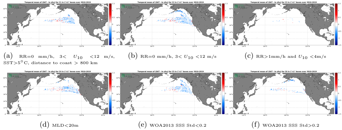
Figure 12: Temporal mean gridded over spatial boxes of size 1^{\circ} \times 1^{\circ} of \Delta\text{SSS} (SMOS SSS L3 v5 - 18 Days (CATDS-CECOS-LOCEAN) - Marine mammals) for 6 different subdatasets corresponding to: RR=0 mm/h, 3 < U_{10} < 12 m/s, SST > 5^{\circ}\text{C} , distance to coast > 800 km (a), RR=0 mm/h, 3 < U_{10} < 12 m/s (b), RR > 1 mm/h and U_{10} < 4 m/s (c), MLD < 20\text{m} (d), WOA2013 SSS Std < 0.2 (e), WOA2013 SSS Std > 0.2 (f).
