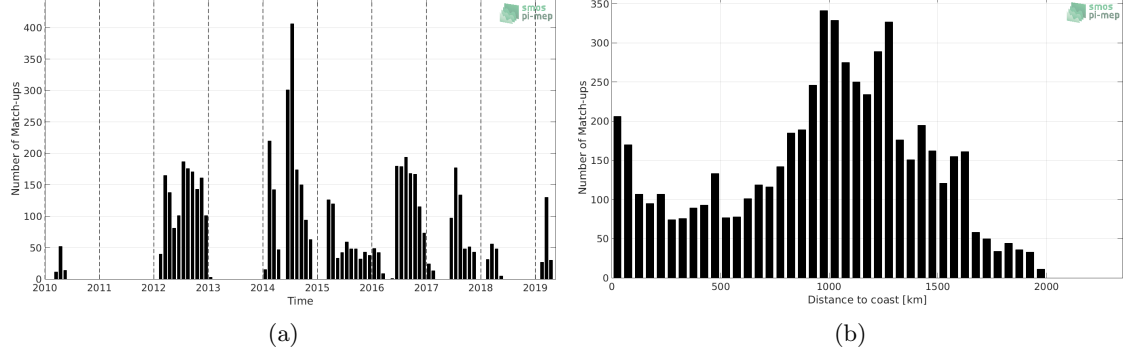
Figure 1: Number of match-ups between Marine mammals and SMOS SSS L3 v5 - 18 Days (CATDS-CECOS-LOCEAN) SSS as a function of time (a) and as function of the distance to coast (b) over the North Pacific Ocean Pi-MEP region and for the full satellite product period.
