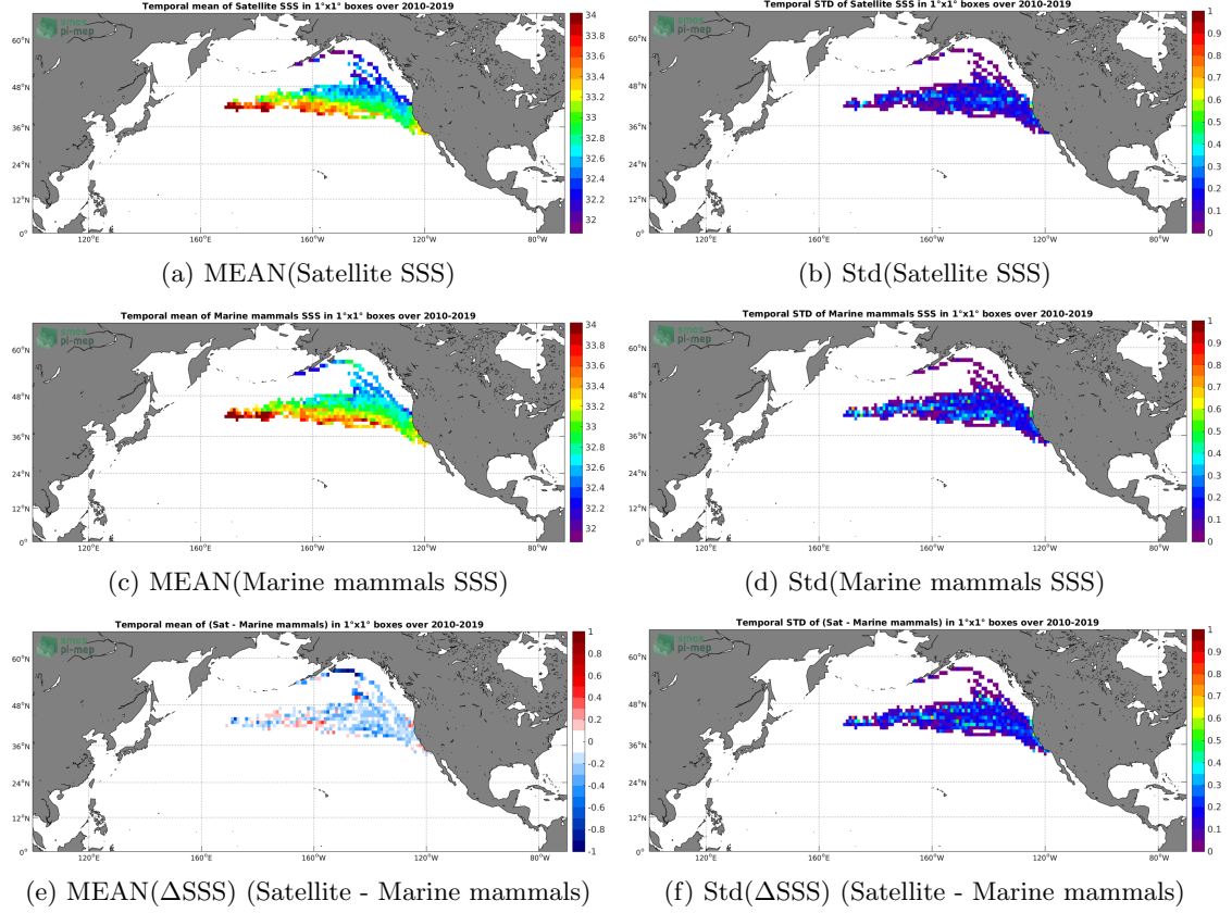
Figure 6: Temporal mean (left) and Std (right) of SSS from SMOS SSS L3 v5 - 18 Days (CATDS-CECOS-LOCEAN) (top), Marine mammals (middle), and of \Delta\text{SSS} (Satellite - Marine mammals). Only match-up pairs are used to generate these maps.
