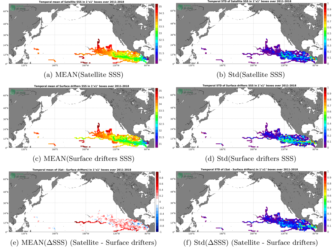
Figure 5: Temporal mean (left) and Std (right) of SSS from SMOS SSS L3 v5 - 18 Days (CATDS-CECOS-LOCEAN) (top), Surface drifters (middle), and of \Delta SSS (Satellite - Surface drifters). Only match-up pairs are used to generate these maps.
