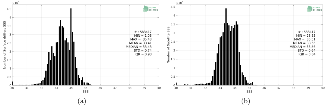
Figure 2: Histograms of SSS from Surface drifters (a) and SMOS SSS L3 v5 - 18 Days (CATDS-CECOS-LOCEAN) (b) considering all match-up pairs per bins of 0.1 over the North Pacific Ocean Pi-MEP region and for the full satellite product period.
