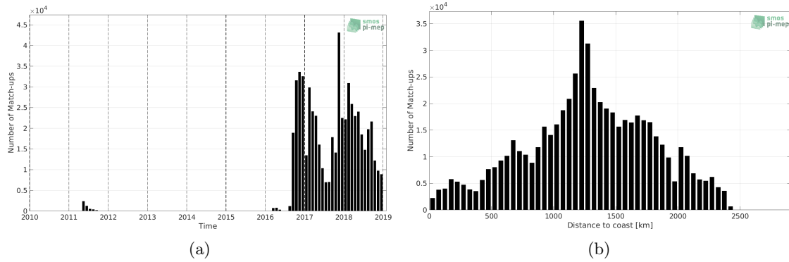
Figure 1: Number of match-ups between Surface drifters and SMOS SSS L3 v5 - 18 Days (CATDS-CECOS-LOCEAN) SSS as a function of time (a) and as function of the distance to coast (b) over the North Pacific Ocean Pi-MEP region and for the full satellite product period.
