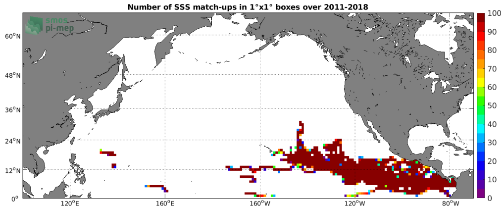
Figure 3: Number of SSS match-ups between Surface drifters SSS and the SMOS SSS L3 v5 - 18 Days (CATDS-CECOS-LOCEAN) SSS product for the North Pacific Ocean Pi-MEP region over 1^\circ \times 1^\circ boxes and for the full satellite product period.
