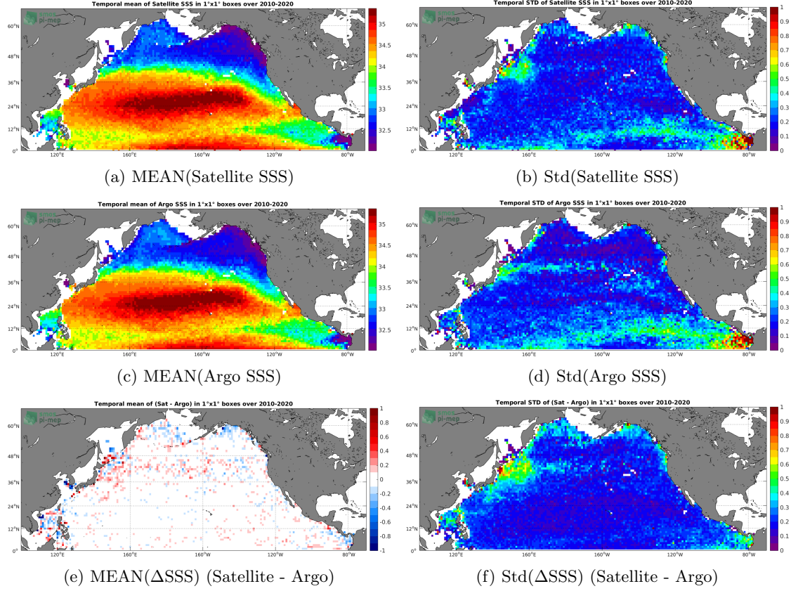
Figure 6: Temporal mean (left) and Std (right) of SSS from SMOS SSS L3 v5 - 18 Days (CATDS-CECOS-LOCEAN) (top), Argo (middle), and of \Delta\text{SSS} (Satellite - Argo). Only match-up pairs are used to generate these maps.
