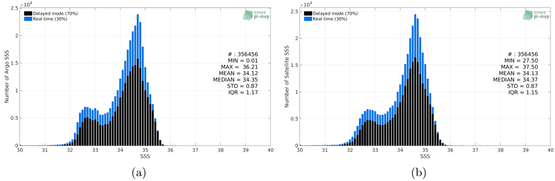
Figure 2: Histograms of SSS from Argo (a) and SMOS SSS L3 v5 - 18 Days (CATDS-CECOS-LOCEAN) (b) considering all match-up pairs per bins of 0.1 over the North Pacific Ocean Pi-MEP region and for the full satellite product period.
