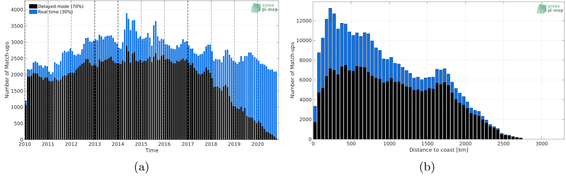
Figure 1: Number of match-ups between Argo and SMOS SSS L3 v5 - 18 Days (CATDS-CECOS-LOCEAN) SSS as a function of time (a) and as function of the distance to coast (b) over the North Pacific Ocean Pi-MEP region and for the full satellite product period.
