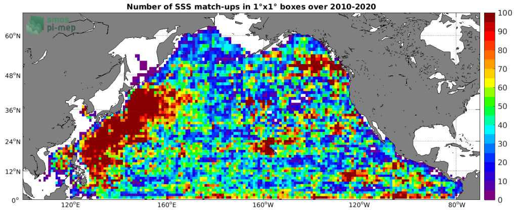
Figure 4: Number of SSS match-ups between Argo SSS and the SMOS SSS L3 v5 - 18 Days (CATDS-CECOS-LOCEAN) SSS product for the North Pacific Ocean Pi-MEP region over 1^\circ \times 1^\circ boxes and for the full satellite product period.
