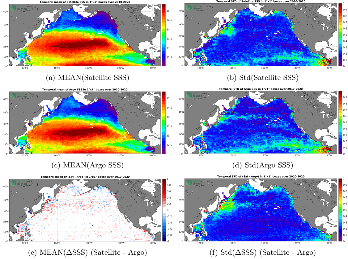
Figure 6: Temporal mean (left) and Std (right) of SSS from SMOS SSS L3 v5 - 18 Days (CATDS-CECOS-LOCEAN) (top), Argo (middle), and of \Delta SSS (Satellite - Argo). Only match-up pairs are used to generate these maps.
