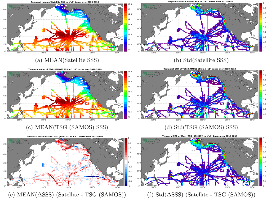
Figure 6: Temporal mean (left) and Std (right) of SSS from SMOS SSS L3 v4 - 18 Days (CATDS-CECOS-LOCEAN) (top), TSG (SAMOS) (middle), and of \Delta SSS (Satellite - TSG (SAMOS)). Only match-up pairs are used to generate these maps.
