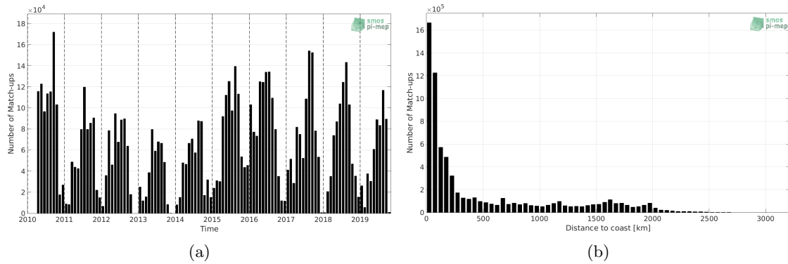
Figure 1: Number of match-ups between TSG (SAMOS) and SMOS SSS L3 v4 - 18 Days (CATDS-CECOS-LOCEAN) SSS as a function of time (a) and as function of the distance to coast (b) over the North Pacific Ocean Pi-MEP region and for the full satellite product period.
