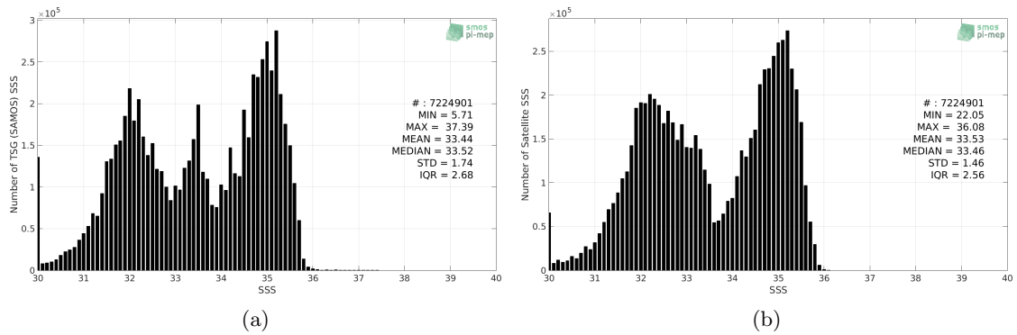
Figure 2: Histograms of SSS from TSG (SAMOS) (a) and SMOS SSS L3 v4 - 18 Days (CATDS-CECOS-LOCEAN) (b) considering all match-up pairs per bins of 0.1 over the North Pacific Ocean Pi-MEP region and for the full satellite product period.
