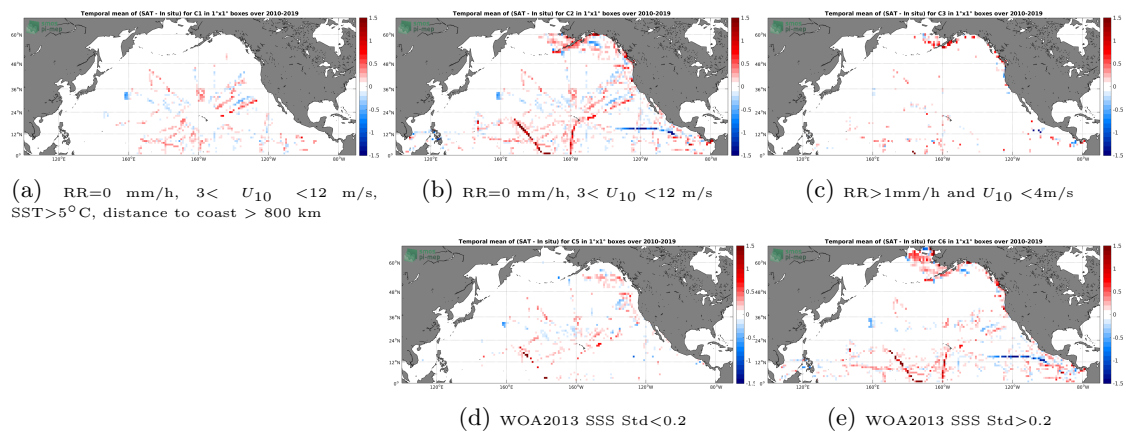
Figure 12: Temporal mean gridded over spatial boxes of size 1^\circ \times 1^\circ of \Delta\text{SSS} (SMOS SSS L3 v4 - 18 Days (CATDS-CECOS-LOCEAN) - TSG (SAMOS)) for 5 different subdatasets corresponding to:RR=0 mm/h, 3 < U_{10} < 12 m/s, SST >5^\circ\text{C} , distance to coast > 800 km (a), RR=0 mm/h, 3 < U_{10} < 12 m/s (b), RR >1 mm/h and U_{10} < 4 m/s (c), WOA2013 SSS Std <0.2 (d), WOA2013 SSS Std >0.2 (e).
