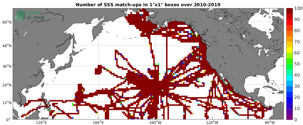
Figure 4: Number of SSS match-ups between TSG (SAMOS) SSS and the SMOS SSS L3 v4 - 18 Days (CATDS-CECOS-LOCEAN) SSS product for the North Pacific Ocean Pi-MEP region over 1°x1° boxes and for the full satellite product period.
