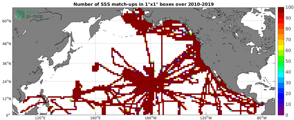
Figure 4: Number of SSS match-ups between TSG-SAMOS SSS and the SMOS-L3-CATDS-CECOS-LOCEAN-V4-18DAYS-25KM SSS product for the North Pacific Ocean Pi-MEP region over 1°x1° boxes and for the full satellite product period.
