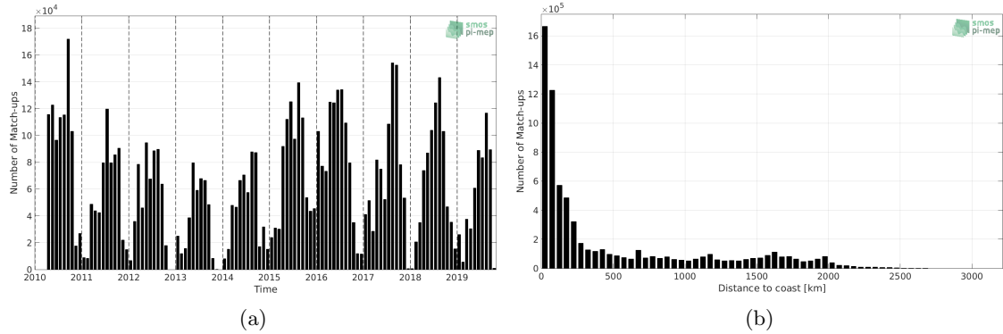
Figure 1: Number of match-ups between TSG-SAMOS and SMOS-L3-CATDS-CECOS-LOCEAN-V4-18DAYS-25KM SSS as a function of time (a) and as function of the distance to coast (b) over the North Pacific Ocean Pi-MEP region and for the full satellite product period.
