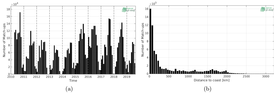
Figure 1: Number of match-ups between TSG-SAMOS and SMOS-L3-CATDS-CECOS-LOCEAN-V4-18DAYS-25KM SSS as a function of time (a) and as function of the distance to coast (b) over the North Pacific Ocean Pi-MEP region and for the full satellite product period.
