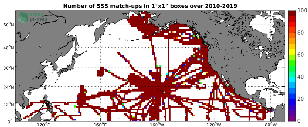
Figure 4: Number of SSS match-ups between TSG-SAMOS SSS and the SMOS-L3-CATDS-CECOS-LOCEAN-V4-18DAYS-25KM SSS product for the North Pacific Ocean Pi-MEP region over 1^\circ \times 1^\circ boxes and for the full satellite product period.
