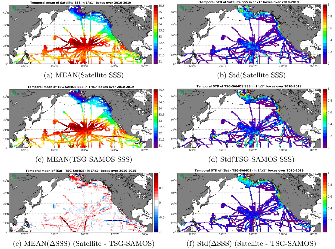
Figure 6: Temporal mean (left) and Std (right) of SSS from SMOS-L3-CATDS-CECOS-LOCEAN-V4-18DAYS-25KM (top), TSG-SAMOS (middle), and of \Delta SSS (Satellite - TSG-SAMOS). Only match-up pairs are used to generate these maps.
