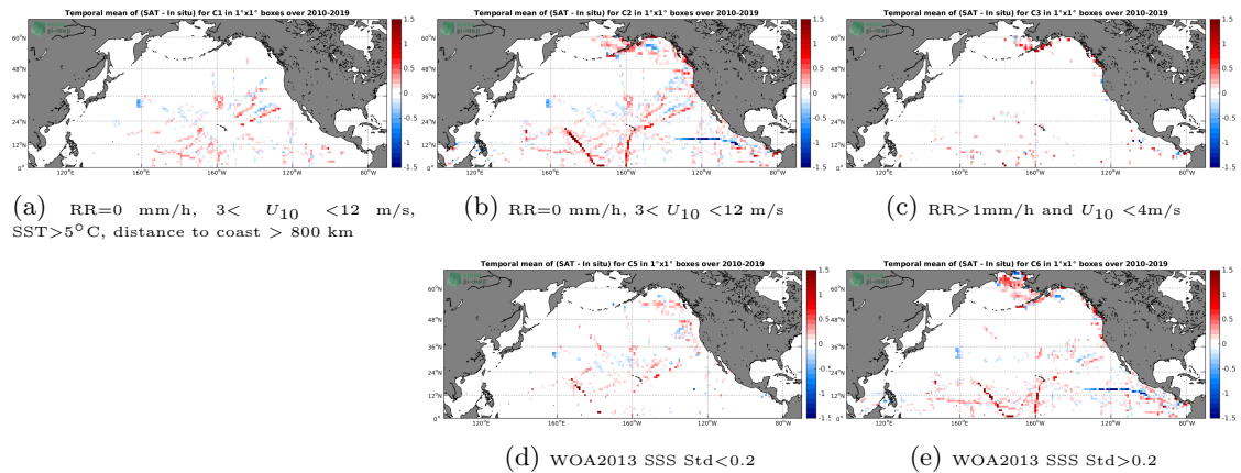
Figure 12: Temporal mean gridded over spatial boxes of size 1^\circ \times 1^\circ of \Delta SSS (SMOS-L3-CATDS-CECOS-LOCEAN-V4-18DAYS-25KM - TSG-SAMOS) for 5 different subdatasets corresponding to:RR=0 mm/h, 3 < U_{10} < 12 m/s, SST >5^\circ C, distance to coast > 800 km (a), RR=0 mm/h, 3 < U_{10} < 12 m/s (b), RR >1 mm/h and U_{10} < 4 m/s (c), WOA2013 SSS Std <0.2 (d), WOA2013 SSS Std >0.2 (e).
