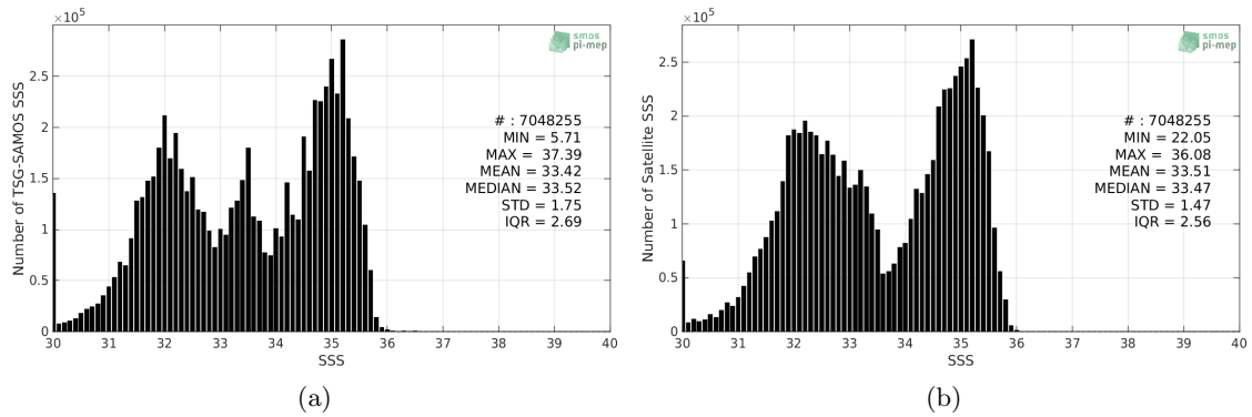
Figure 2: Histograms of SSS from TSG-SAMOS (a) and SMOS-L3-CATDS-CECOS-LOCEAN-V4-18DAYS-25KM (b) considering all match-up pairs per bins of 0.1 over the North Pacific Ocean Pi-MEP region and for the full satellite product period.
