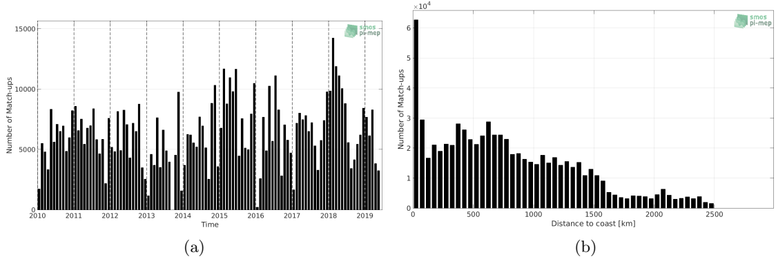
Figure 1: Number of match-ups between TSG (LEGOS-DM) and SMOS SSS L3 v4 - 18 Days (CATDS-CECOS-LOCEAN) SSS as a function of time (a) and as function of the distance to coast (b) over the North Pacific Ocean Pi-MEP region and for the full satellite product period.
