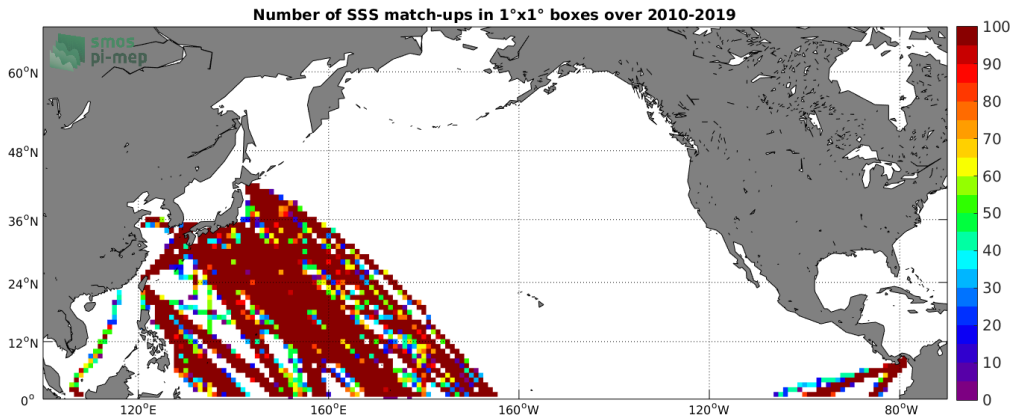
Figure 4: Number of SSS match-ups between TSG (LEGOS-DM) SSS and the SMOS SSS L3 v4 - 18 Days (CATDS-CECOS-LOCEAN) SSS product for the North Pacific Ocean Pi-MEP region over 1^\circ \times 1^\circ boxes and for the full satellite product period.
