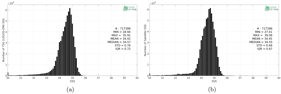
Figure 2: Histograms of SSS from TSG (LEGOS-DM) (a) and SMOS SSS L3 v4 - 18 Days (CATDS-CECOS-LOCEAN) (b) considering all match-up pairs per bins of 0.1 over the North Pacific Ocean Pi-MEP region and for the full satellite product period.
