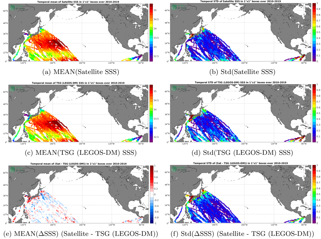
Figure 6: Temporal mean (left) and Std (right) of SSS from SMOS SSS L3 v4 - 18 Days (CATDS-CECOS-LOCEAN) (top), TSG (LEGOS-DM) (middle), and of \Delta SSS (Satellite - TSG (LEGOS-DM)). Only match-up pairs are used to generate these maps.
