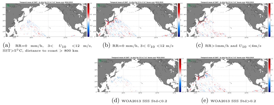
Figure 12: Temporal mean gridded over spatial boxes of size 1^\circ \times 1^\circ of \Delta SSS (SMOS SSS L3 v4 - 18 Days (CATDS-CECOS-LOCEAN) - TSG (LEGOS-DM)) for 5 different subdatasets corresponding to: RR=0 mm/h, 3 < U_{10} < 12 m/s, SST >5^\circ\text{C} , distance to coast > 800 km (a), RR=0 mm/h, 3 < U_{10} < 12 m/s (b), RR >1 mm/h and U_{10} < 4 m/s (c), WOA2013 SSS Std <0.2 (d), WOA2013 SSS Std >0.2 (e).
