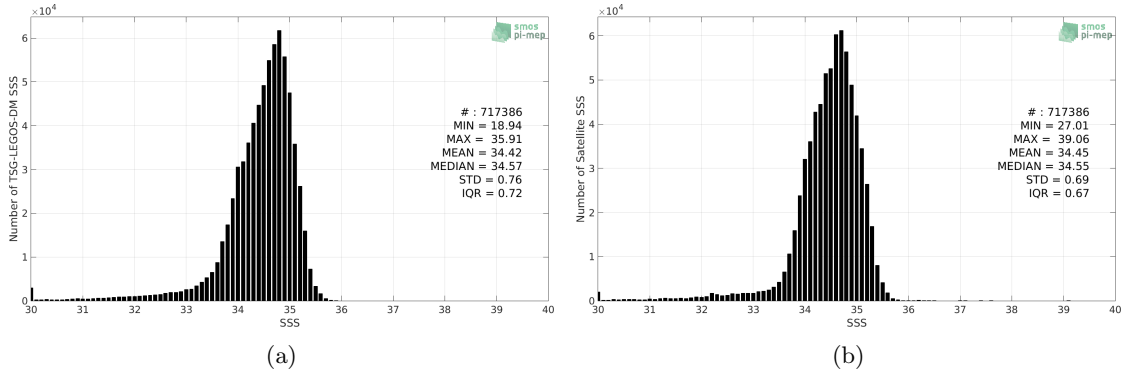
Figure 2: Histograms of SSS from TSG-LEGOS-DM (a) and SMOS-L3-CATDS-CECOS-LOCEAN-V4-18DAYS-25KM (b) considering all match-up pairs per bins of 0.1 over the North Pacific Ocean Pi-MEP region and for the full satellite product period.
