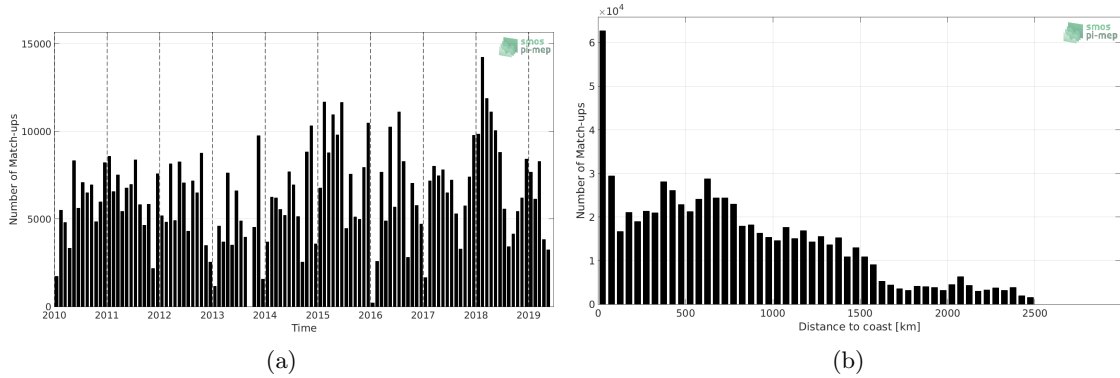
Figure 1: Number of match-ups between TSG-LEGOS-DM and SMOS-L3-CATDS-CECOS-LOCEAN-V4-18DAYS-25KM SSS as a function of time (a) and as function of the distance to coast (b) over the North Pacific Ocean Pi-MEP region and for the full satellite product period.
