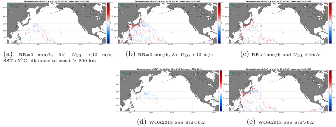
Figure 12: Temporal mean gridded over spatial boxes of size 1^\circ \times 1^\circ of \Delta SSS (SMOS-L3-CATDS-CECOS-LOCEAN-V4-18DAYS-25KM - TSG-LEGOS-DM) for 5 different subdatasets corresponding to: RR=0 mm/h, 3 < U_{10} < 12 m/s, SST > 5^\circ\text{C} , distance to coast > 800 km (a), RR=0 mm/h, 3 < U_{10} < 12 m/s (b), RR > 1 mm/h and U_{10} < 4 m/s (c), WOA2013 SSS Std < 0.2 (d), WOA2013 SSS Std > 0.2 (e).
