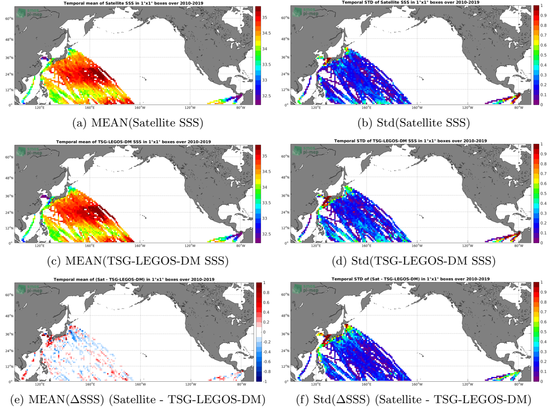
Figure 6: Temporal mean (left) and Std (right) of SSS from SMOS-L3-CATDS-CECOS-LOCEAN-V4-18DAYS-25KM (top), TSG-LEGOS-DM (middle), and of \Delta SSS (Satellite - TSG-LEGOS-DM). Only match-up pairs are used to generate these maps.
