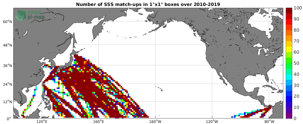
Figure 4: Number of SSS match-ups between TSG-LEGOS-DM SSS and the SMOS-L3-CATDS-CECOS-LOCEAN-V4-18DAYS-25KM SSS product for the North Pacific Ocean Pi-MEP region over 1°x1° boxes and for the full satellite product period.
