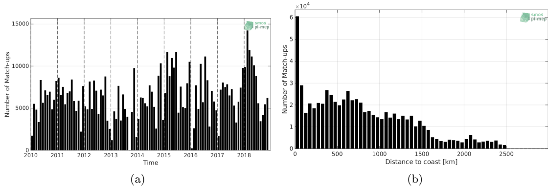
Figure 1: Number of match-ups between TSG-LEGOS-DM and SMOS-L3-CATDS-CECOS-LOCEAN-V4-18DAYS-25KM SSS as a function of time (a) and as function of the distance to coast (b) over the North Pacific Ocean Pi-MEP region and for the full satellite product period.
