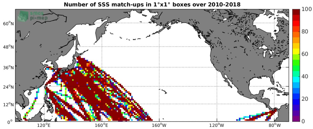
Figure 4: Number of SSS match-ups between TSG-LEGOS-DM SSS and the SMOS-L3-CATDS-CECOS-LOCEAN-V4-18DAYS-25KM SSS product for the North Pacific Ocean Pi-MEP region over 1^\circ \times 1^\circ boxes and for the full satellite product period.
