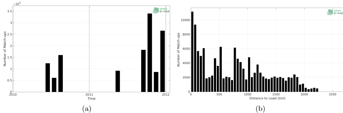
Figure 1: Number of match-ups between TSG (GOSUD-Sailing-ship) and SMOS SSS L3 v4 - 18 Days (CATDS-CECOS-LOCEAN) SSS as a function of time (a) and as function of the distance to coast (b) over the North Pacific Ocean Pi-MEP region and for the full satellite product period.
