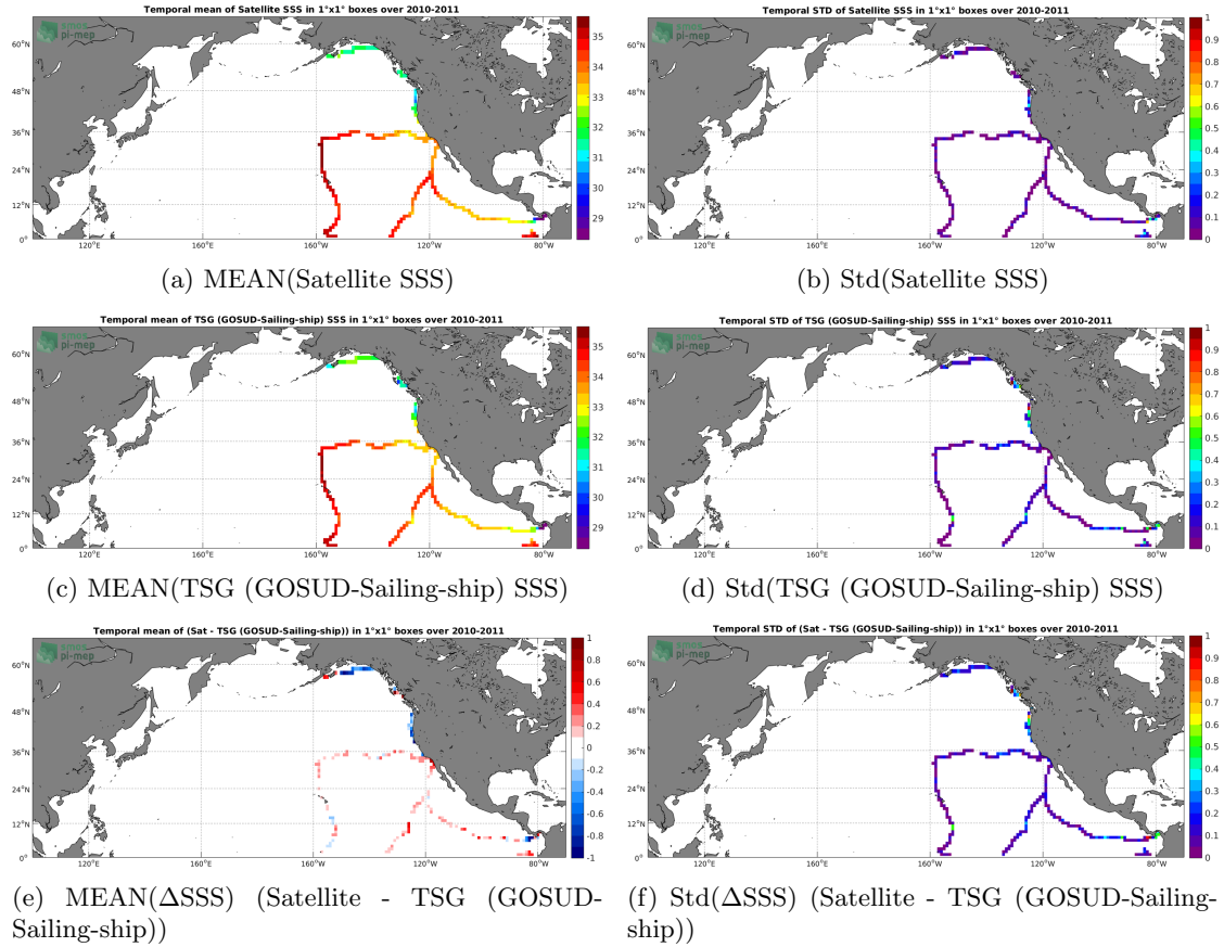
Figure 6: Temporal mean (left) and Std (right) of SSS from SMOS SSS L3 v4 - 18 Days (CATDS-CECOS-LOCEAN) (top), TSG (GOSUD-Sailing-ship) (middle), and of \Delta SSS (Satellite - TSG (GOSUD-Sailing-ship)). Only match-up pairs are used to generate these maps.
