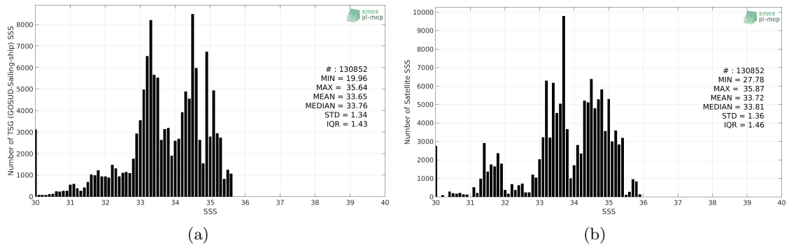
Figure 2: Histograms of SSS from TSG (GOSUD-Sailing-ship) (a) and SMOS SSS L3 v4 - 18 Days (CATDS-CECOS-LOCEAN) (b) considering all match-up pairs per bins of 0.1 over the North Pacific Ocean Pi-MEP region and for the full satellite product period.
