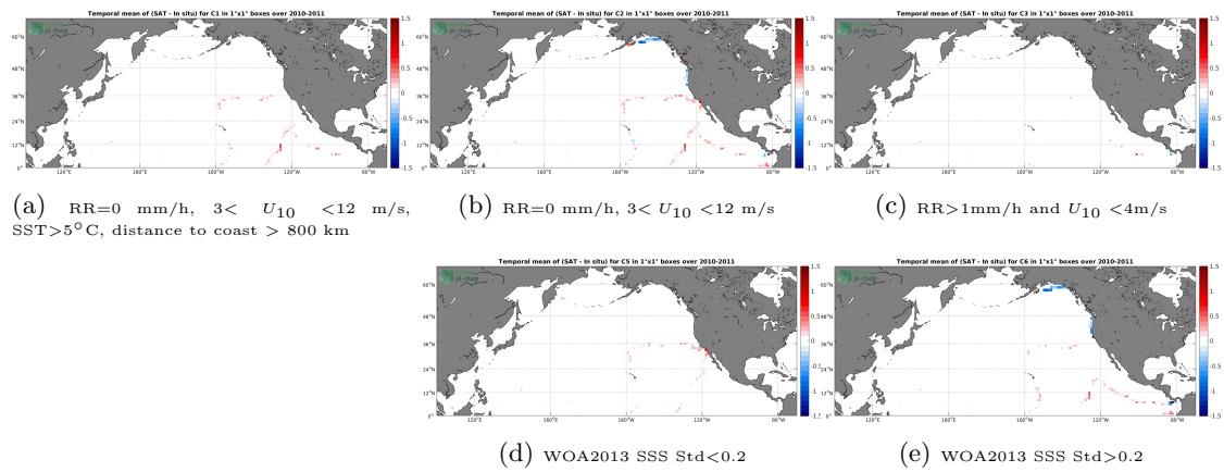
Figure 12: Temporal mean gridded over spatial boxes of size 1^\circ \times 1^\circ of \Delta SSS (SMOS SSS L3 v4 - 18 Days (CATDS-CECOS-LOCEAN) - TSG (GOSUD-Sailing-ship)) for 5 different subdatasets corresponding to: RR=0 mm/h, 3 < U_{10} < 12 m/s, SST > 5°C, distance to coast > 800 km (a), RR=0 mm/h, 3 < U_{10} < 12 m/s (b), RR > 1mm/h and U_{10} < 4 m/s (c), WOA2013 SSS Std < 0.2 (d), WOA2013 SSS Std > 0.2 (e).
