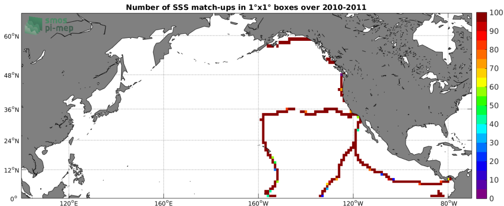
Figure 4: Number of SSS match-ups between TSG-GOSUD-Sailing-ship SSS and the SMOS-L3-CATDS-CECOS-LOCEAN-V4-18DAYS-25KM SSS product for the North Pacific Ocean Pi-MEP region over 1°x1° boxes and for the full satellite product period.
