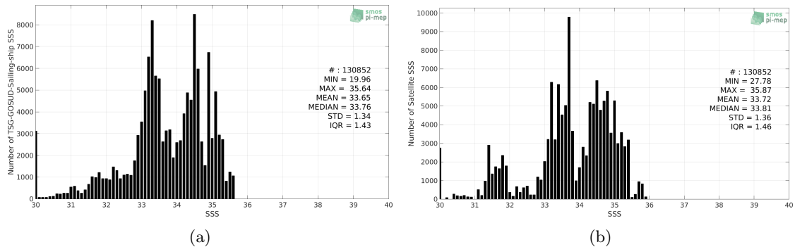
Figure 2: Histograms of SSS from TSG-GOSUD-Sailing-ship (a) and SMOS-L3-CATDS-CECOS-LOCEAN-V4-18DAYS-25KM (b) considering all match-up pairs per bins of 0.1 over the North Pacific Ocean Pi-MEP region and for the full satellite product period.
