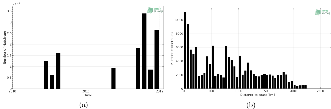
Figure 1: Number of match-ups between TSG-GOSUD-Sailing-ship and SMOS-L3-CATDS-CECOS-LOCEAN-V4-18DAYS-25KM SSS as a function of time (a) and as function of the distance to coast (b) over the North Pacific Ocean Pi-MEP region and for the full satellite product period.
