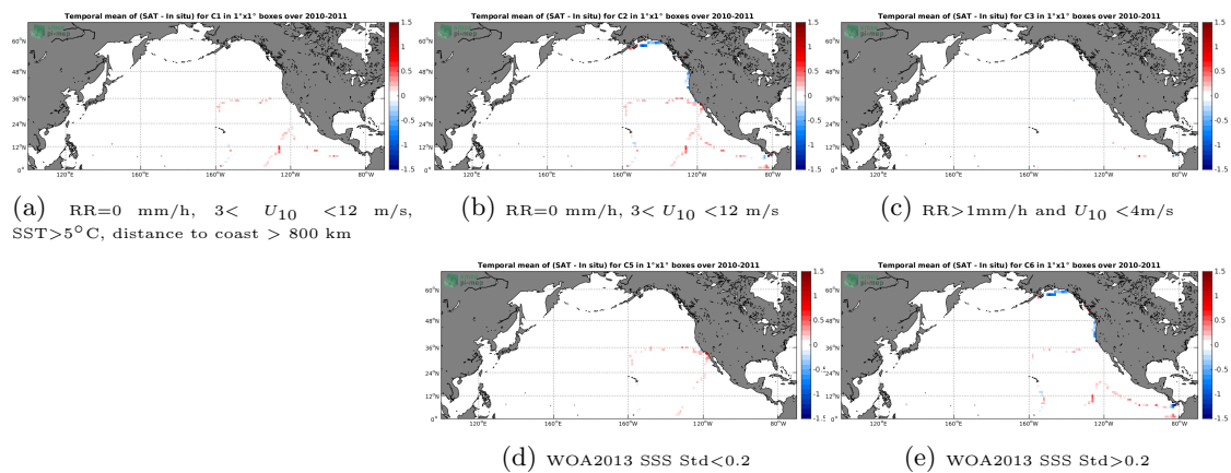
Figure 12: Temporal mean gridded over spatial boxes of size 1^\circ \times 1^\circ of \Delta\text{SSS} (SMOS-L3-CATDS-CECOS-LOCEAN-V4-18DAYS-25KM - TSG-GOSUD-Sailing-ship) for 5 different subdatasets corresponding to: RR=0 mm/h, 3 < U_{10} < 12 m/s, SST > 5°C, distance to coast > 800 km (a), RR=0 mm/h, 3 < U_{10} < 12 m/s (b), RR > 1mm/h and U_{10} < 4 m/s (c), WOA2013 SSS Std < 0.2 (d), WOA2013 SSS Std > 0.2 (e).
