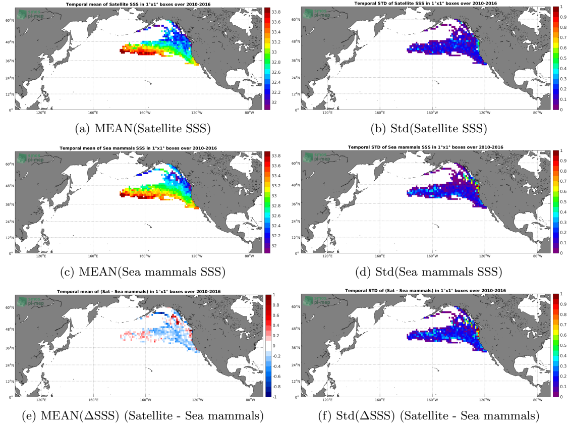
Figure 6: Temporal mean (left) and Std (right) of SSS from SMOS SSS L3 v4 - 18 Days (CATDS-CECOS-LOCEAN) (top), Sea mammals (middle), and of \Delta SSS (Satellite - Sea mammals). Only match-up pairs are used to generate these maps.
