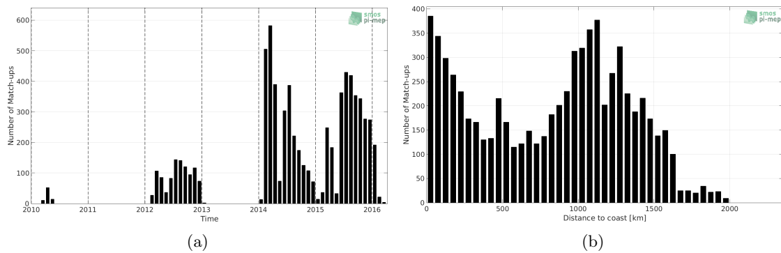
Figure 1: Number of match-ups between Sea mammals and SMOS SSS L3 v4 - 18 Days (CATDS-CECOS-LOCEAN) SSS as a function of time (a) and as function of the distance to coast (b) over the North Pacific Ocean Pi-MEP region and for the full satellite product period.
