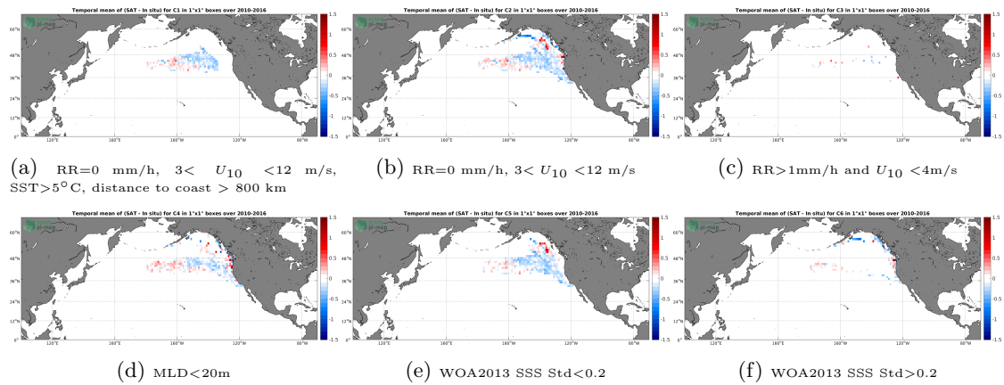
Figure 12: Temporal mean gridded over spatial boxes of size 1^\circ \times 1^\circ of \Delta SSS (SMOS SSS L3 v4 - 18 Days (CATDS-CECOS-LOCEAN) - Sea mammals) for 6 different subdatasets corresponding to:RR=0 mm/h, 3 < U_{10} < 12 m/s, SST >5^\circ C, distance to coast > 800 km (a), RR=0 mm/h, 3 < U_{10} < 12 m/s (b), RR >1 mm/h and U_{10} < 4 m/s (c),MLD <20 m (d),WOA2013 SSS Std <0.2 (e),WOA2013 SSS Std >0.2 (f).
