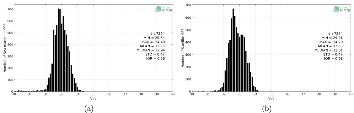
Figure 2: Histograms of SSS from Sea mammals (a) and SMOS SSS L3 v4 - 18 Days (CATDS-CECOS-LOCEAN) (b) considering all match-up pairs per bins of 0.1 over the North Pacific Ocean Pi-MEP region and for the full satellite product period.
