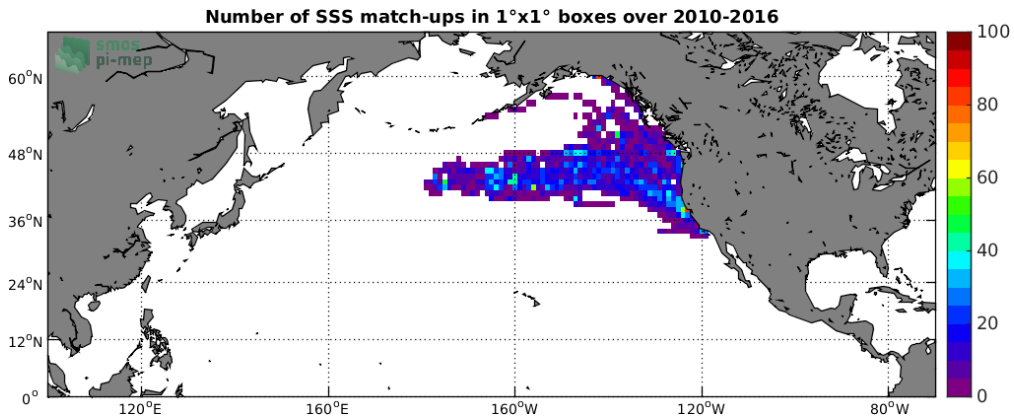
Figure 4: Number of SSS match-ups between Sea mammals SSS and the SMOS-L3-CATDS-CECOS-LOCEAN-V4-18DAYS-25KM SSS product for the North Pacific Ocean Pi-MEP region over 1°x1° boxes and for the full satellite product period.
