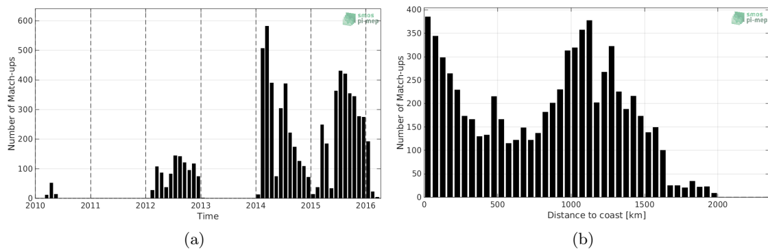
Figure 1: Number of match-ups between Sea mammals and SMOS-L3-CATDS-CECOS-LOCEAN-V4-18DAYS-25KM SSS as a function of time (a) and as function of the distance to coast (b) over the North Pacific Ocean Pi-MEP region and for the full satellite product period.
