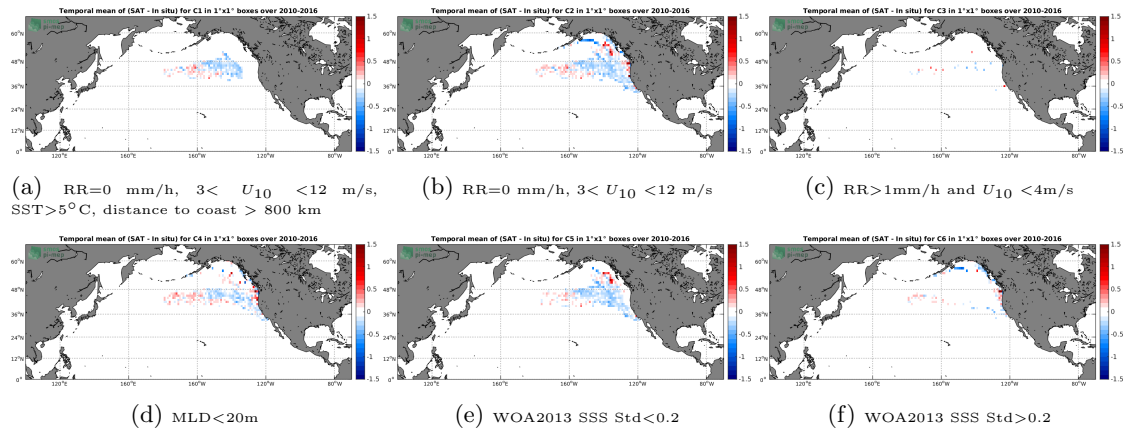
Figure 12: Temporal mean gridded over spatial boxes of size 1^\circ \times 1^\circ of \Delta SSS (SMOS-L3-CATDS-CECOS-LOCEAN-V4-18DAYS-25KM - Sea mammals) for 6 different subdatasets corresponding to:RR=0 mm/h, 3 < U_{10} < 12 m/s, SST>5°C, distance to coast > 800 km (a), RR=0 mm/h, 3 < U_{10} < 12 m/s (b), RR>1mm/h and U_{10} < 4 m/s (c),MLD<20m (d),WOA2013 SSS Std<0.2 (e),WOA2013 SSS Std>0.2 (f).
