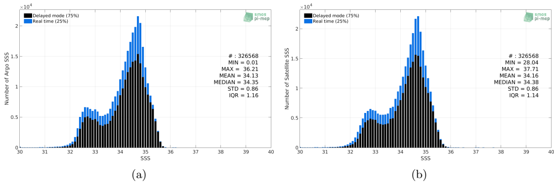
Figure 2: Histograms of SSS from Argo (a) and SMOS SSS L3 v4 - 18 Days (CATDS-CECOS-LOCEAN) (b) considering all match-up pairs per bins of 0.1 over the North Pacific Ocean Pi-MEP region and for the full satellite product period.
