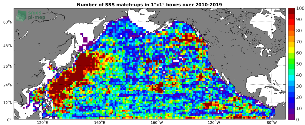
Figure 4: Number of SSS match-ups between Argo SSS and the SMOS SSS L3 v4 - 18 Days (CATDS-CECOS-LOCEAN) SSS product for the North Pacific Ocean Pi-MEP region over 1^\circ \times 1^\circ boxes and for the full satellite product period.
