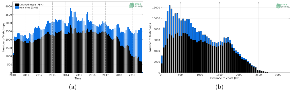
Figure 1: Number of match-ups between Argo and SMOS SSS L3 v4 - 18 Days (CATDS-CECOS-LOCEAN) SSS as a function of time (a) and as function of the distance to coast (b) over the North Pacific Ocean Pi-MEP region and for the full satellite product period.
