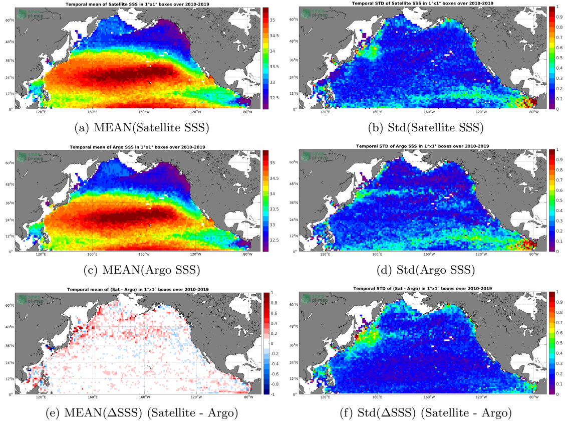
Figure 6: Temporal mean (left) and Std (right) of SSS from SMOS SSS L3 v4 - 18 Days (CATDS-CECOS-LOCEAN) (top), Argo (middle), and of \Delta SSS (Satellite - Argo). Only match-up pairs are used to generate these maps.
