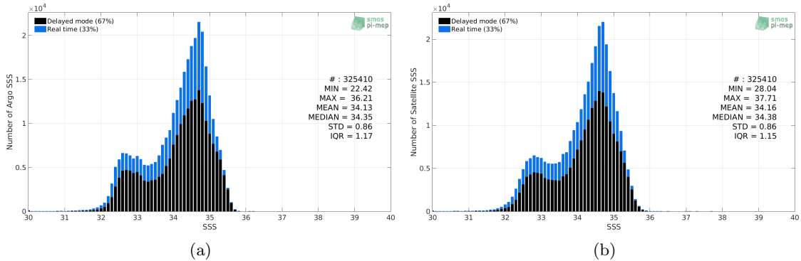
Figure 2: Histograms of SSS from Argo (a) and SMOS-L3-CATDS-CECOS-LOCEAN-V4-18DAYS-25KM (b) considering all match-up pairs per bins of 0.1 over the North Pacific Ocean Pi-MEP region and for the full satellite product period.
