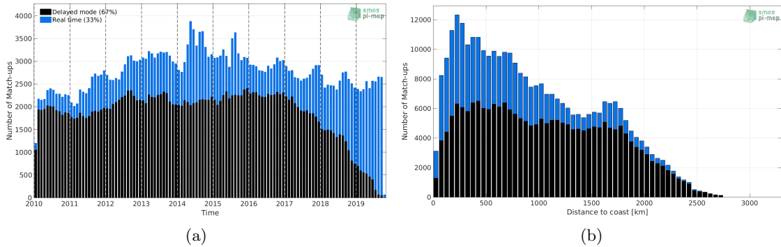
Figure 1: Number of match-ups between Argo and SMOS-L3-CATDS-CECOS-LOCEAN-V4-18DAYS-25KM SSS as a function of time (a) and as function of the distance to coast (b) over the North Pacific Ocean Pi-MEP region and for the full satellite product period.
