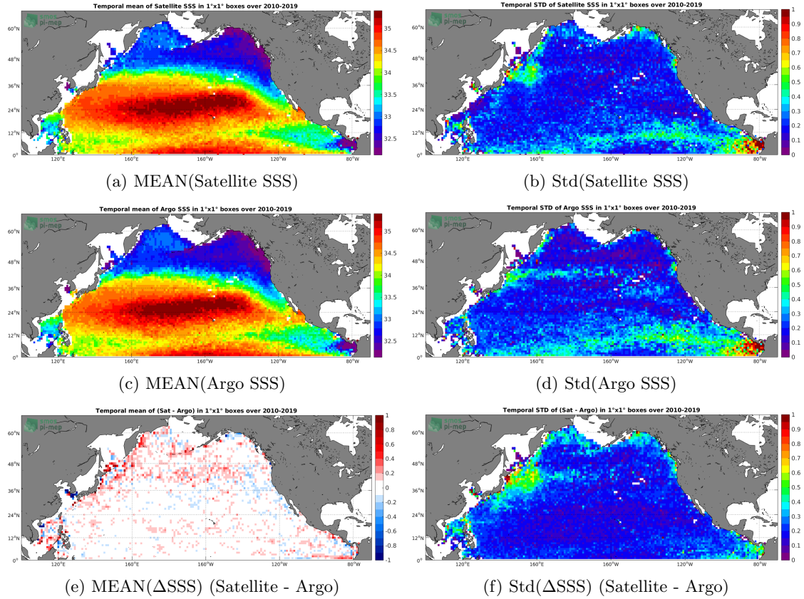
Figure 6: Temporal mean (left) and Std (right) of SSS from SMOS-L3-CATDS-CECOS-LOCEAN-V4-18DAYS-25KM (top), Argo (middle), and of \Delta SSS (Satellite - Argo). Only match-up pairs are used to generate these maps.
