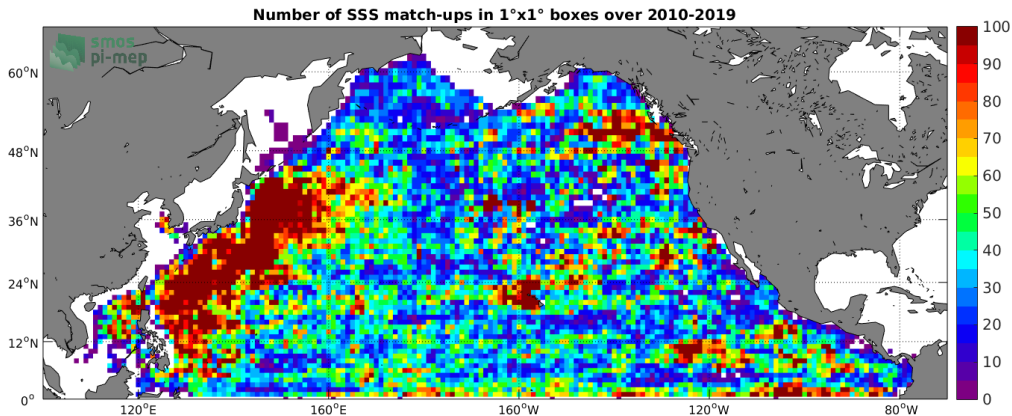
Figure 4: Number of SSS match-ups between Argo SSS and the SMOS-L3-CATDS-CECOS-LOCEAN-V4-18DAYS-25KM SSS product for the North Pacific Ocean Pi-MEP region over 1^\circ \times 1^\circ boxes and for the full satellite product period.
