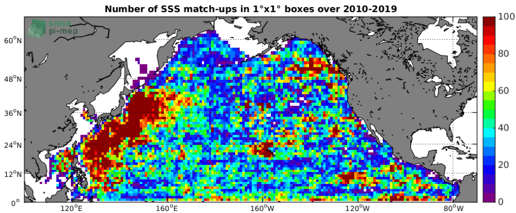
Figure 4: Number of SSS match-ups between Argo SSS and the SMOS-L3-CATDS-CECOS-LOCEAN-V4-18DAYS-25KM SSS product for the North Pacific Ocean Pi-MEP region over 1°x1° boxes and for the full satellite product period.
