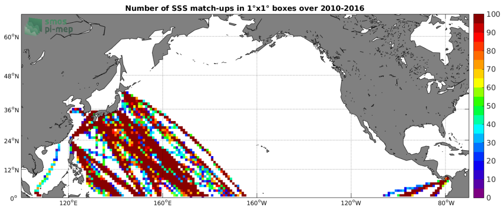
Figure 4: Number of SSS match-ups between TSG-LEGOS-DM SSS and the SMOS-L3-CATDS-CECOS-LOCEAN-V3-9DAYS-25KM SSS product for the North Pacific Ocean Pi-MEP region over 1^\circ \times 1^\circ boxes and for the full satellite product period.
