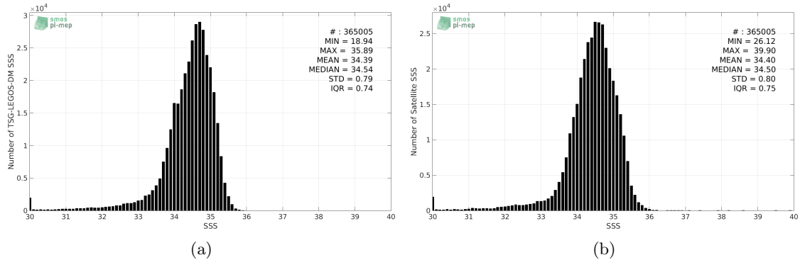
Figure 2: Histograms of SSS from TSG-LEGOS-DM (a) and SMOS-L3-CATDS-CECOS-LOCEAN-V3-9DAYS-25KM (b) considering all match-up pairs per bins of 0.1 over the North Pacific Ocean Pi-MEP region and for the full satellite product period.
