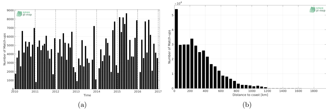
Figure 1: Number of match-ups between TSG-LEGOS-DM and SMOS-L3-CATDS-CECOS-LOCEAN-V3-9DAYS-25KM SSS as a function of time (a) and as function of the distance to coast (b) over the North Pacific Ocean Pi-MEP region and for the full satellite product period.
