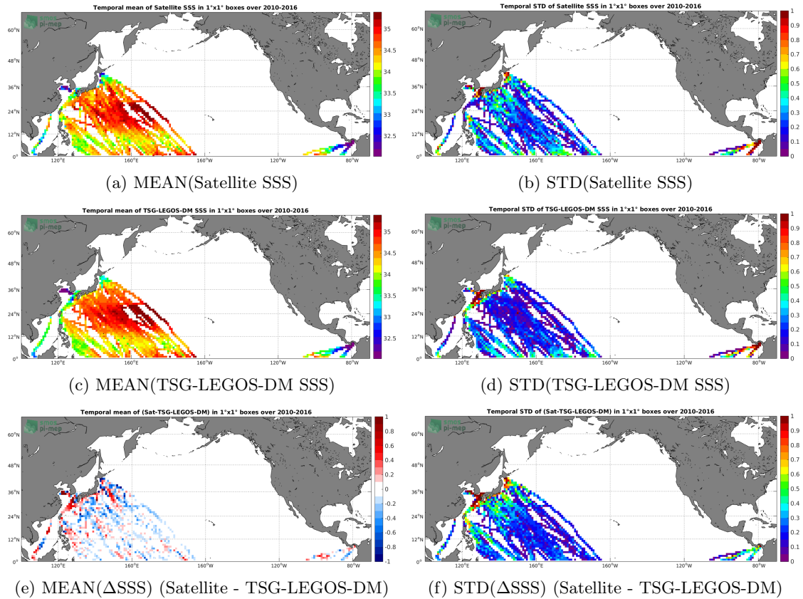
Figure 6: Temporal mean (left) and STD (right) of SSS from SMOS-L3-CATDS-CECOS-LOCEAN-V3-9DAYS-25KM (top), TSG-LEGOS-DM (middle), and of \Delta SSS (Satellite - TSG-LEGOS-DM). Only match-up pairs are used to generate these maps.
