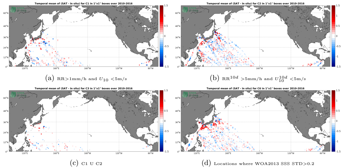
Figure 12: Temporal mean gridded over spatial boxes of size 1^\circ \times 1^\circ of \Delta SSS (SMOS-L3-CATDS-CECOS-LOCEAN-V3-9DAYS-25KM - TSG-LEGOS-DM) for 4 different subdatasets corresponding to: RR > 1\text{mm/h} and U_{10} < 5\text{m/s} (a), RR^{10d} > 5\text{mm/h} and U_{10}^{10d} < 5\text{m/s} (b), C1 U C2 (c), Locations where WOA2013 SSS STD > 0.2 (d).
